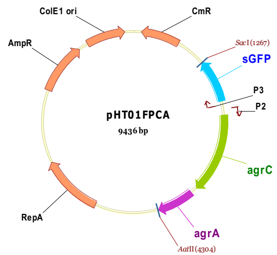
Figure 5| A. pHT01-based AIP generating system. B. AIP detecting system.
