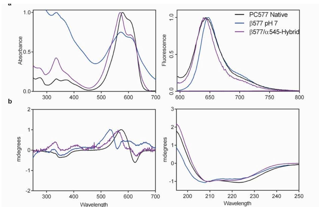
Figure 4. Characterisation data of \beta_{577}/\alpha_{545} closed form hybrid (purple line), \beta_{577} (blue line) and PC577 (black line). (a) UV-Vis absorbance (left) and Fluorescence (right) (b) Circular Dichroism of chromophore region (left) and folding region (right).
