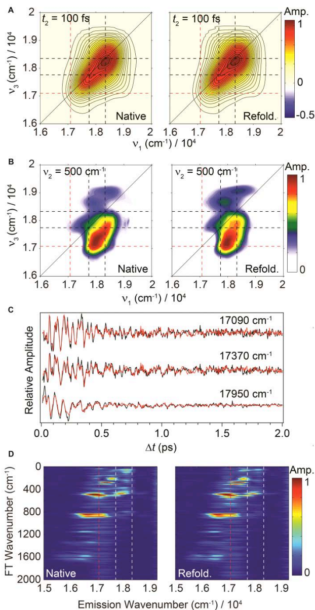
Figure 2. Coherent spectroscopy of the light-harvesting PE545 protein. A) Normalized 2D spectra at t_2 = 100 fs. B) 2D coherence maps at 500 \text{ cm}^{-1} for native (left) and refolded (right) proteins. C) Broadband transient absorption (BBTA) traces of native (black) and refolded (red) proteins at various spectral positions, where each trace is an average of five repeats. D) The power spectra for native (left) and refolded (right) proteins generated from coherent BBTA. Dashed lines indicate steady-state absorption (white) and fluorescence (red) maxima.
