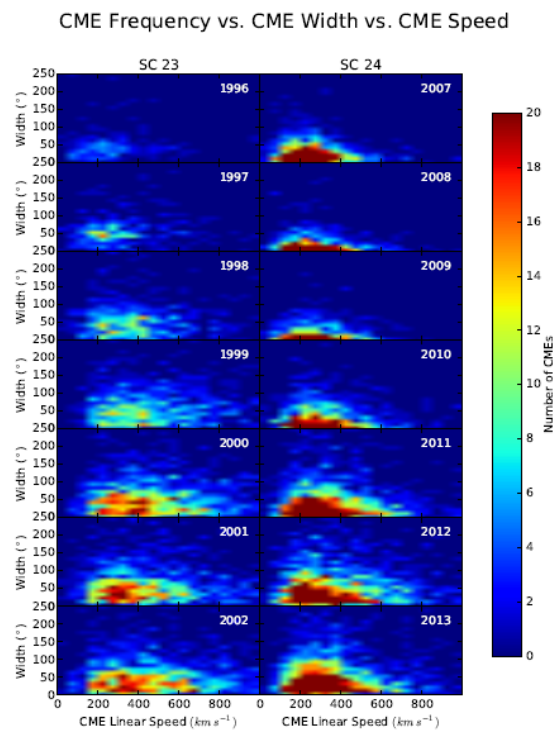
Figure 6: 2D histograms of CME frequency as a function of angular width and speed. The first column is approximately the first 7 years of SC (Solar Cycle) 23; the second column is the corresponding 7 years of SC24. Each row represents 2 distributions from identical phases in different solar cycles. For example, 1996 and 2007 are in the same row and are solar minimum years for SC23 and SC24, respectively. The histograms are presented on the same color scale so that the disparity in CME frequency for identical phases is apparent. Solar cycle dependence of CME frequency and speed is also clear when examining a single column {the histogram structures widen along the speed axis and become more intense (redder) as one proceeds from solar minimum to solar maximum. There are far more CMEs recorded in SC24 with widths <50^\circ , as well.
