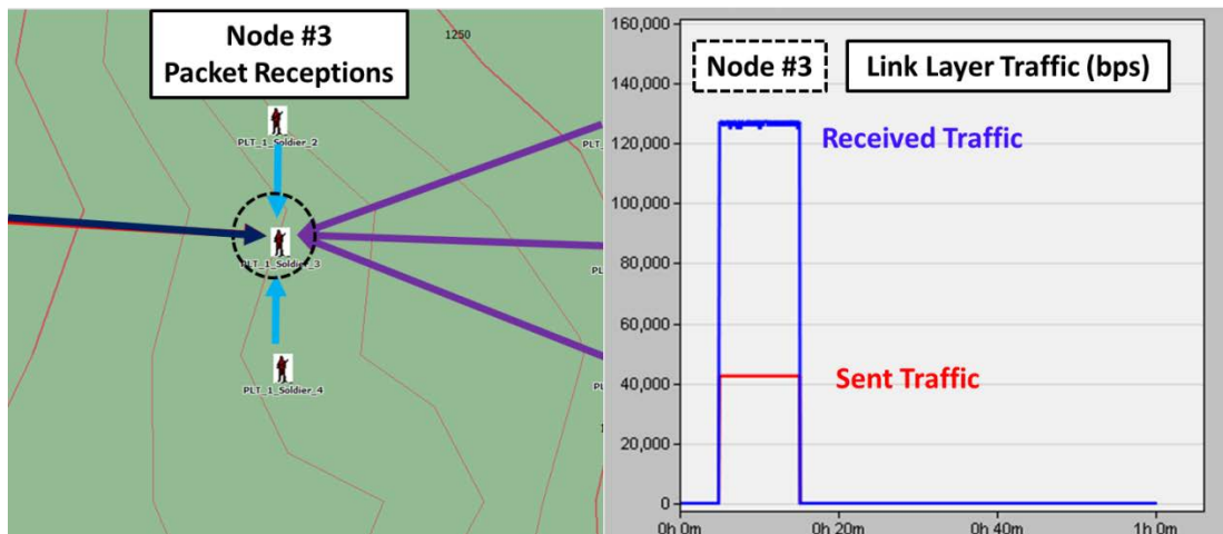
Figure 2-20. Voice Traffic Sent and Received by Node #3
