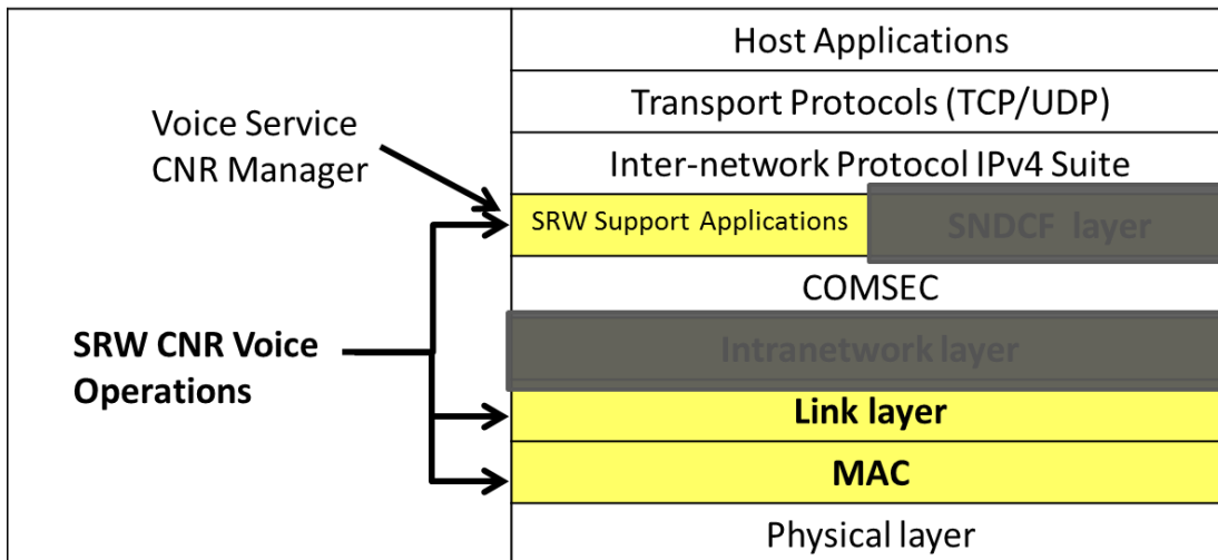
Figure 2-14. CNR Operations within the SRW Protocol Stack
