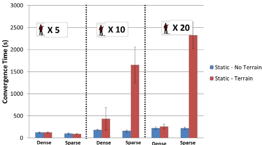
Figure 2-13. Convergence Times
