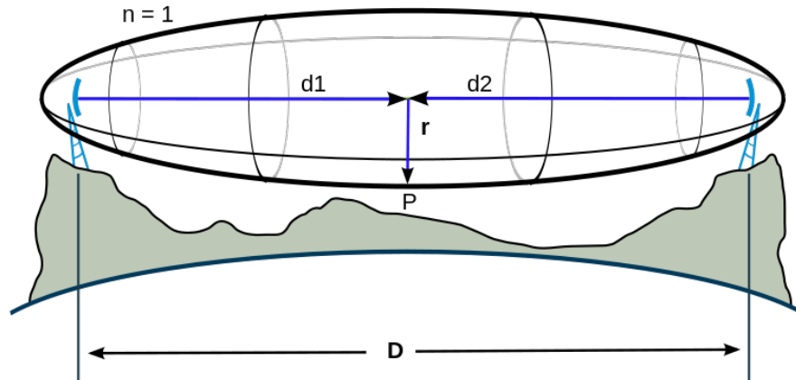
Figure 3-3. Fresnel Zone [12]
