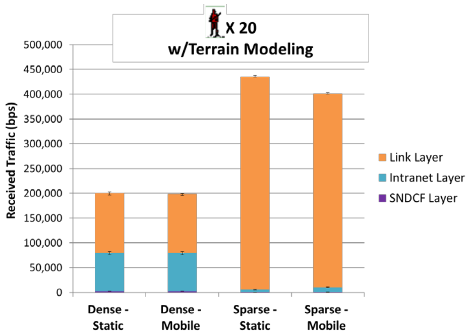
Figure 2-11. Overhead Traffic Broken Down by Link, Intranet, SNDCF Layer
