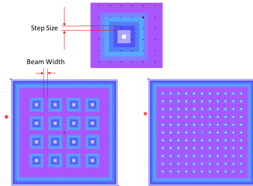
Figure 21. Potential layouts for 6 step hybrid grayscale patterns which accommodate a 1\ \mu\text{m} beam diameter with two different step sizes. The lower left image represents the spacing requirements for a low resolution patterning where a 400nm step size is required while the lower right shows the spacing for an 80nm step size.
