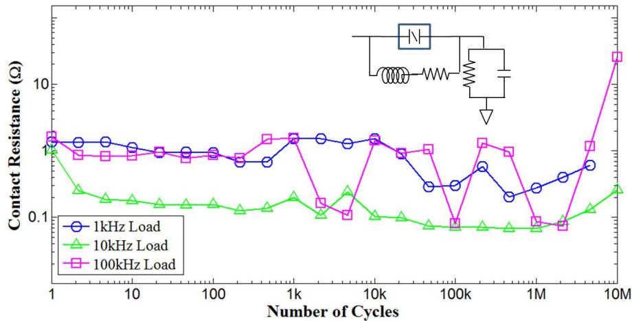
Figure 61. Comparison of contact resistance vs. device life of Au-Au 8\mu\text{m} radius micro-contacts for the test circuit shown. The inductance used was 100\ \mu\text{H} along with a 5\ \text{M}\Omega parallel resistance, as well as an RC circuit in series, using a 1\ \Omega series resistance, and 0.6\ \text{pF} of capacitance). The tests were conducted at the three frequencies listed, two of which were still operational at the 10 million cycle target and one which failed to close just prior to reaching 10 million cycles [164].
