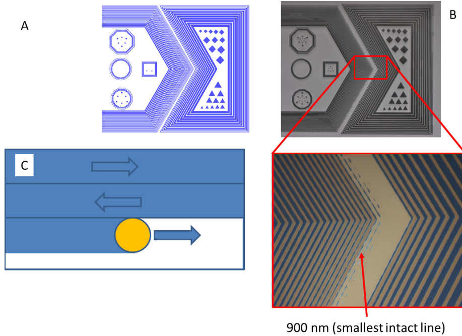
Figure 43. Conceptual illustration of lithographic printing from a CAD-based file (A), resulting in fully exposed or unexposed areas (B). To accomplish this, the beam used to print is swept horizontally along precalculated lines, and beam is activated and deactivated to expose only the geometric shapes provided..
