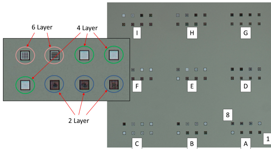
Figure 44. Test matrix of nine variations of power and duty cycle applied to identical eight pattern design for evaluation of optimal settings for two, four, and six layer designs.
