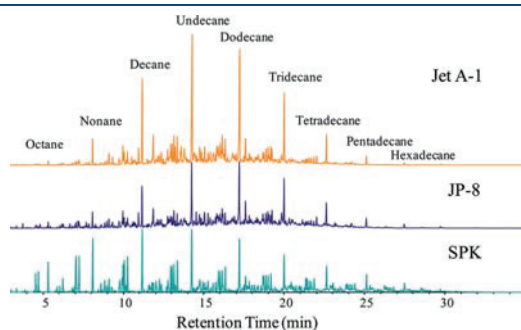
Figure 2. Gas chromatograms of fuels.
