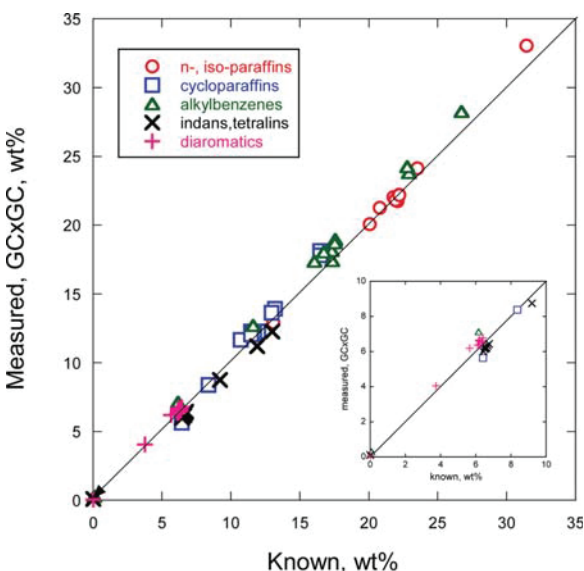
Figure 3. GC × GC results for 92 different chemical components blended into 12 different mixtures reflecting jet fuel ranges of hydrocarbon group types.
