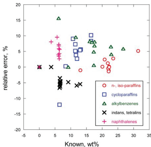
Figure 4. Relative error versus known compound class for the 12 model mixtures examined using GC × GC.
