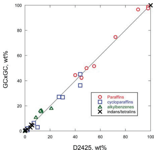
Figure 10. Comparison of alternative fuel hydrocarbon type results by two techniques, D2425 and GC × GC, for these alternative fuel sources: FT SPK, Camelina HEFA-SPK, tallow HEFA-SPK, algal oil product, ATJ fuel process, and mixed fat conversion process.
