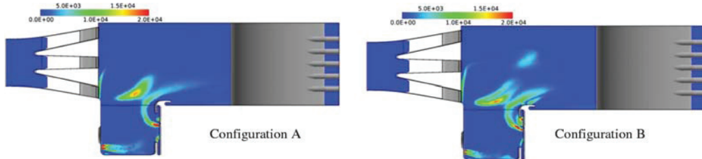
Fig. 12 Product formation rate \rho S_C contours at centerplane. The units are in kilograms per cubic meter per second. The product formation rate is the same progress variable source term.
