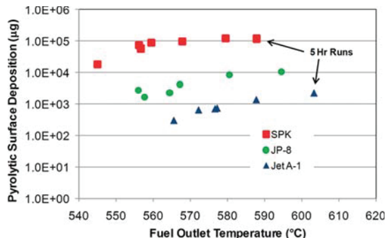
Figure 14. Comparison of total pyrolytic deposition as a function of fuel type and bulk outlet temperature.
