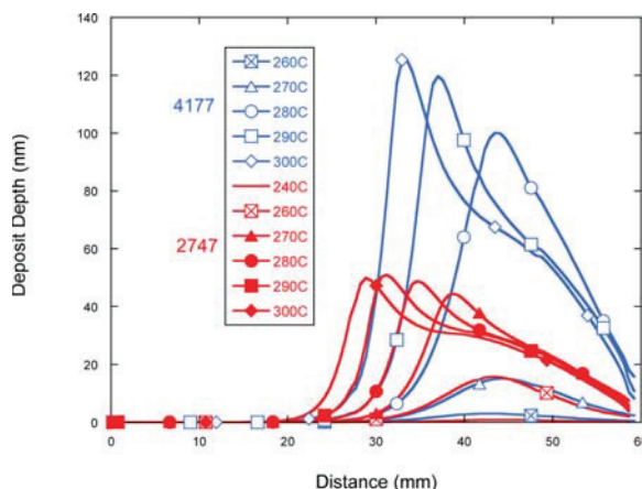
Figure 13. Plots of CFD with chemistry calculated deposit depths vs distance for two fuels at various JFTOT set point temperatures. The markers are not actual data points; they are used to identify the curves only.
