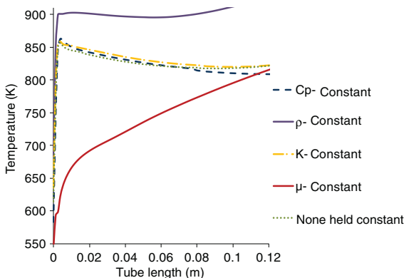
Fig. 10 Simulated interior surface temperatures with one supercritical phase property held constant (value determined at 780 K) while the other properties vary with temperature.
