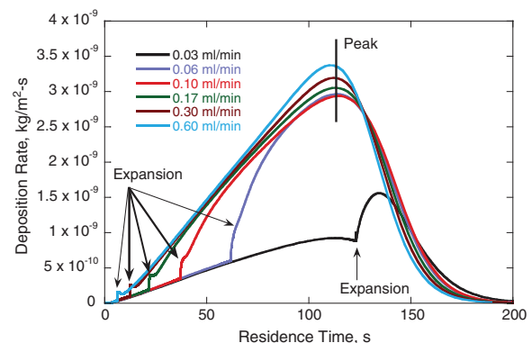
Fig. 7 Simulated deposition rate variation with residence time for F3084 fuel flowing into an abrupt expansion.
