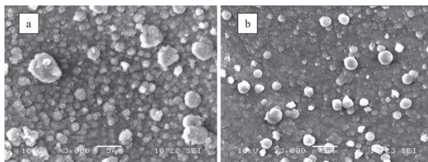
Figure 16. SEM micrographs of oxidative deposit formed during thermal stressing of JP-8: (a) T_{\text{out}} = 566\text{ }^{\circ}\text{C} , X_{\text{L-G}} = 11.3\% ; (b) T_{\text{out}} = 574\text{ }^{\circ}\text{C} , X_{\text{L-G}} = 15.7\% .
