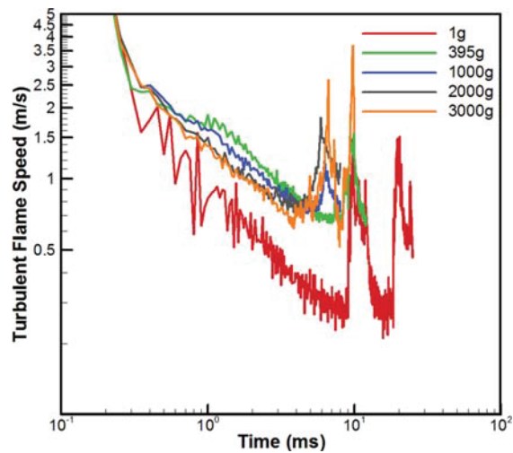
Fig. 8 Turbulent flame speed as a function of time for propane-air premixed flames presented in Fig. 6
