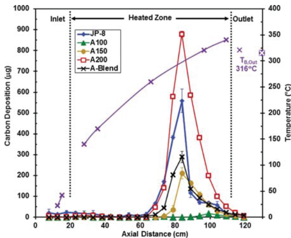
Figure 10. Carbon deposition and measured wall temperature profiles from flow reactor testing with a varying aromatic solvent type in Sasol SPK at 10%v.
