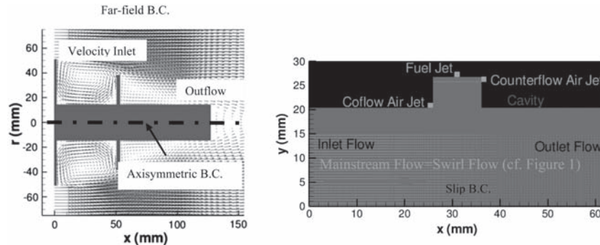
Fig. 2 Computational domains for the axisymmetric cavity (left) and the planar cavity (right). The sample axisymmetric cavity corresponds to the case in which the afterbody disk is placed at x/D_o = 0.5 . The whole computational domain is not shown here. The planar cavity indicates the location of the injections in its normal configuration. The boundary conditions are also indicated. The air mainstream flow direction is also indicated for the small planar cavity case. Note that the air mainstream flow corresponds to the swirl flow in Fig. 1.
