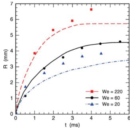
Figure 3. Temporal evolution of the maximum wetting radius (or contact line position) ( R ) on an isothermal dry surface at T_s = 180^\circ\text{C} with characteristic Weber numbers of We = 220, 60, and 20 . The initial droplet radius is R_0 = 1.5 mm, and the Weber numbers correspond to impact velocities of V_0 = 2.34, 1.21, and 0.7 m/s, respectively. The experimental results (filled-symbol data) are from Bernardin et al. 18 and the lines are our numerical predictions. The accommodation coefficient used in the Schrage model is \varepsilon = 0.03 .
