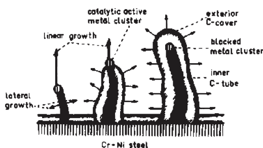
Figure 1. Comparison of linear and lateral growth mechanisms of carbon filaments. 13
