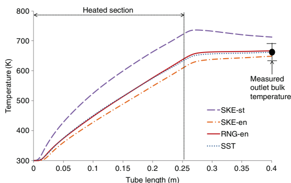
Fig. 3 Calculated bulk fuel temperatures along the length of the long tube using different turbulence models.
