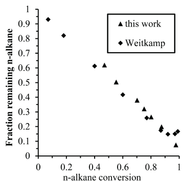
Figure 3. Residual normal alkane fraction in the fed C_n effluent mixture as a function of conversion for n-C_{14} (this work, -0.5\% Pt/US-Y zeolite) and n-C_{15} (Weitkamp, -0.5\% Pt/CaY zeolite) as a function of conversion.
