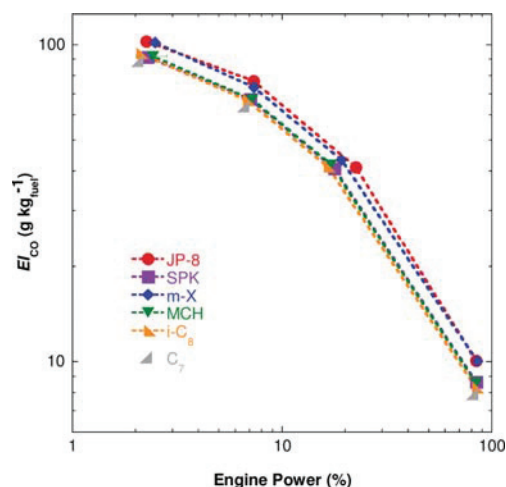
Figure 2. Emission indices for CO as a function of engine power and fuel.
