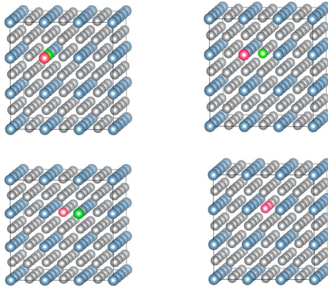
Fig. 8: A 3x3x4 supercell of \text{Ni}_3\text{Al} showing Co (red) and Ti (green) atoms at Al-Al, A-Ni, Ni-Ni and Ni-Al sites.
