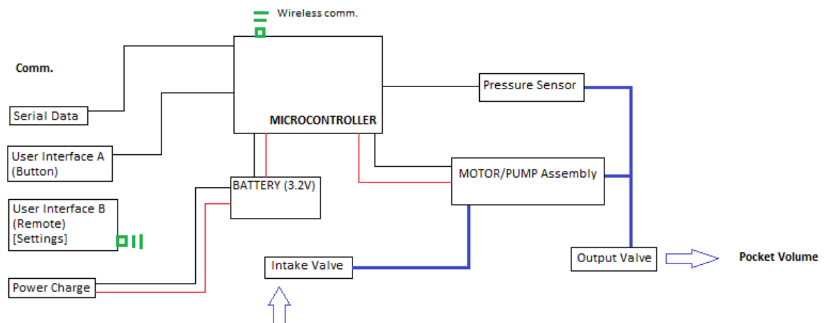
Figure 16: Design Schematic Diagram
