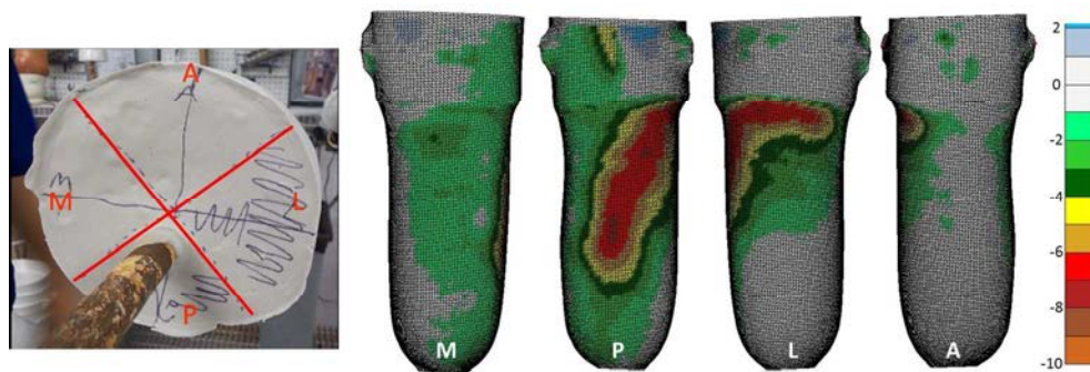
Quadrant system and exemplar mold rectification map for NU-FlexSIV Socket. M: medial; P: posterior; L: lateral; A: anterior. Color coding on the rectification map indicates depth of plaster removed.
