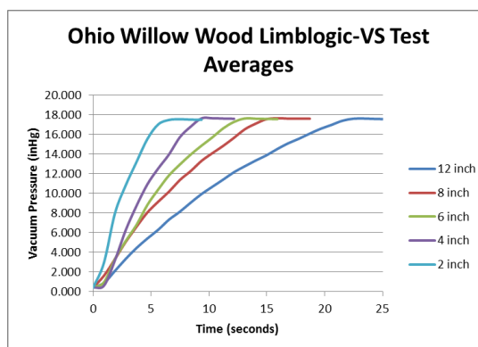
Plot 2 – Ohio Willow Wood Test Data: Evacuating volumes
