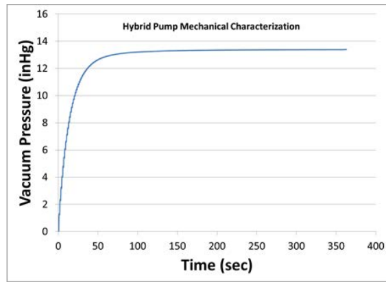
Figure 8 Mechanical test set up (left) and results for 6.46 in 3 canister (right).
