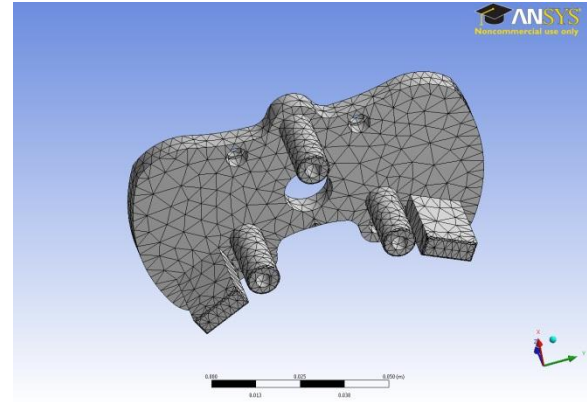
Simulation Figure B – Top view of Top Plate Mesh
