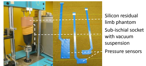
Figure 2: Experimental setup to validate FE model. (Left) Loads are applied to a silicon limb model in a custom made socket. (Right) Sensors are inserted between the liner and socket to estimate the normal stress (interface pressure).
