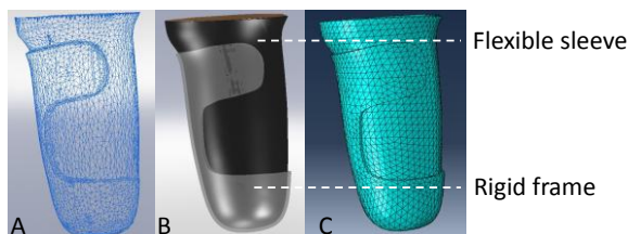
Figure 1: Anterior view of a sub-ischial socket modeled as a simplified two-layered system. A) Scanned 3D vertex data of the socket. B) Solid geometric model. C) FE model is discretized using tetrahedral elements.
