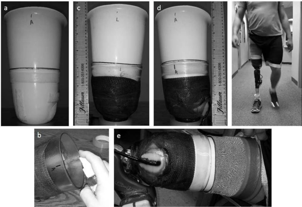
Flexible check socket fabrication: (a) flexible inner socket with Velcro and sealing ring to hold rigid PETG (polyethylene terephthalate) outer socket in place (distal port hole for air not shown); (b) outer socket sprayed with alcohol to allow it to be pushed onto inner socket; (c) lateral and (d) anterior view of flexible inner socket inserted into outer socket and reinforced with fiberglass tape, black line indicates top of rigid socket; (e) donned socket showing attachment of barb to distal end of outer socket (vacuum is drawn from between liner and inner socket through port hole and between inner and outer socket via barb); and (f) mid-stance of gait with flexible check socket.
