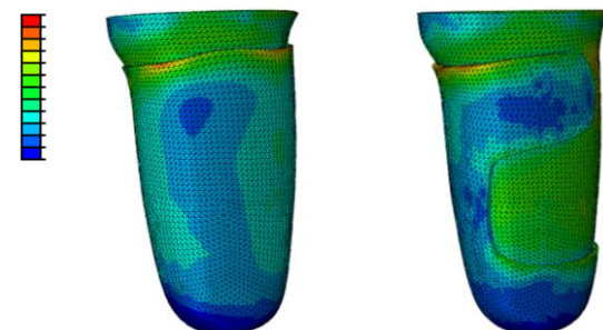
Figure 3: Anterior view of FE analysis stress results: (Left) Totally rigid frame (i.e. no cut-outs) and (Right) a ladle shaped frame with medial strut.
