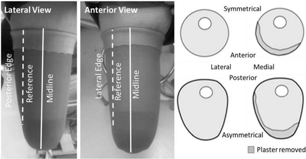
Example of a symmetrical residual limb shape wherein the area of the residual limb bounded by the reference line and posterior or lateral edges of the limb are approximately the same: this area represents the material to be removed during rectification of the positive model. Cross-sectional diagrams show the plaster removed based on whether the residual limb is considered symmetrical or asymmetrical.
