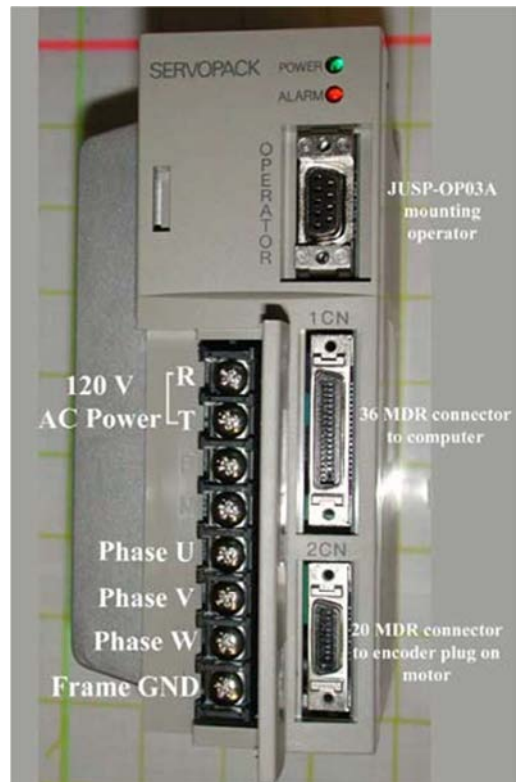
Figure 20: The Yaskawa SGD-02BS Servopack.
