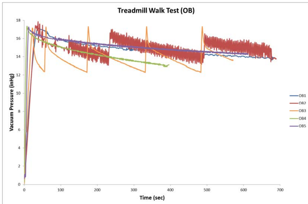
Figure 13: Vacuum pressure over time recorded during treadmill testing using the e-Pulse
