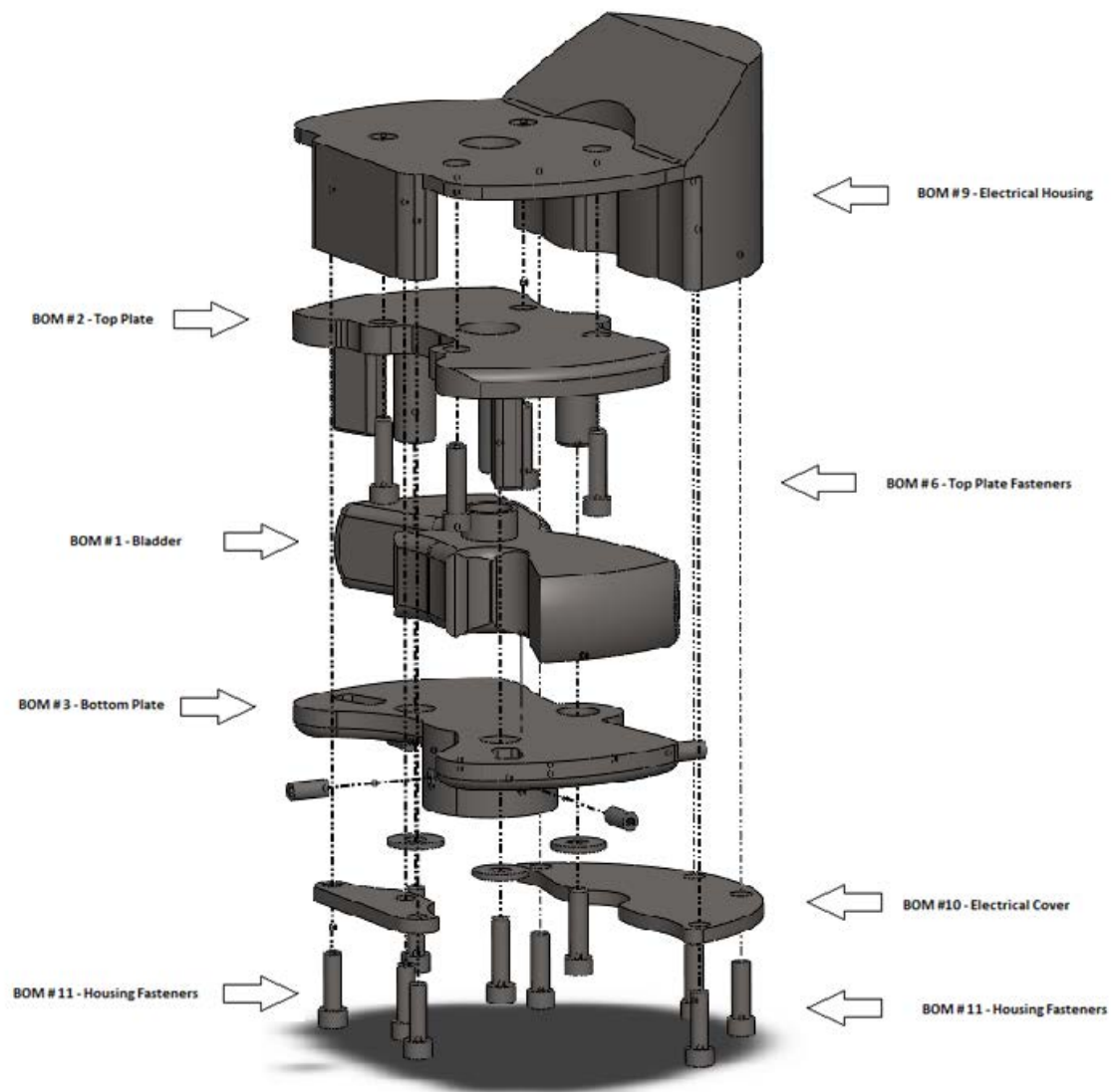
Figure 12: Exploded View of Prototype Assembly
