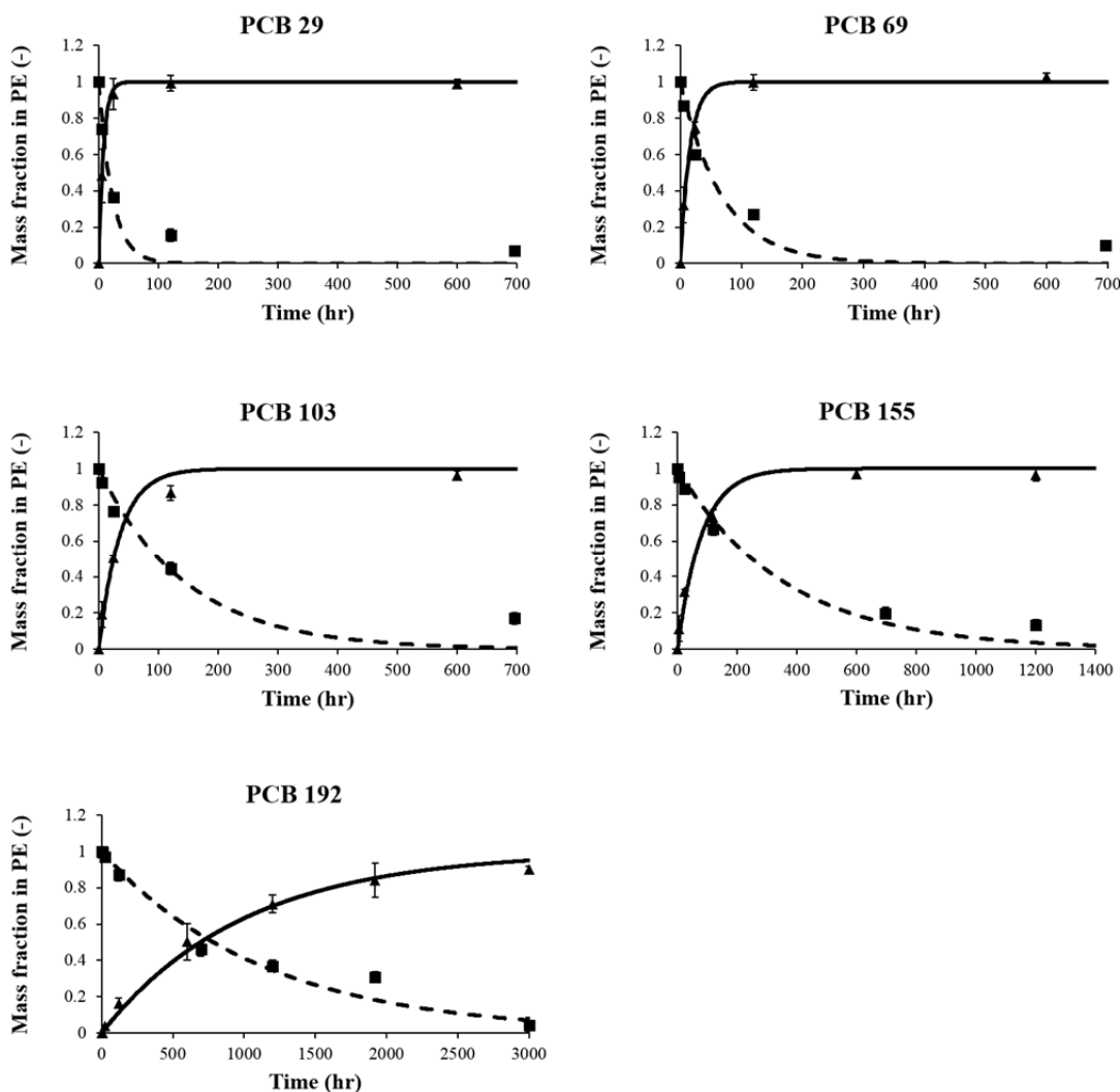
Figure 11. Uptake and release kinetics of five PCB congeners for PE in water. The triangles and squares are experimental results for uptake and release kinetics, respectively. The solid and dashed lines are fitted data using first-order model for uptake and release kinetics, respectively. Note the different scales in x-axis for different PCB congeners.
