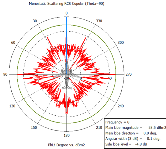
(a) The RCS of B-737 400
