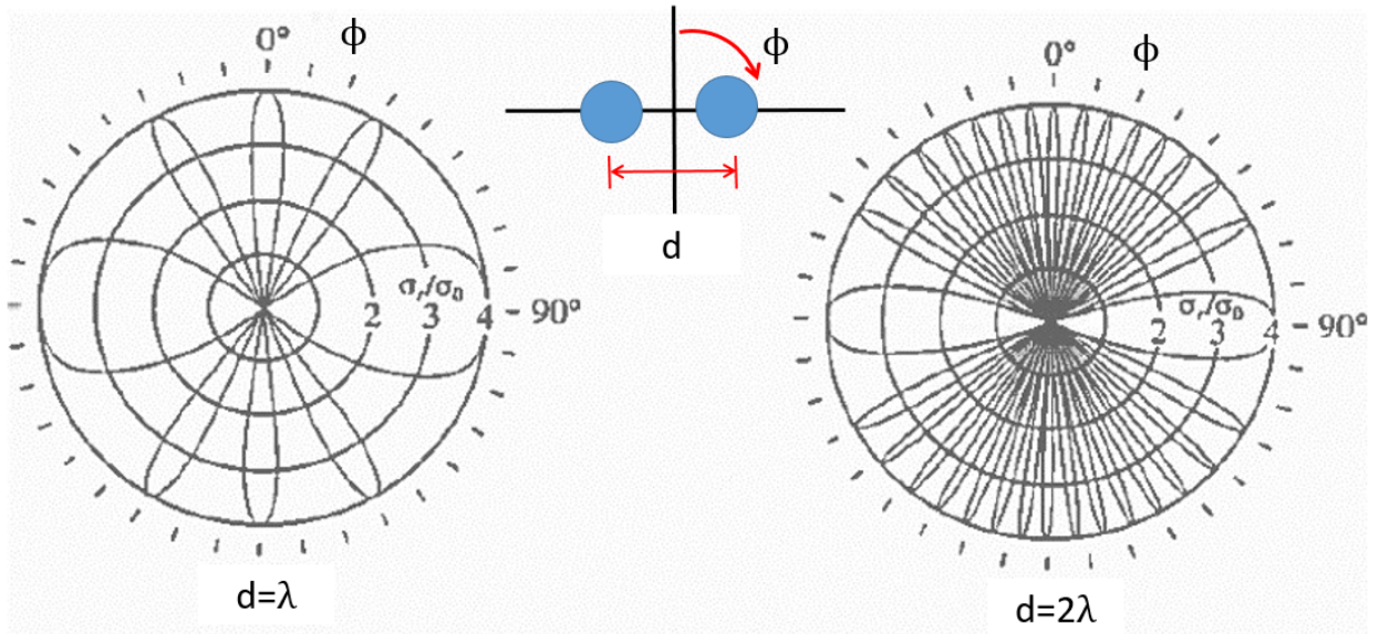
Figure 2.22. The RCS measure of two sphere objects are set apart by \lambda (left) and 2\lambda (right), in azimuth angle 0^\circ \leq \phi \leq 360^\circ . Adapted from: [40]
