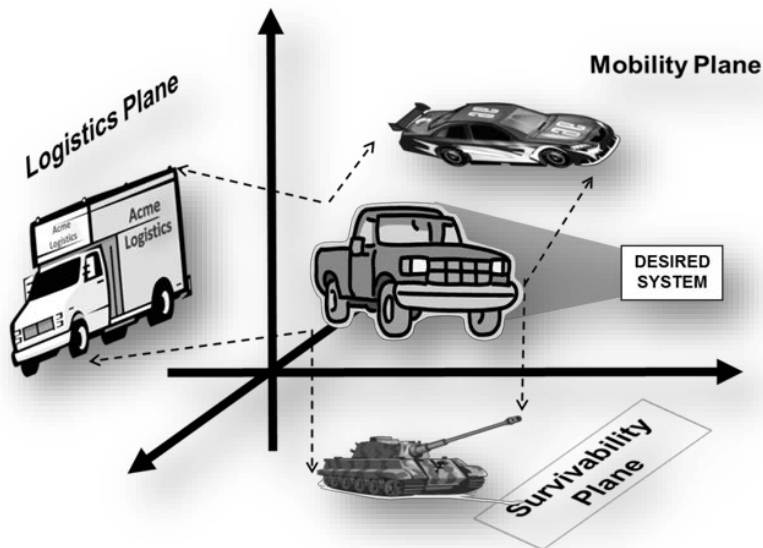
Figure A2. An example of a projection from 3-D to 2-D space. An abstract example of projections from a higher space to three lower spaces. This issue is what truck properties (from the real 3-D) space are identically projected to the three subspaces. Knowledge of the sharing or exclusivity of this can impact performance and, ultimately, platform effectiveness.
