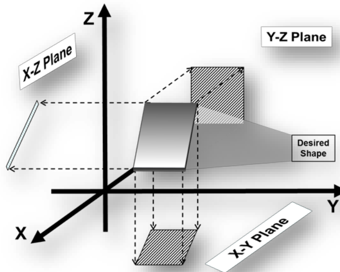
Figure A1. Projections in spaces of differing dimensions. An opaque physical object is located in three-dimensional space. If a light is projected from right to left, parallel to the Y axis, a shadow is cast on the X-Z plane. Likewise, if a light is projected directly downward, parallel to the Z axis, a shadow will be cast on the X-Y plane. So also a light beam projected along the X axis casts another shadow on the Y-Z plane. In this case, the three projections are different, but each provides valid, but incomplete, information concerning the 3-D object.
