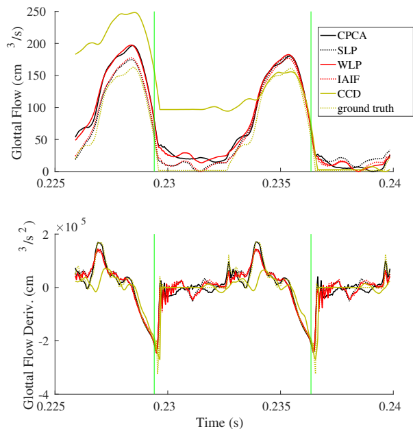
Figure 8. Glottal flow and derivative ( \dot{\bar{e}}_c[n] ) estimates generated by the tested algorithms at the median cycle marked in Fig. 7. The endpoints of the cycle are marked with vertical green lines.
