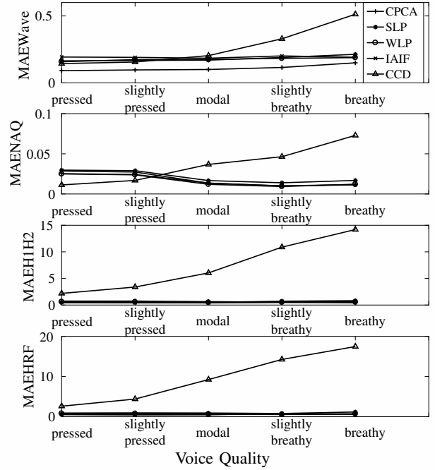
Figure 4. Subset error averages for voice qualities. Only utterances of vowel /ä/ in the sustained-vowel data set are used.
