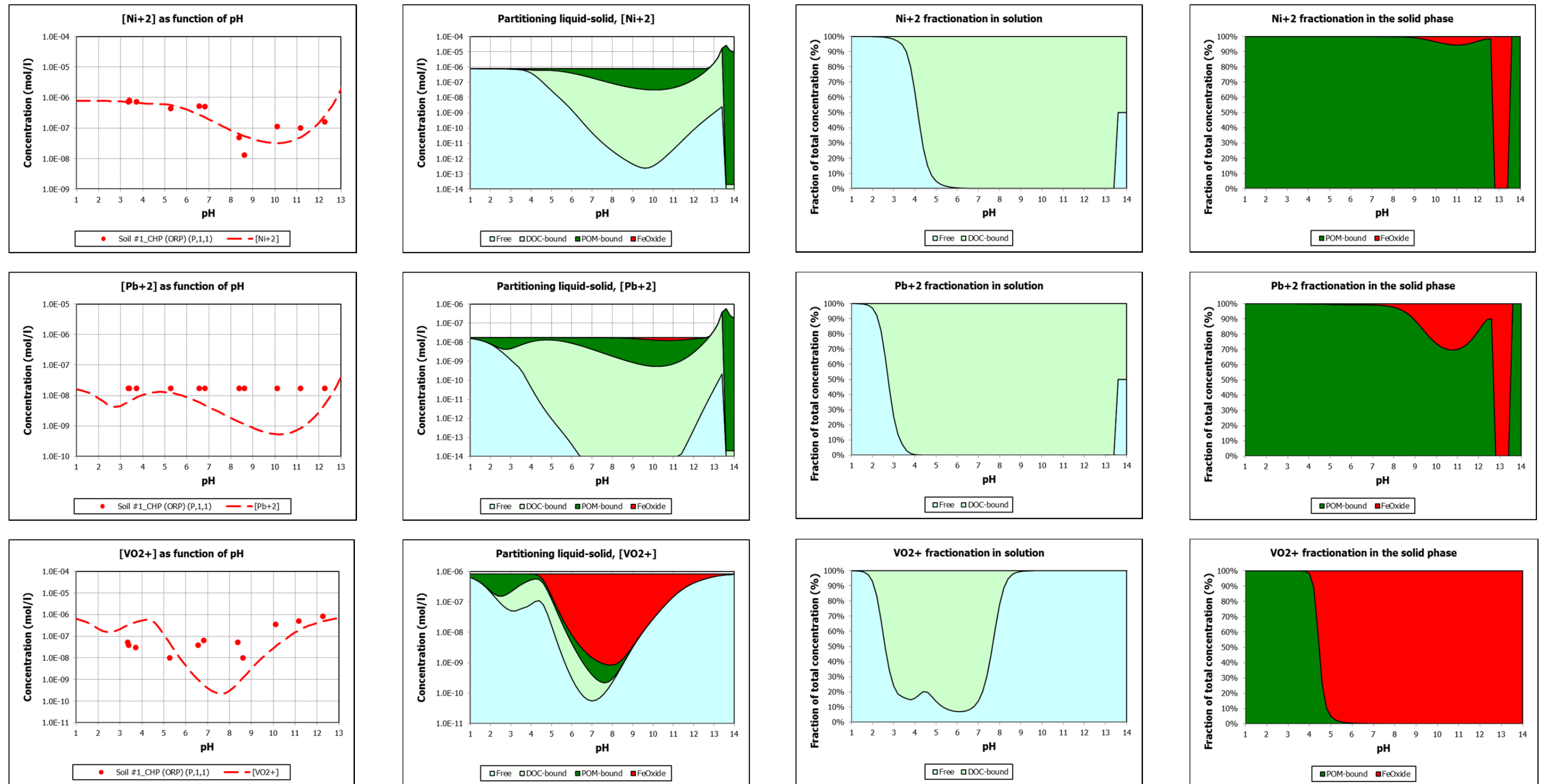
Figure 4.2.15 (cont.) Geotechnical Modeling: Metal release and partitioning in the presence of CHP in Soil #1. The first graph in each row depicts the solubility of a given metal (symbols and line represent experimental data and model prediction, respectively) The subsequent graphs in the row show the liquid-solid partitioning and the solution and solid phase fractionation of the same metal.
