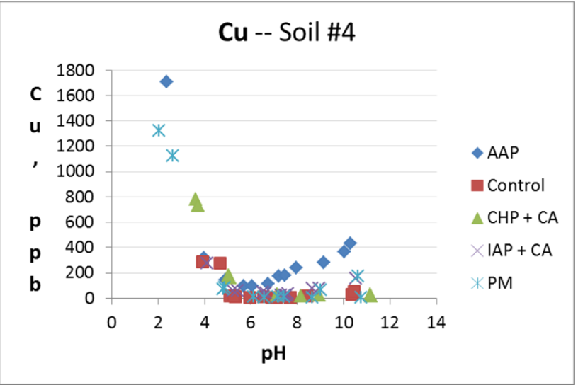
Figure 4.2.11 Detailed pH Evaluation: pH-dependent leaching of metals from Soil #4 Note: (AAP = alkaline-activated persulfate; CHP = iron-catalyzed hydrogen peroxide; CA = citric acid chelating agent; IAP = iron-activated persulfate; PM = permanganate)
