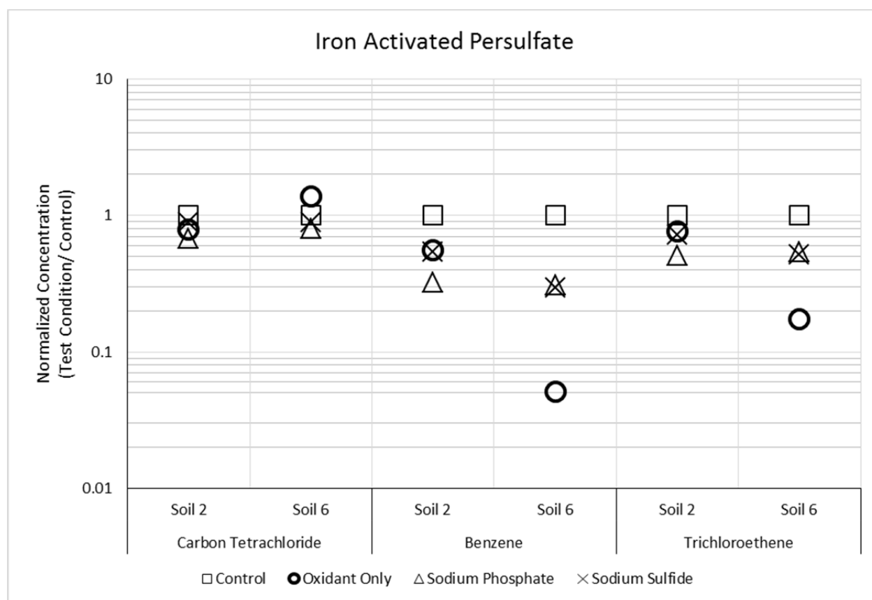
Figure 4.4.10 Pretreatment Stabilization of IAP System: Treatment Efficacy- Normalized Concentrations of probe compounds carbon tetrachloride, benzene, and trichloroethene.
