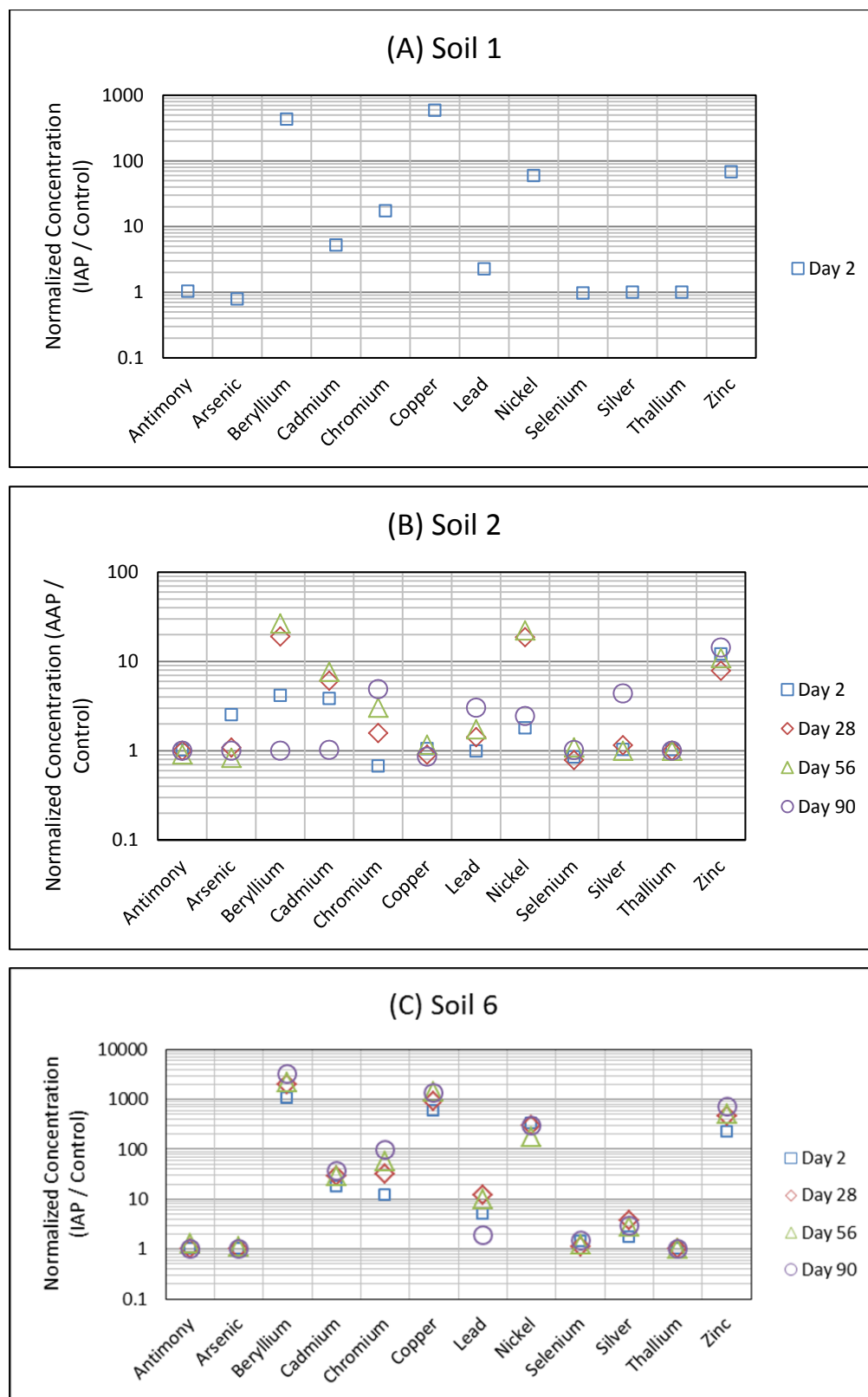
Figure 4.4.6 Pretreatment Stabilization: Normalized concentration of metals for reactors with IAP applied versus control conditions (no IAP treatment).
