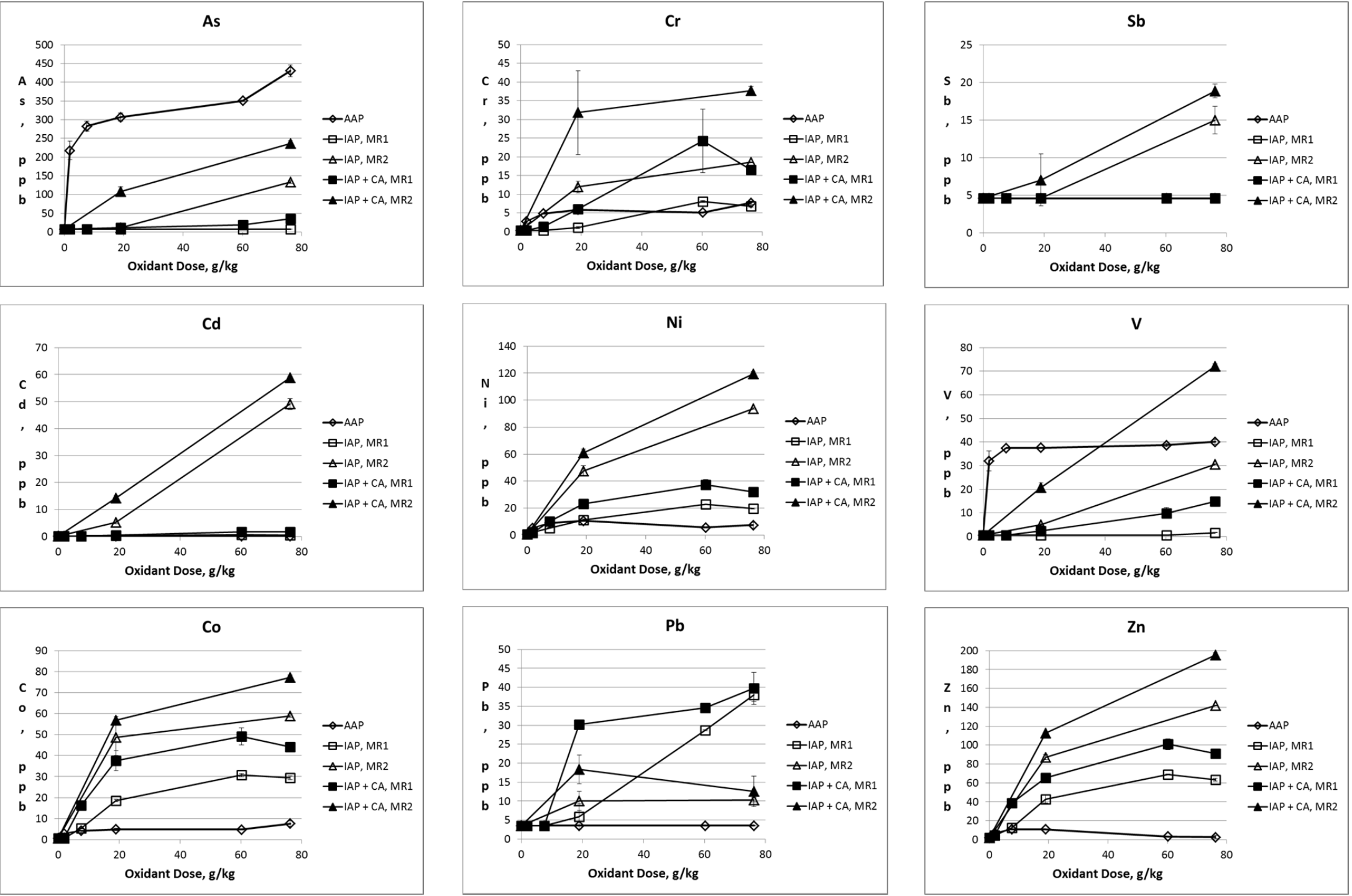
Figure 4.2.7 Initial Screening: Metals mobilization as a function of persulfate dose for soil#1
