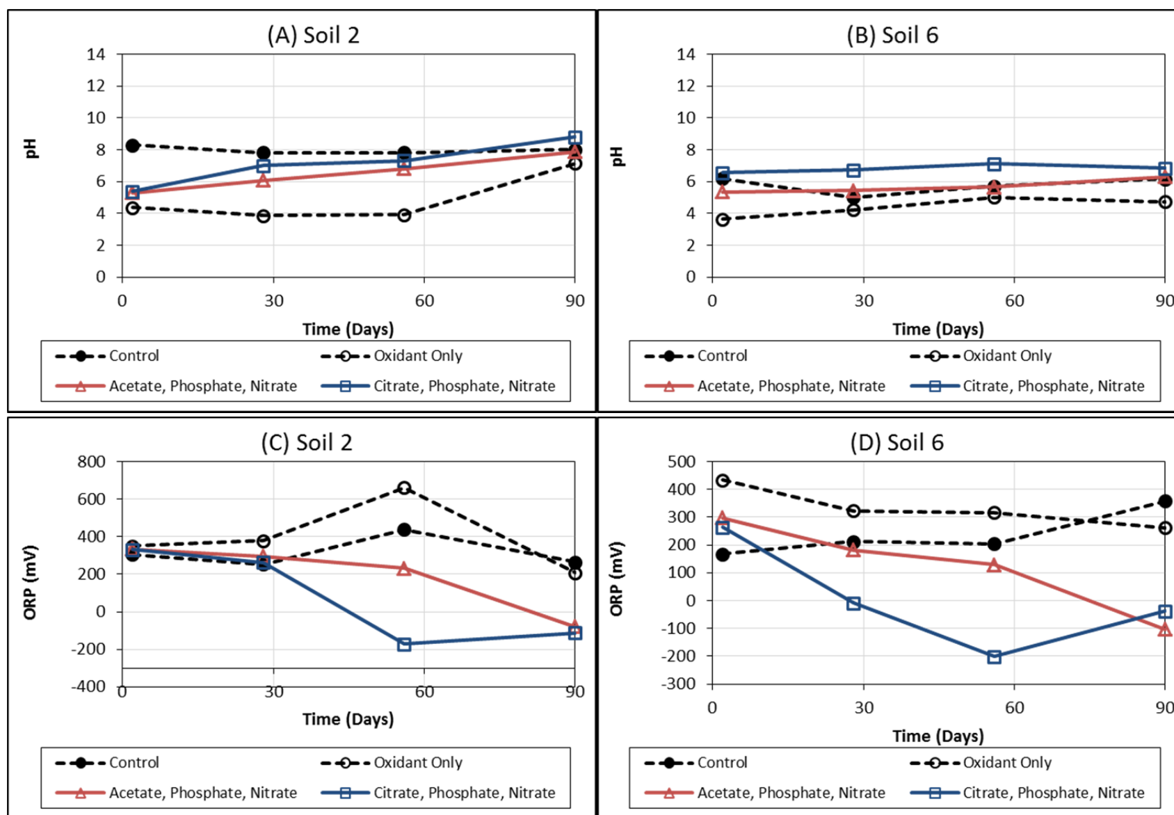
Figure 4.4.30 Co-Treatment Biological Stabilization of CHP System: Geochemical parameters at 2, 28, 56, and 90 days
