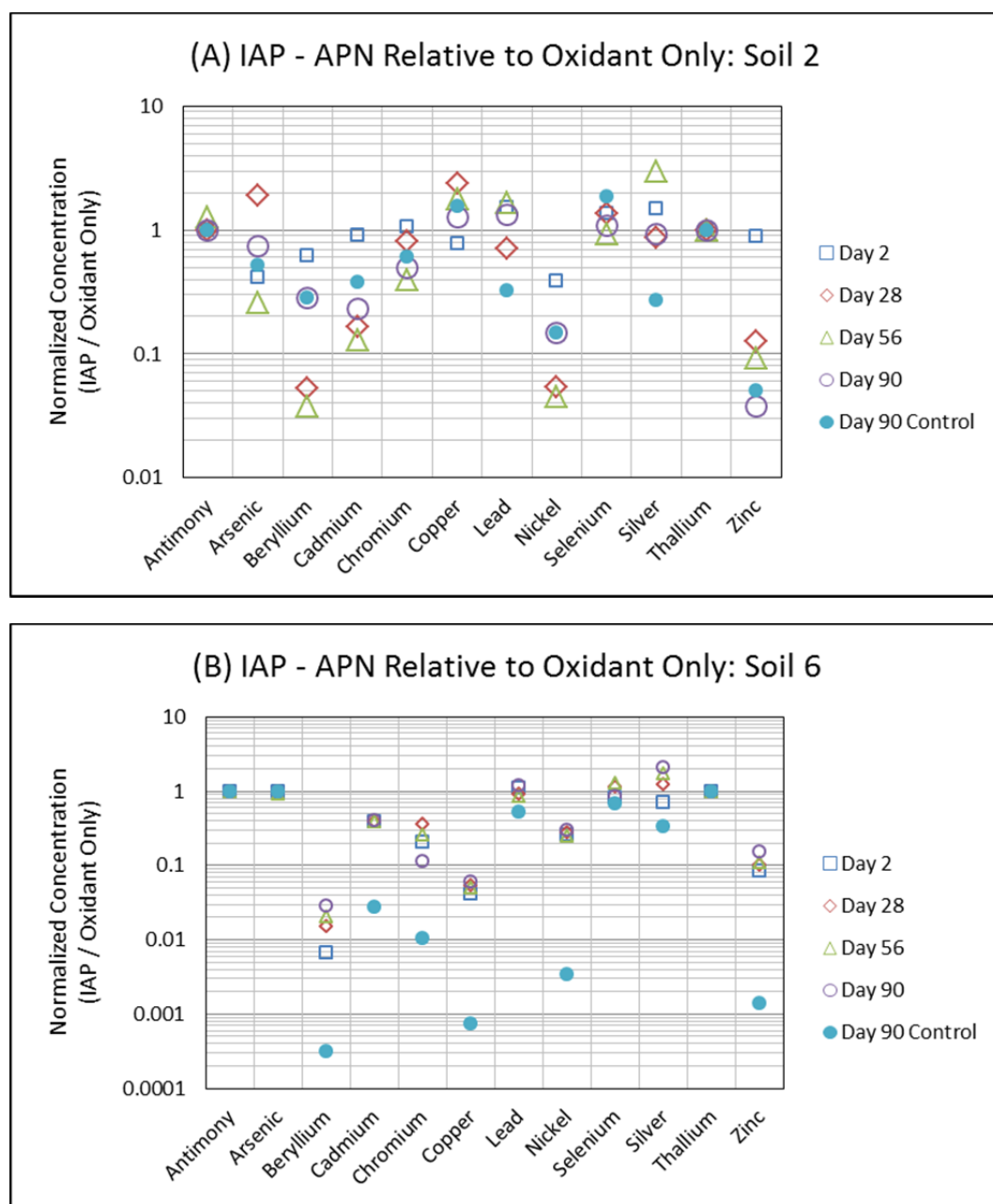
Figure 4.4.26 Co-Treatment Biological Stabilization of IAP System: Select normalized metal concentrations at 2, 28, 56, and 90 days
