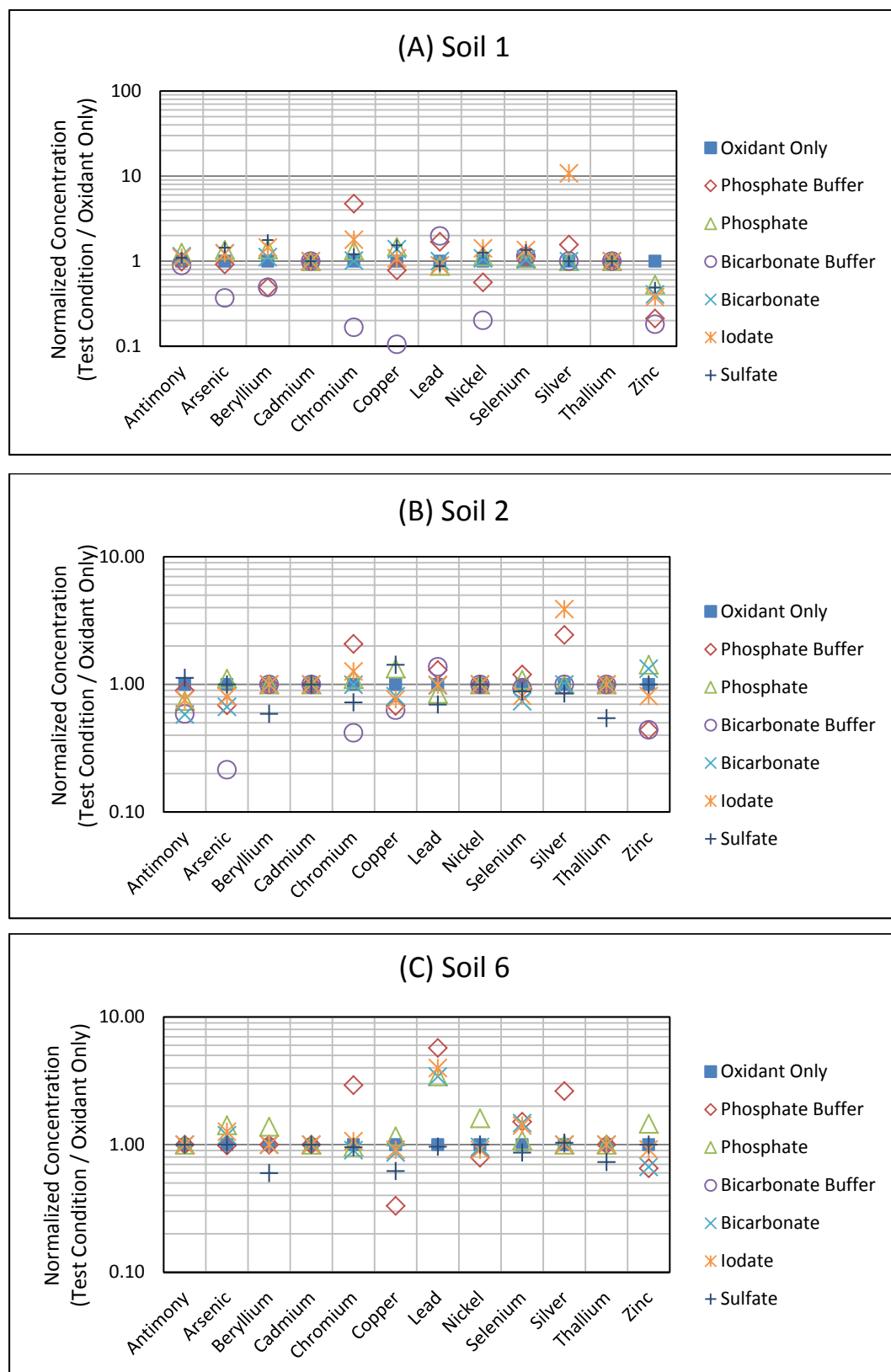
Figure 4.4.39 Co-Treatment Chemical Stabilization of AAP System: Select normalized metal concentrations for 6 chemical treatment options.
