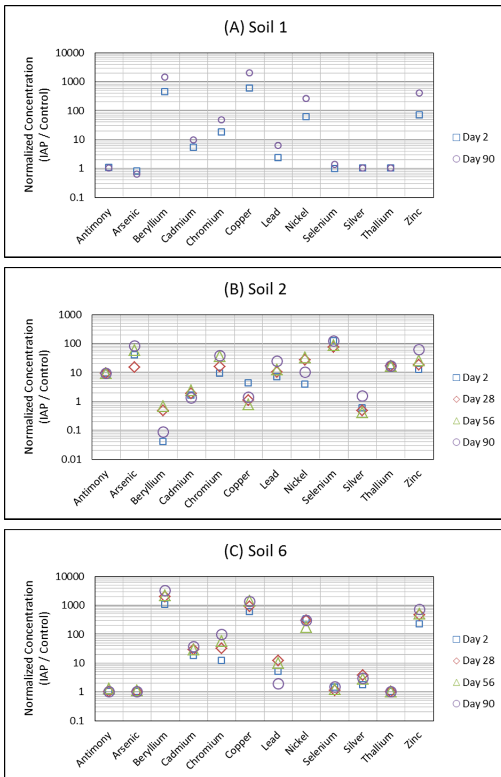
Figure 4.4.23 Co-Treatment Biological Stabilization: Normalized concentration of metals for reactors with IAP applied versus control conditions (no IAP treatment).
