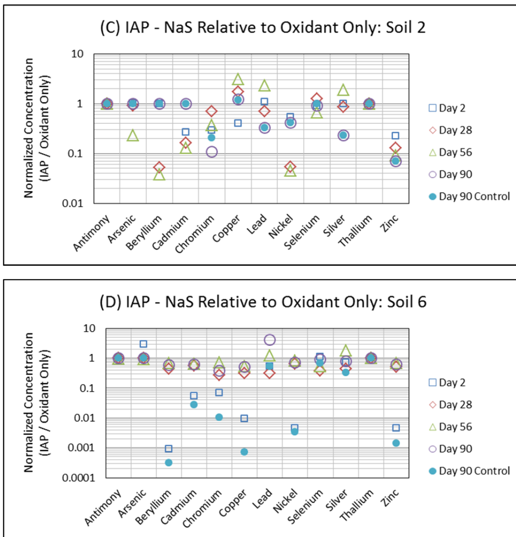
Figure 4.4.9 (cont.) Pretreatment Stabilization of IAP System: Select normalized metal concentrations at 2, 28, 56, and 90 days
