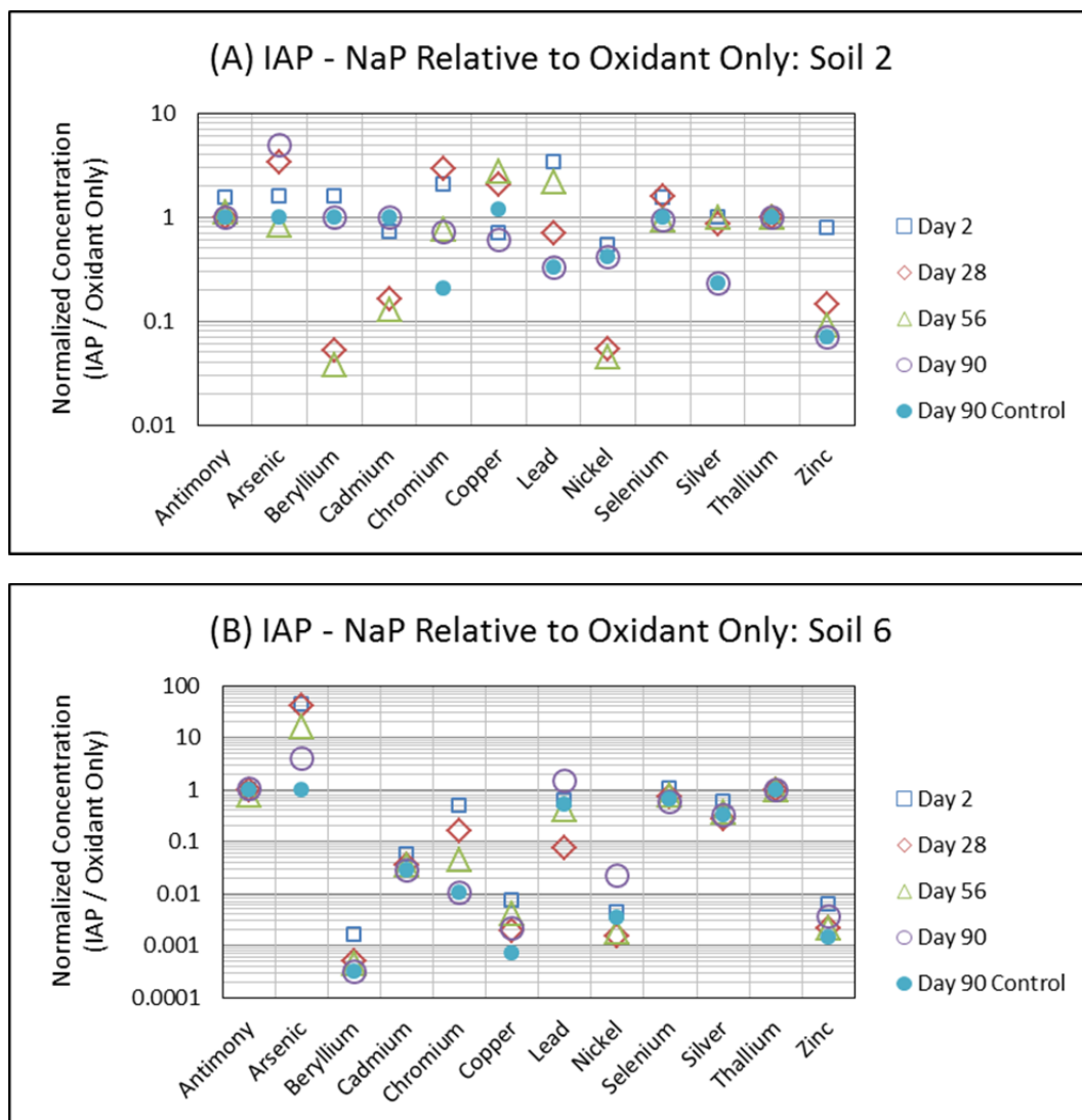
Figure 4.4.9 Pretreatment Stabilization of IAP System: Select normalized metal concentrations at 2, 28, 56, and 90 days
