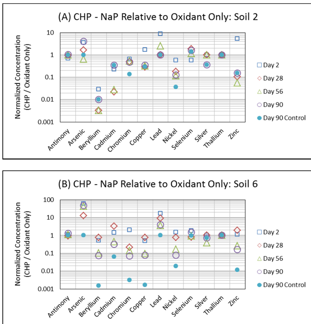
Figure 4.4.14 Pretreatment Stabilization of CHP System: Select normalized metal concentrations at 2, 28, 56, and 90 days
