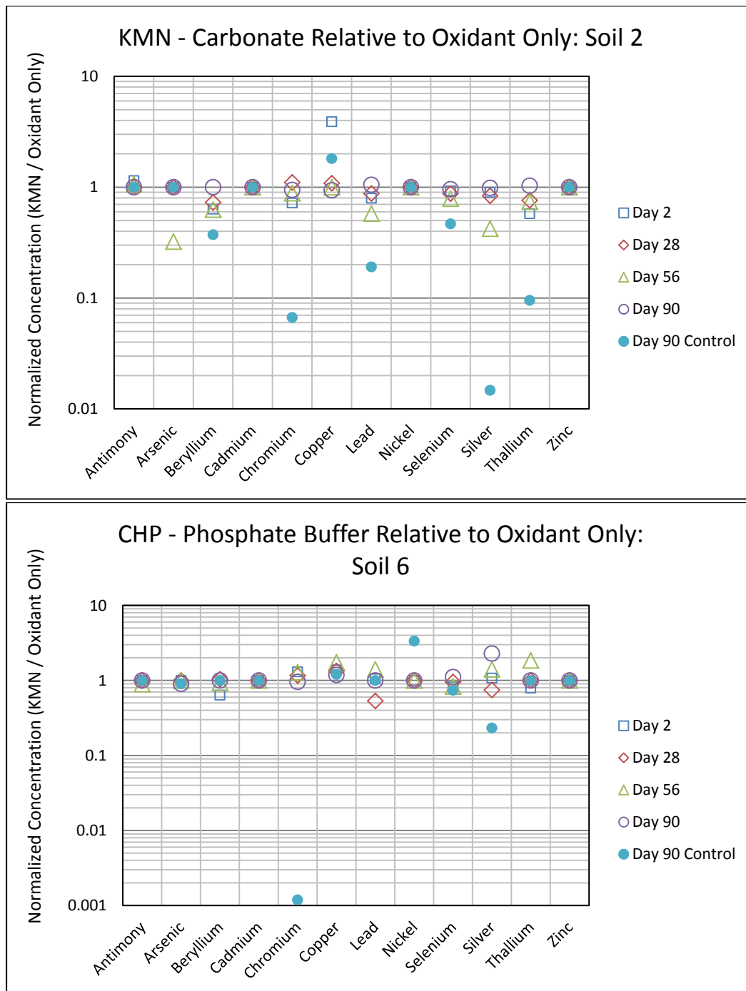
Figure 4.4.53 Co-Treatment Chemical Stabilization of PM System: Select normalized metal concentrations at 2, 28, 56, and 90 days
