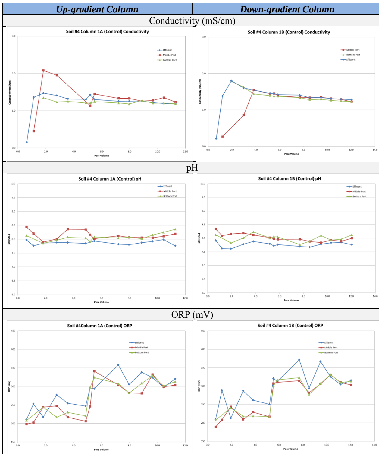
Figure 4.3.7 Column Experiment: Soil #4 with Control Treatment (groundwater only) – Geochemical variation with increasing groundwater PV.
