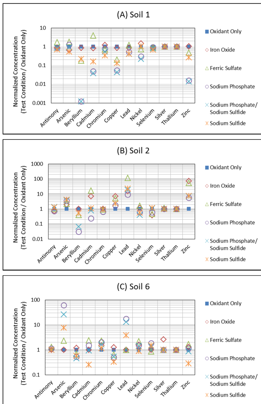
Figure 4.4.12 Pretreatment Stabilization of CHP System: Select normalized metal concentrations for 5 Pretreatment options.
