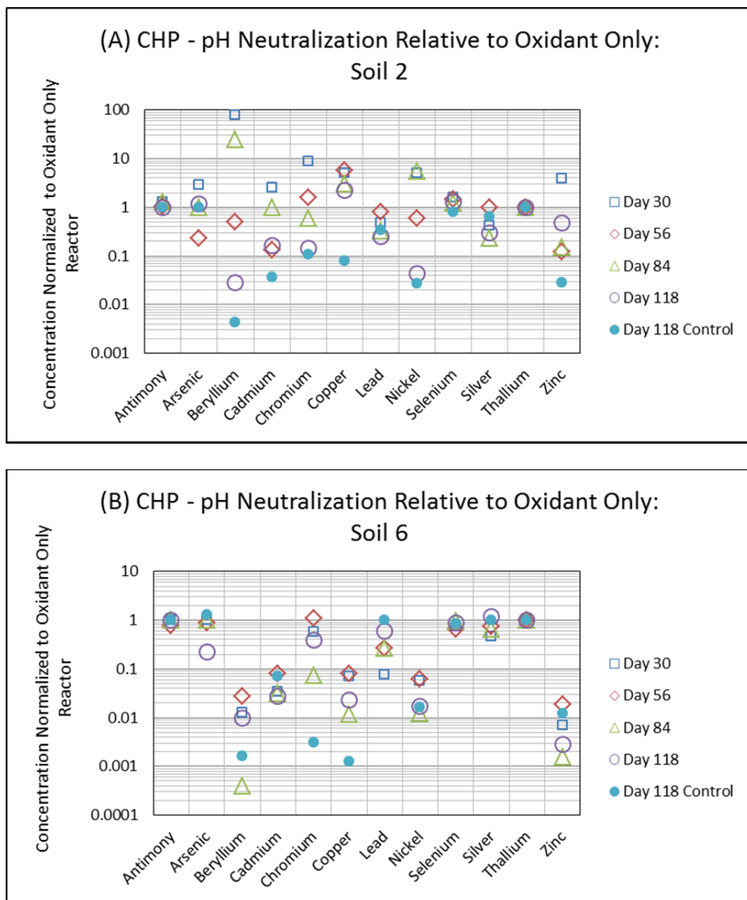
Figure 4.4.66 Post-Treatment Chemical Stabilization of CHP System: Select normalized metal concentrations at 2, 28, 56, and 90 days
