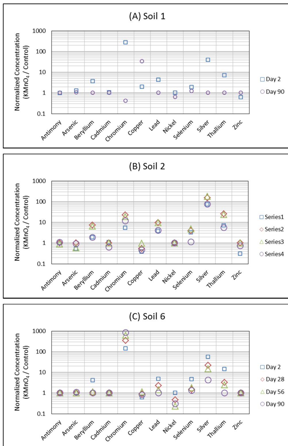
Figure 4.4.33 Co-Treatment Biological Stabilization: Normalized concentration of metals for reactors with PM applied versus control conditions (no PM treatment).
