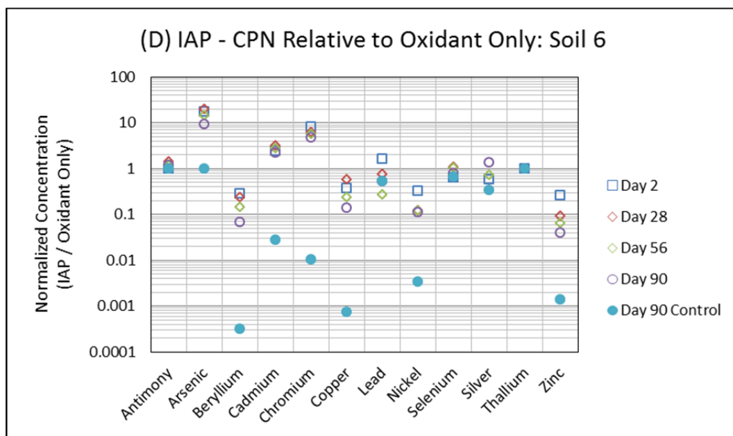
Figure 4.4.26 (cont.) Co-Treatment Biological Stabilization of IAP System: Select normalized metal concentrations at 2, 28, 56, and 90 days
