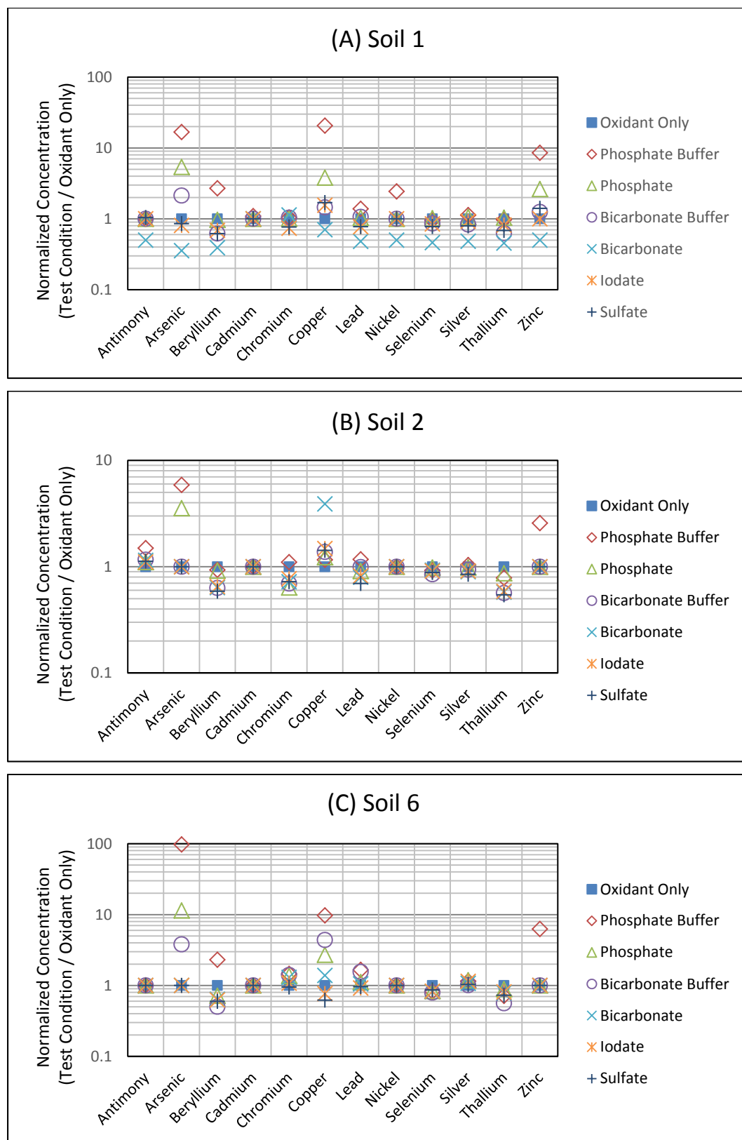
Figure 4.4.51 Co-Treatment Chemical Stabilization of PM System: Select normalized metal concentrations for 6 chemical treatment options.
