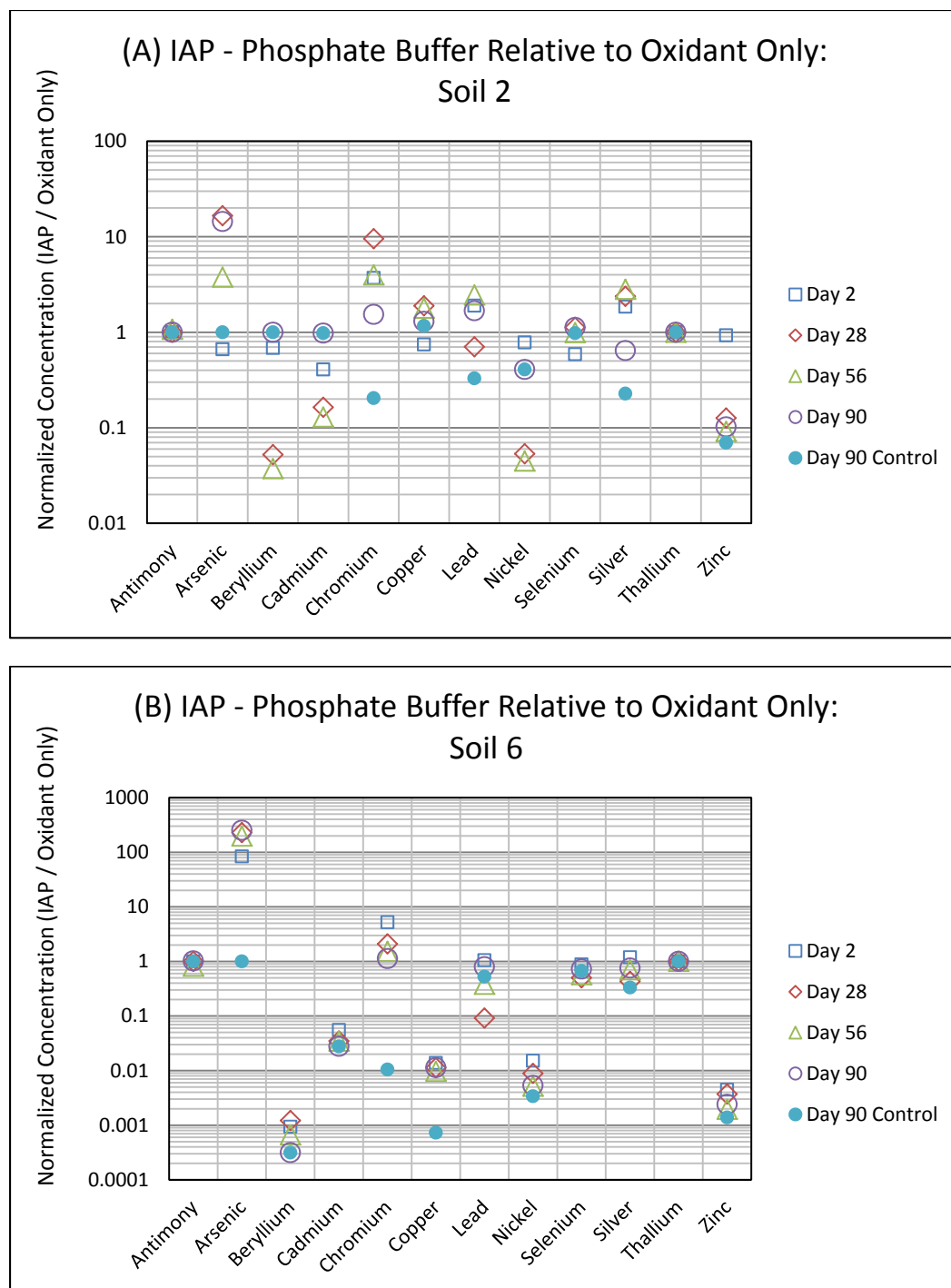
Figure 4.4.43 Co-Treatment Chemical Stabilization of IAP System: Select normalized metal concentrations at 2, 28, 56, and 90 days
