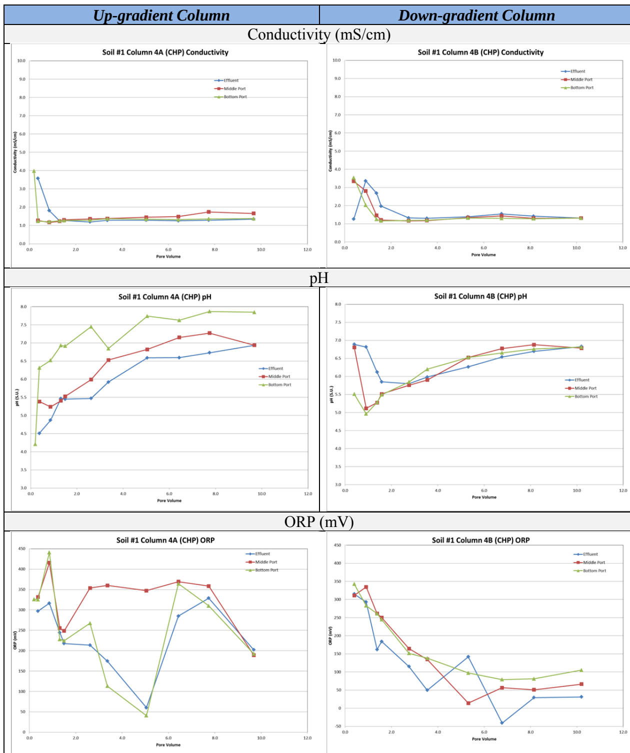
Figure 4.3.15 Column Experiment: Soil #1 with CHP Treatment – Geochemical variation with increasing groundwater PV.
