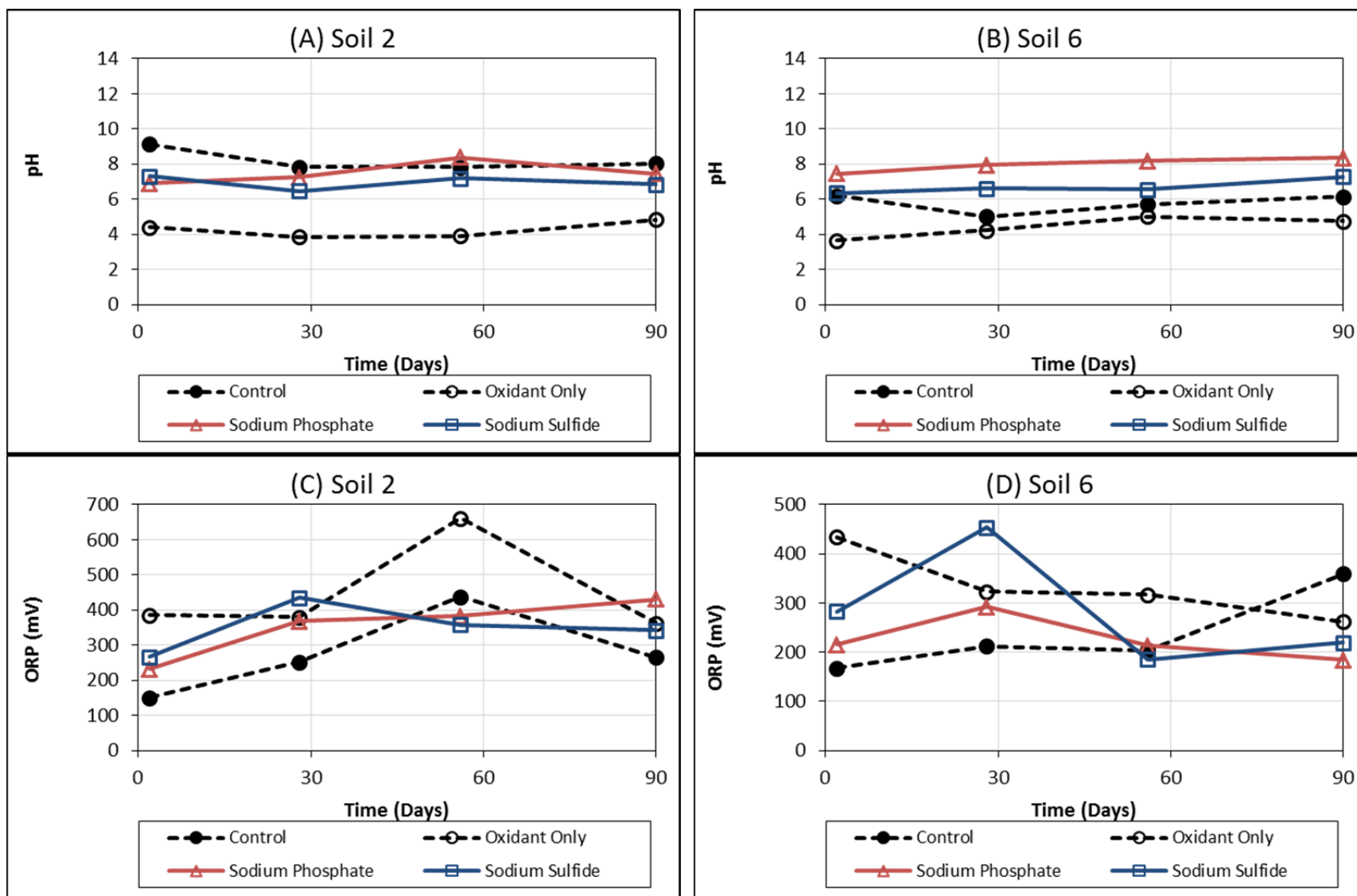
Figure 4.4.13 Pretreatment Stabilization of CHP System: Geochemical parameters at 2, 28, 56, and 90 days
