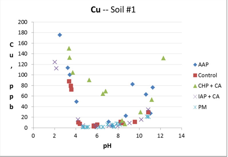
Figure 4.2.9 Detailed pH Evaluation: pH-dependent leaching of metals from Soil #1 Note: (AAP = alkaline-activated persulfate; CHP = iron-catalyzed hydrogen peroxide; CA = citric acid chelating agent; IAP = iron-activated persulfate; PM = permanganate)
