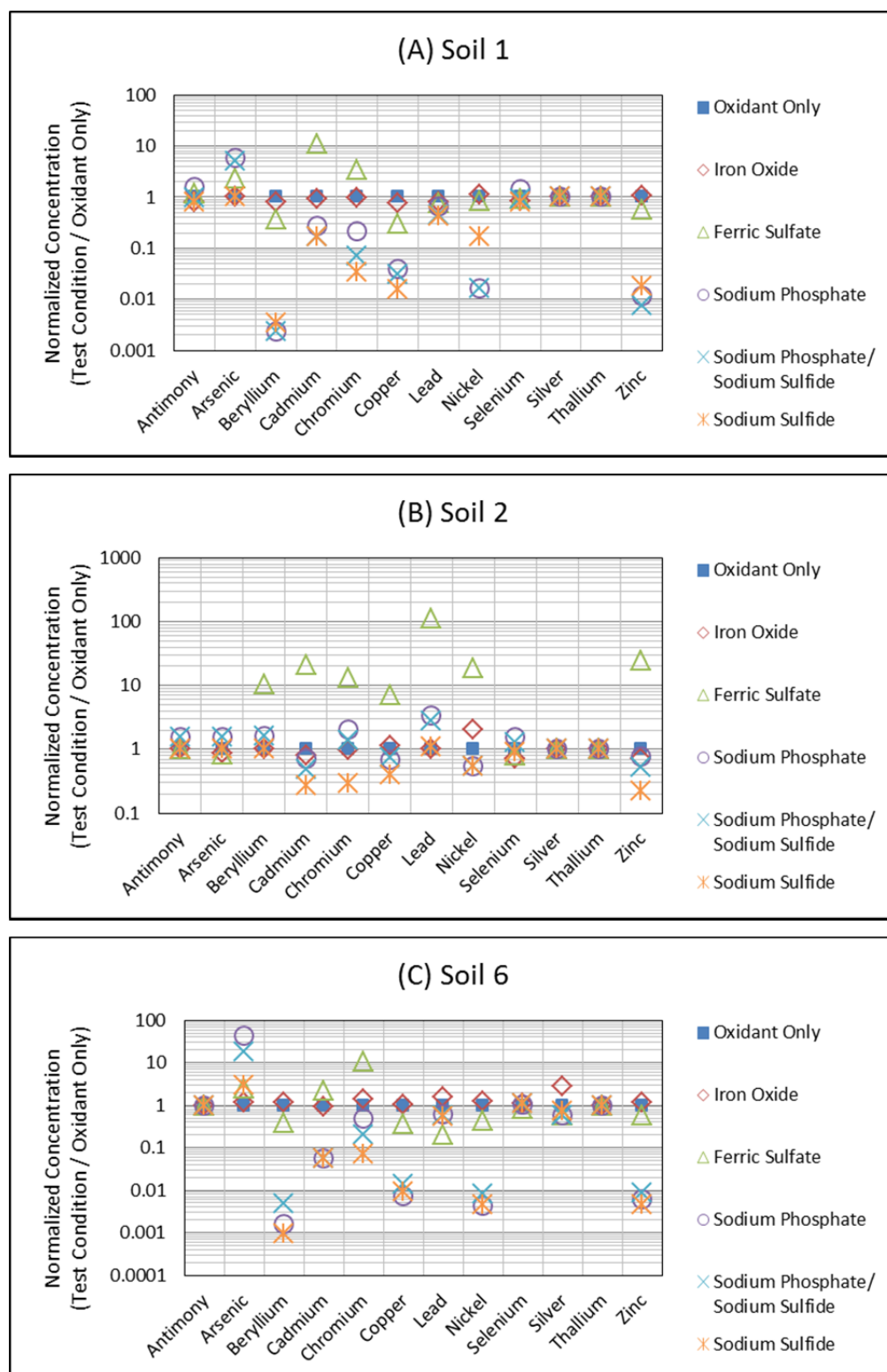
Figure 4.4.7 Pretreatment Stabilization of IAP System: Select normalized metal concentrations for 5 Pretreatment options.
