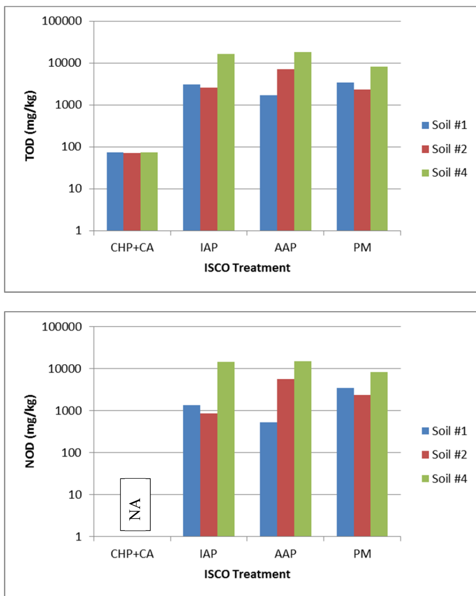
Figure 4.3.1 TOD and NOD of 3 ISCO Soils
