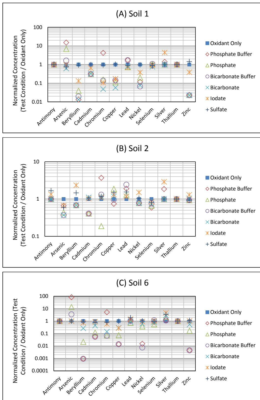
Figure 4.4.41 Co-Treatment Chemical Stabilization: Select normalized metal concentrations for 6 chemical treatment options.
