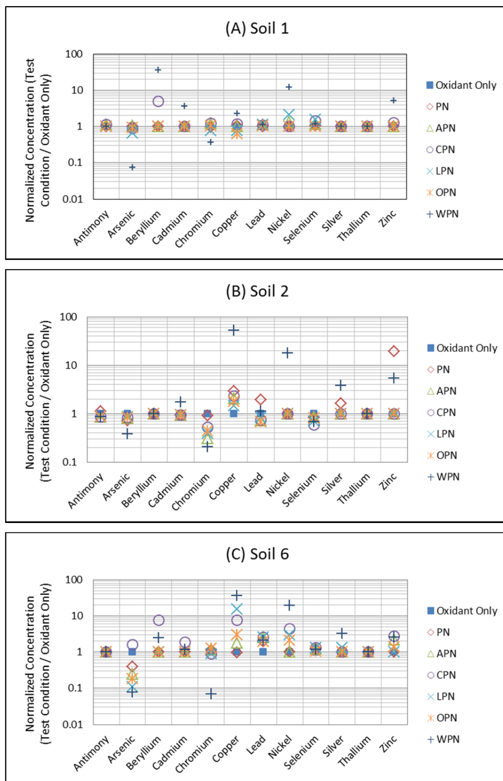
Figure 4.4.22 Co-Treatment Biological Stabilization of AAP System: Select normalized metal concentrations for 6 biological treatment options.
