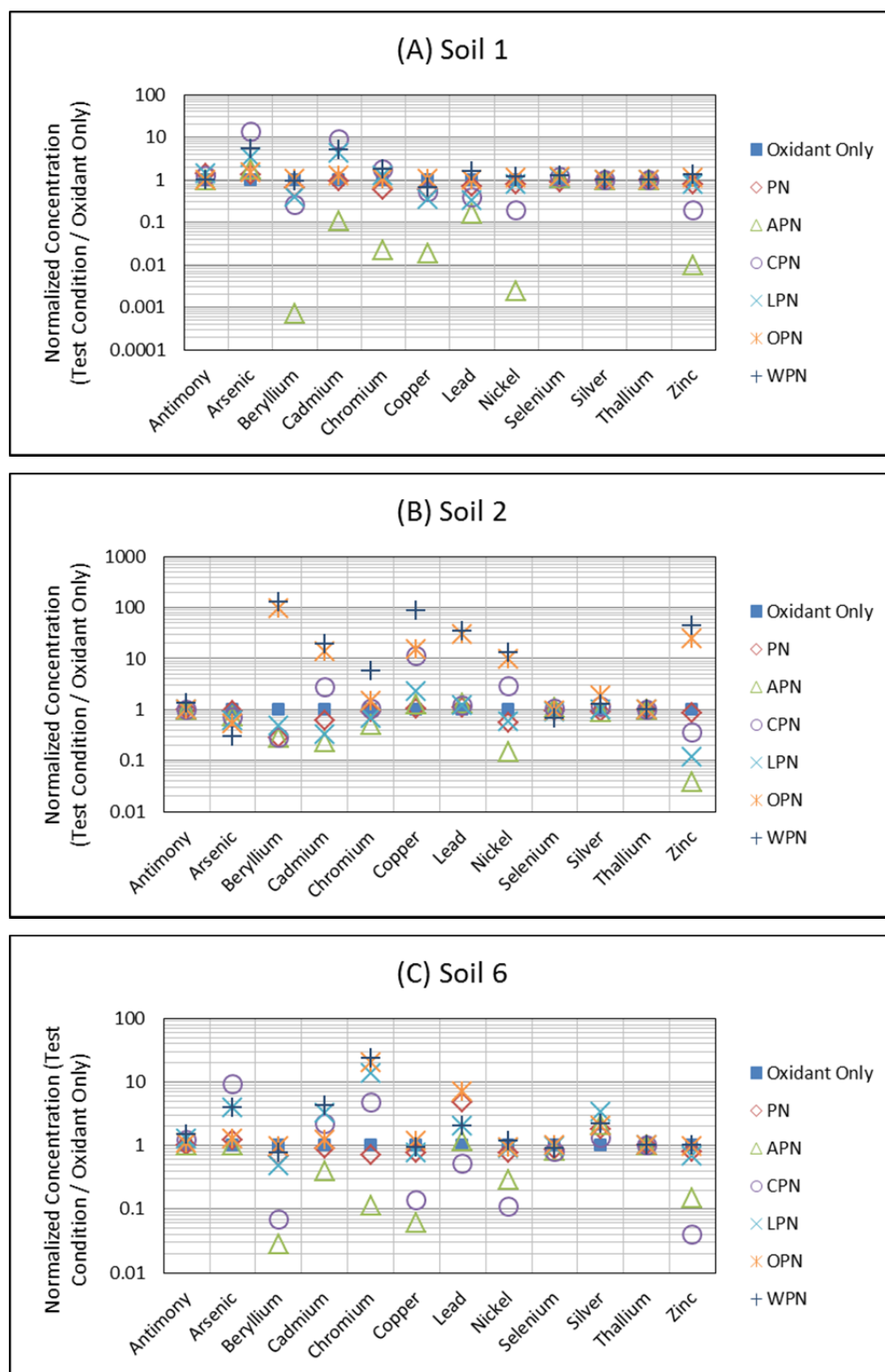
Figure 4.4.24 Co-Treatment Biological Stabilization: Select normalized metal concentrations for 6 biological treatment options
