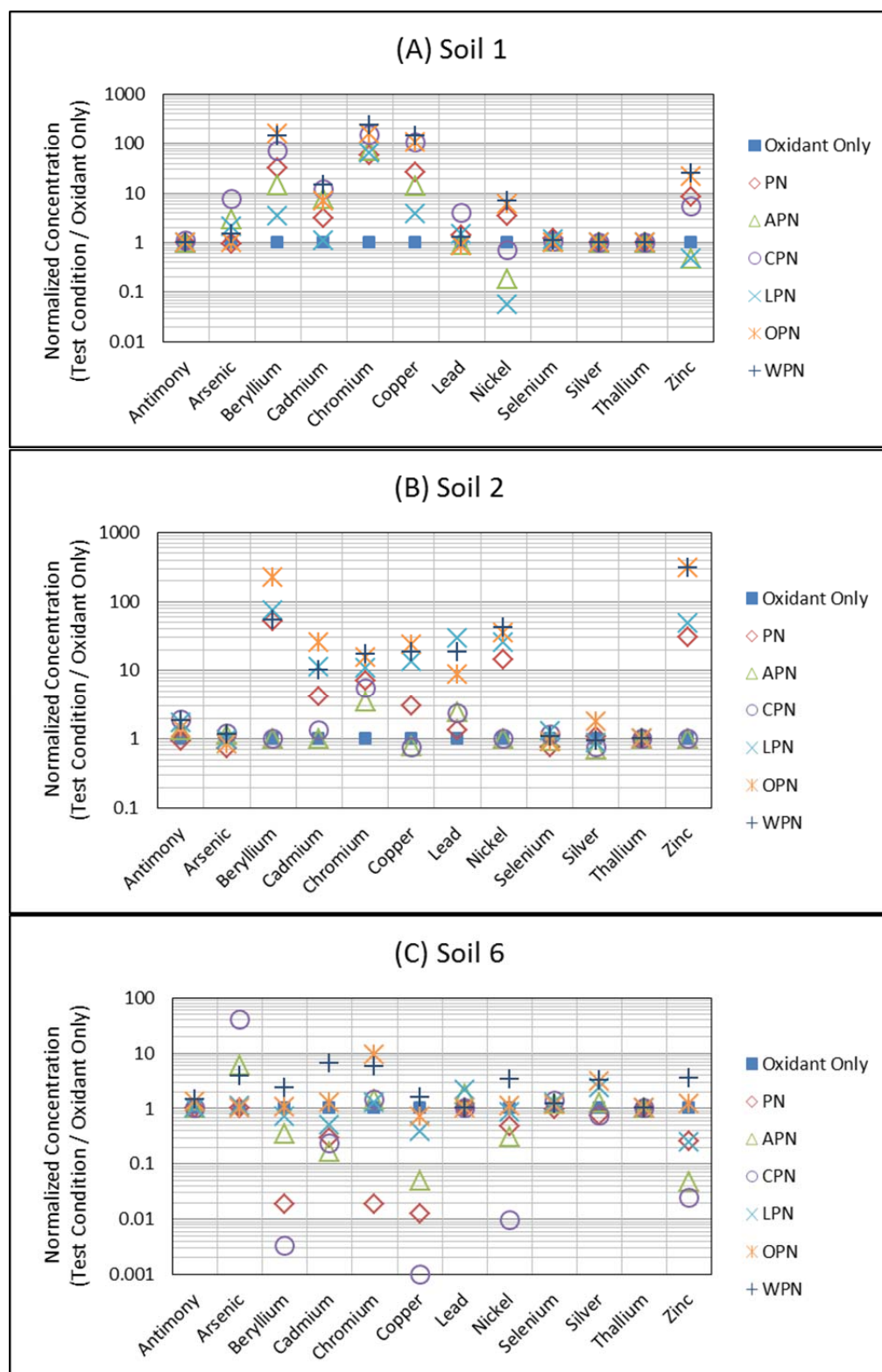
Figure 4.4.29 Co-Treatment Biological Stabilization of CHP System: Select normalized metal concentrations for 6 biological treatment options
