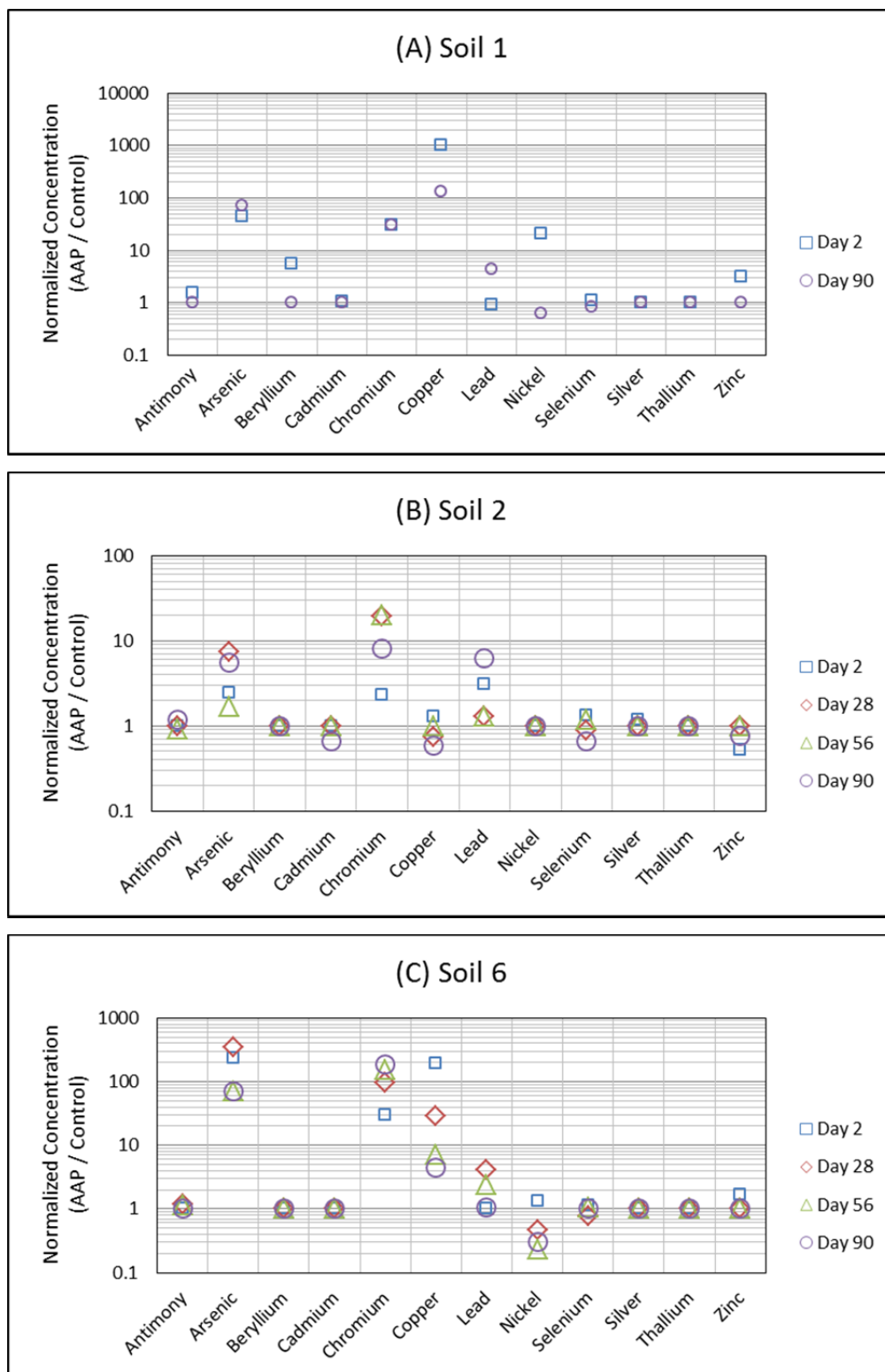
Figure 4.4.21 Co-Treatment Biological Stabilization: Normalized concentration of metals for reactors with AAP applied versus control conditions (no AAP treatment).
