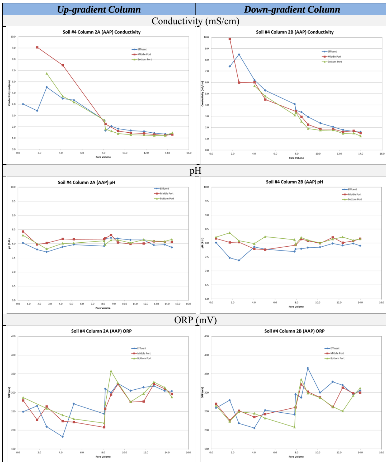
Figure 4.3.8 Column Experiment: Soil #4 with AAP Treatment – Geochemical variation with increasing groundwater PV.
