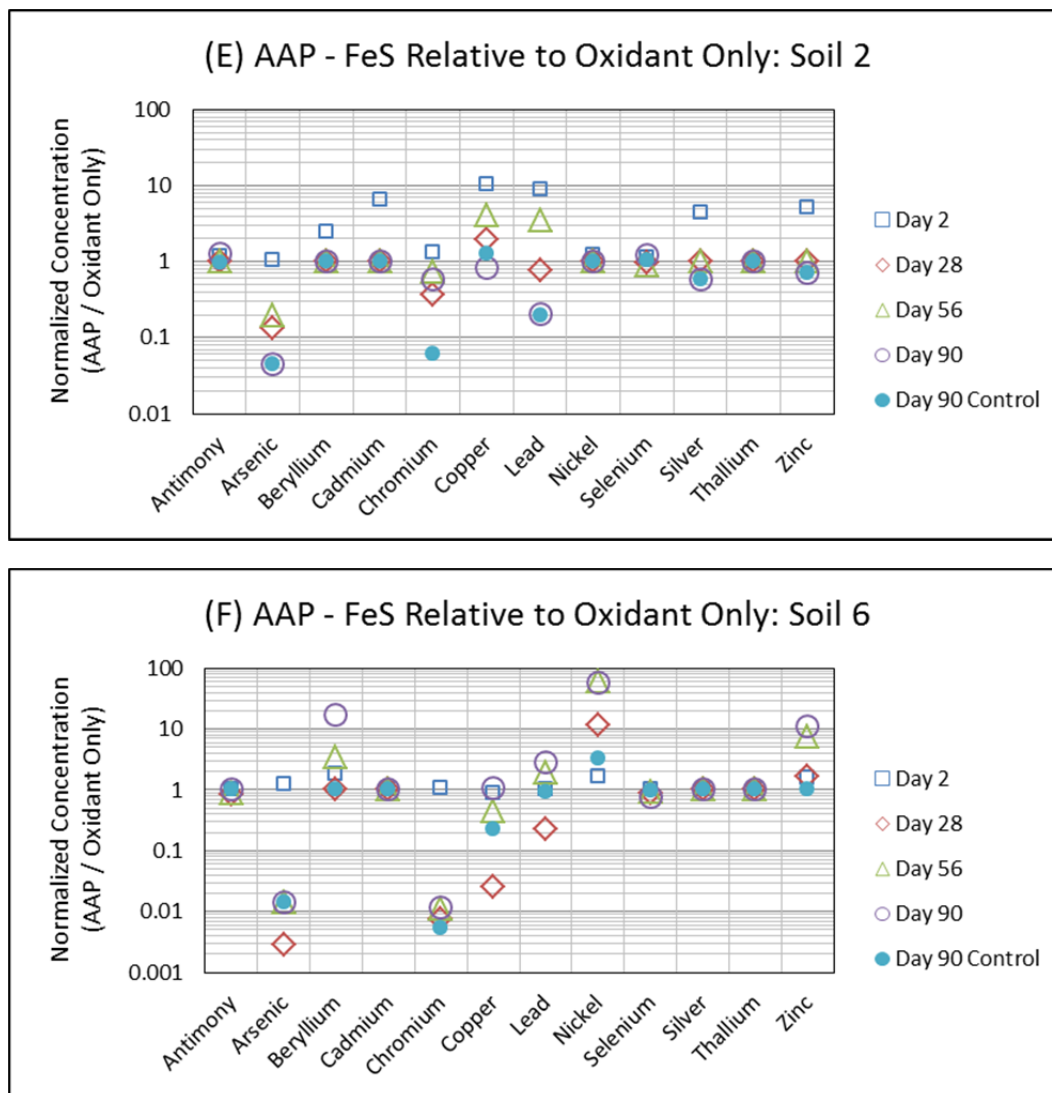
Figure 4.4.4 (cont.) Pretreatment Stabilization of AAP System: Select normalized metal concentrations at 2, 28, 56, and 90 days
