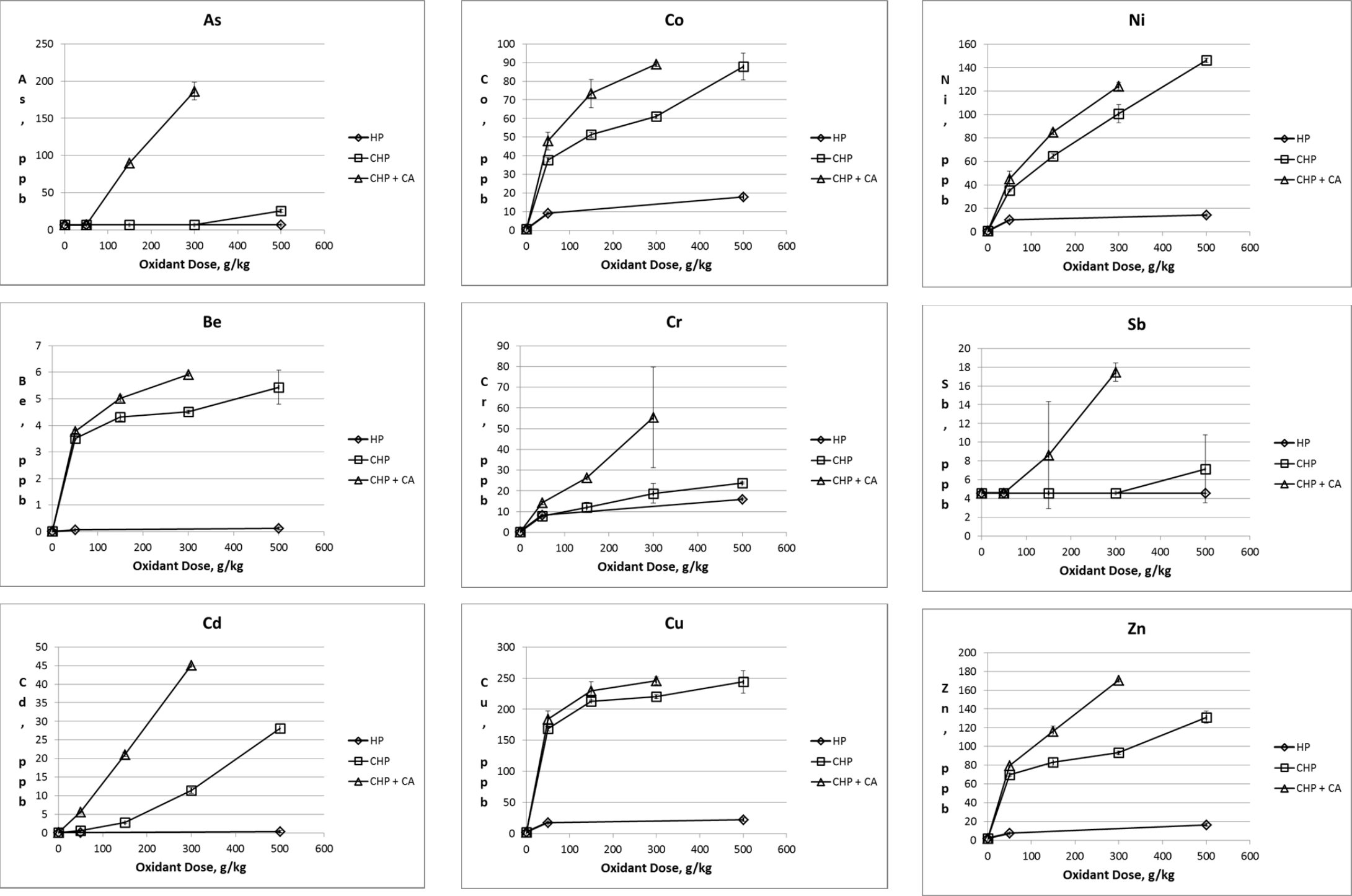
Figure 4.2.6 Initial Screening: Metals mobilization as a function of peroxide dose for soil#1 (HP = hydrogen peroxide; CHP = iron-activated hydrogen peroxide; CA = citric acid chelating agent)
