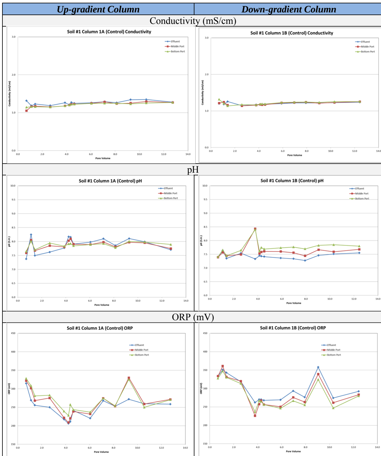
Figure 4.3.12 Column Experiment: Soil #1 with Control Treatment (groundwater only) – Geochemical variation with increasing groundwater PV..
