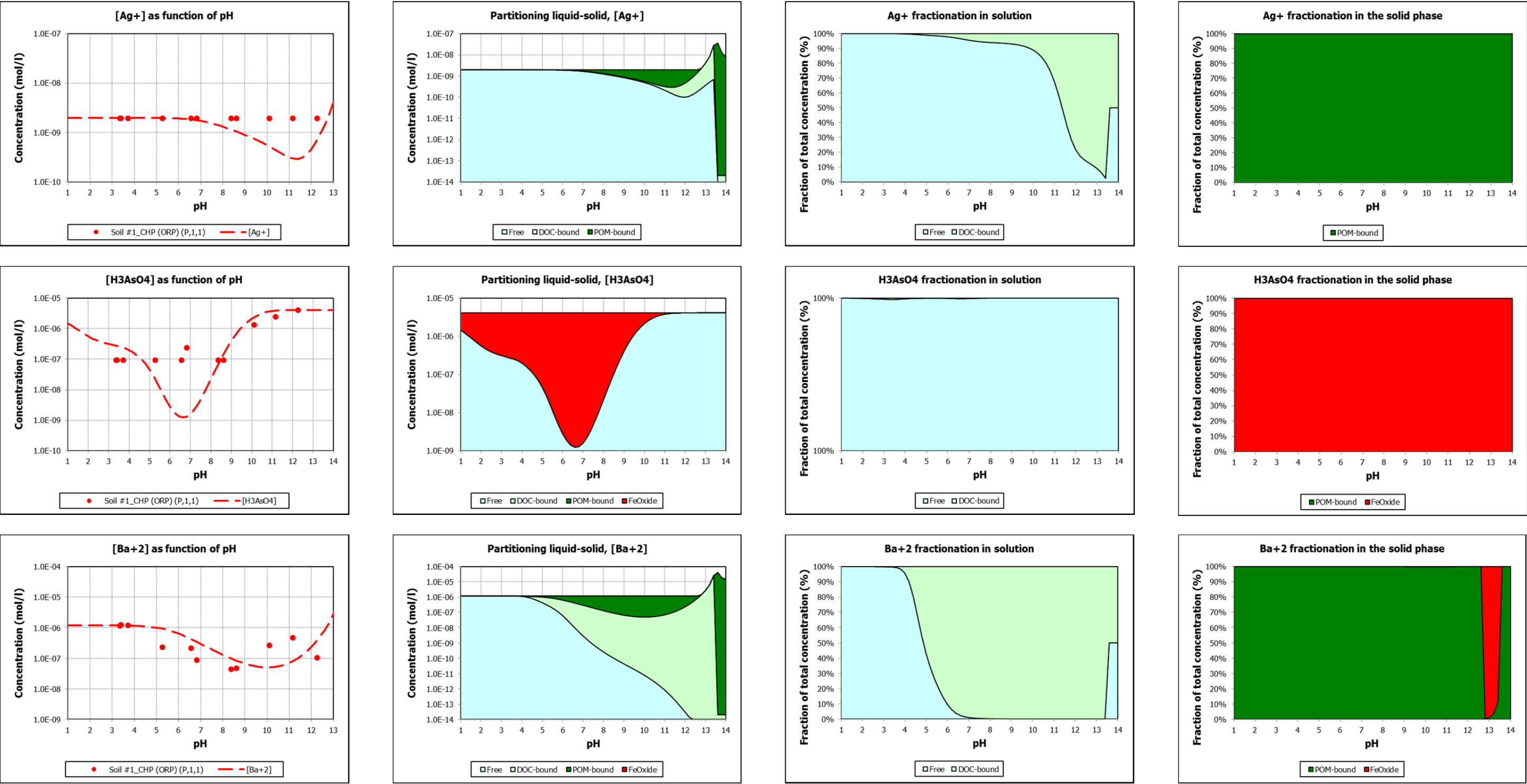
Figure 4.2.15 Geotechnical Modeling: Metal release and partitioning in the presence of CHP in Soil #1. The first graph in each row depicts the solubility of a given metal (symbols and line represent experimental data and model prediction, respectively) The subsequent graphs in the row show the liquid-solid partitioning and the solution and solid phase fractionation of the same metal.
