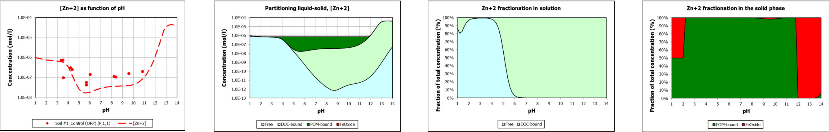
Figure 4.2.12 (cont.) Geotechnical Modeling: Metal release and partitioning in Soil #1. The first graph in each row depicts the solubility of a given metal (symbols and line represent experimental data and model prediction, respectively). The subsequent graphs in the row show the liquid-solid partitioning and the solution and solid phase fractionation of the same metal.
