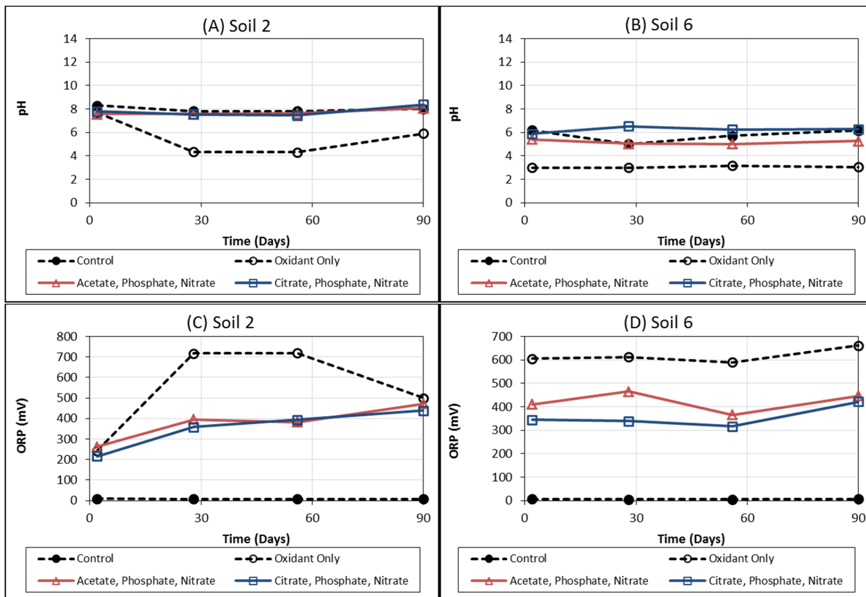
Figure 4.4.25 Co-Treatment Biological Stabilization of IAP System: Geochemical parameters at 2, 28, 56, and 90 days
