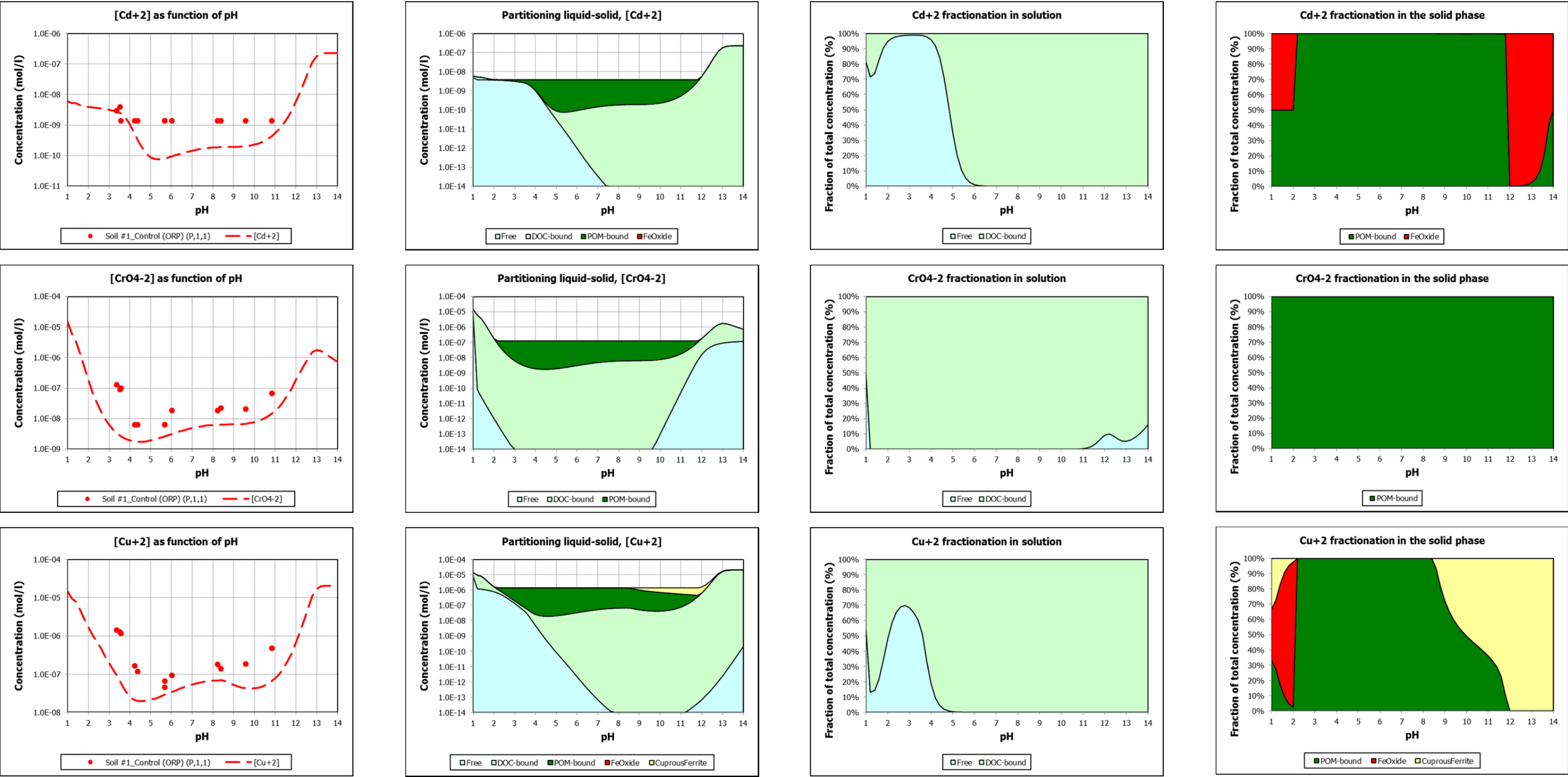
Figure 4.2.12 (cont.) Geotechnical Modeling: Metal release and partitioning in Soil #1. The first graph in each row depicts the solubility of a given metal (symbols and line represent experimental data and model prediction, respectively). The subsequent graphs in the row show the liquid-solid partitioning and the solution and solid phase fractionation of the same metal.
