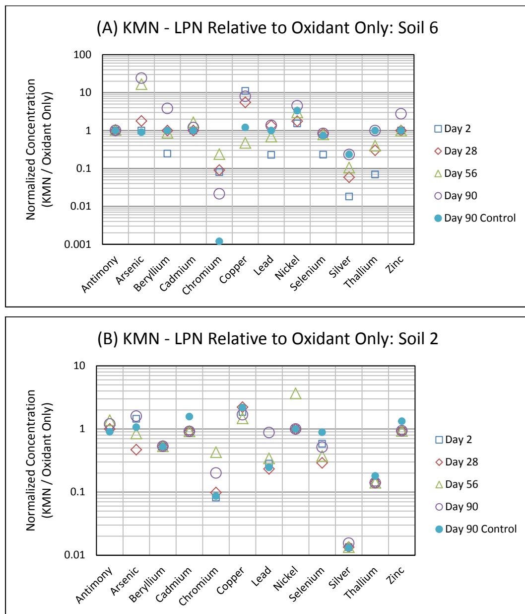
Figure 4.4.36 Co-Treatment Biological Stabilization of PM System: Select normalized metal concentrations at 2, 28, 56, and 90 days
