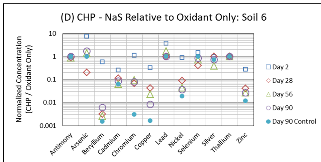
Figure 4.4.13 (cont.) Pretreatment Stabilization of CHP System: Select normalized metal concentrations at 2, 28, 56, and 90 days
