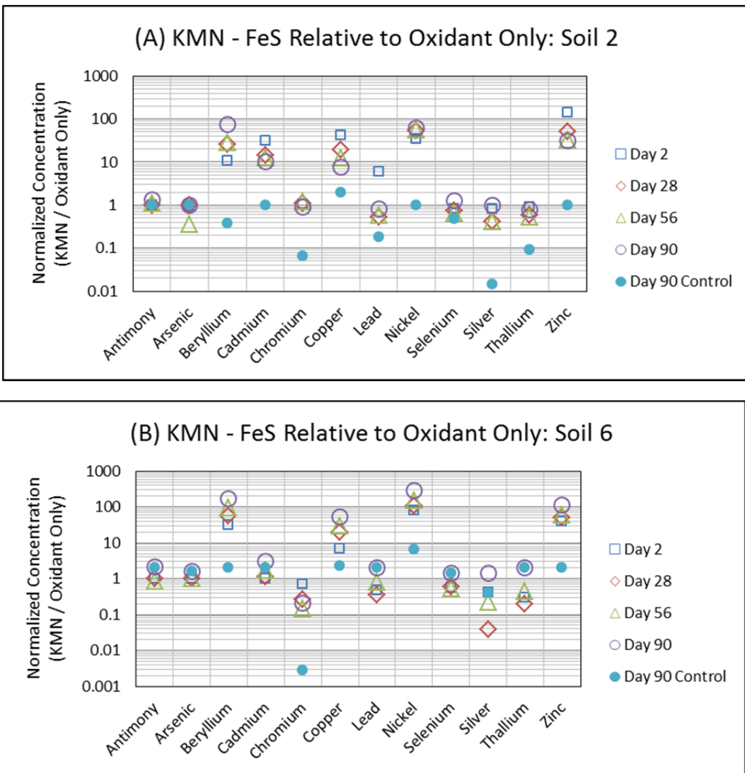
Figure 4.4.19 Pretreatment Stabilization of PM System: Select normalized metal concentrations at 2, 28, 56, and 90 days
