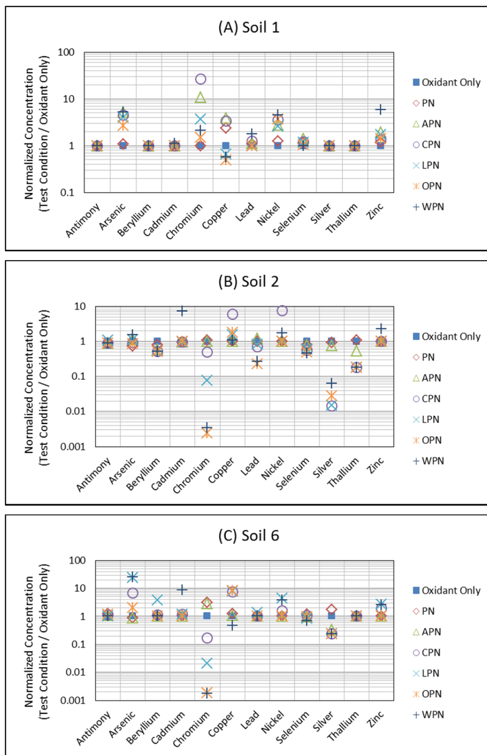
Figure 4.4.34 Co-Treatment Biological Stabilization of PM System: Select normalized metal concentrations for 6 biological treatment options
