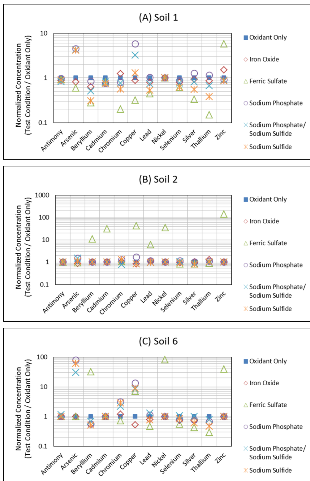
Figure 4.4.17 Pretreatment Stabilization of PM System: Select normalized metal concentrations for 5 Pretreatment options.
