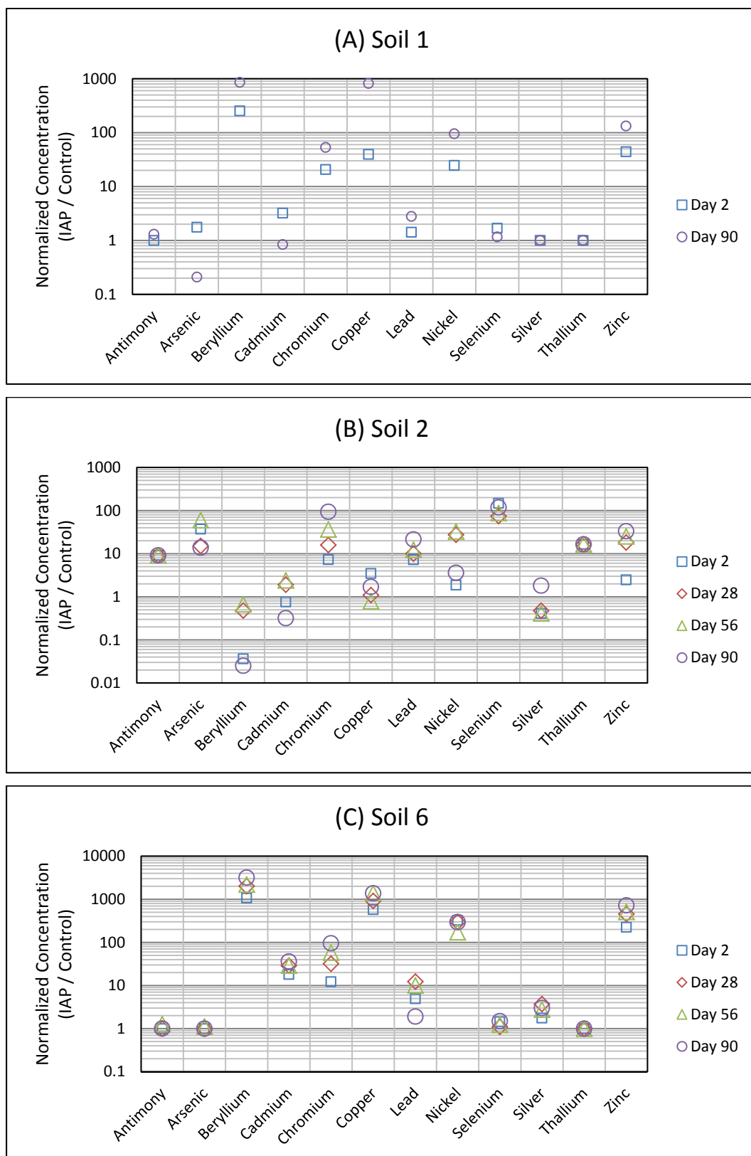
Figure 4.4.40 Co-Treatment Chemical Stabilization: Normalized concentration of metals for reactors with IAP applied versus control conditions (no IAP treatment).
