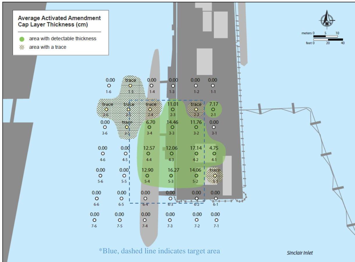
Figure 49. Activated Carbon Amendment Thickness during the 0.5-month Post-placement SPI Survey (Germano and Associates 2013b).
