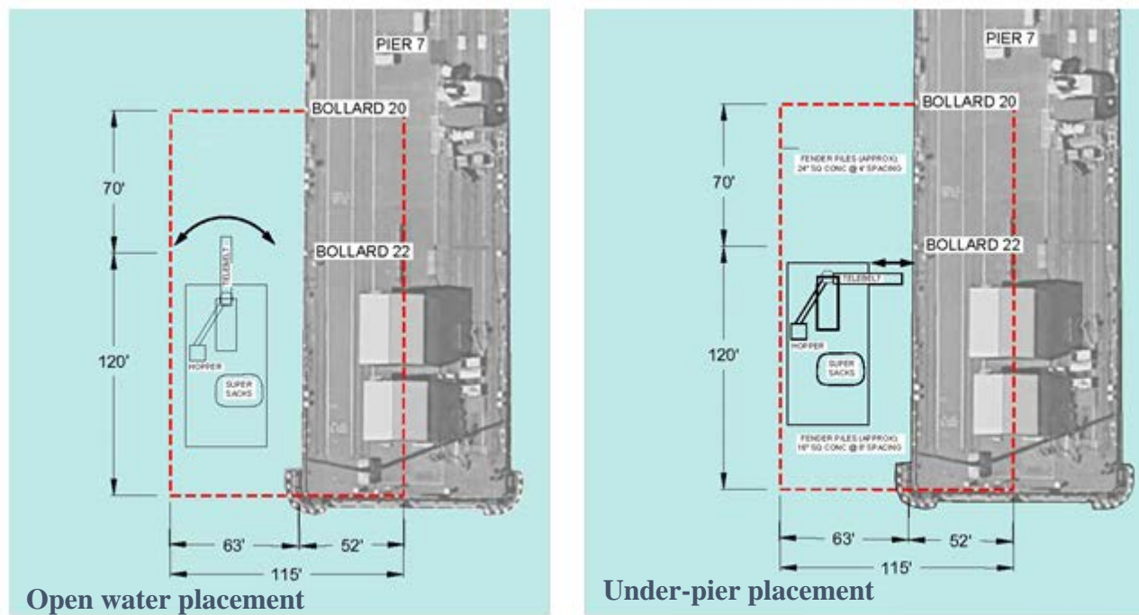
Figure 7. AquaGate Amendment Placement Approaches with the Telebelt System Including Open-berth Method (Left), and Under-pier Method (Right).
