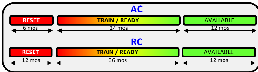
Figure 1. ARFORGEN Model
