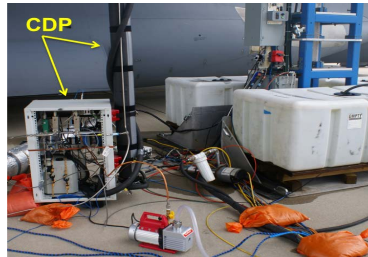
Figure 27. Dilution chamber (DC) and Condensation Dilution Probe (CDP) installed near engine during C-17 demonstration
