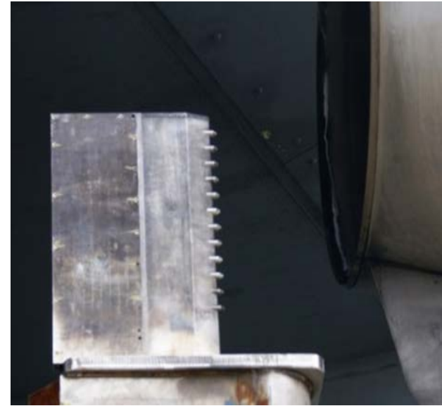
Figure 26. Emissions sampling probes at engine exit, 10m and 20 m, and probe rake for engine exit plane emission sampling
