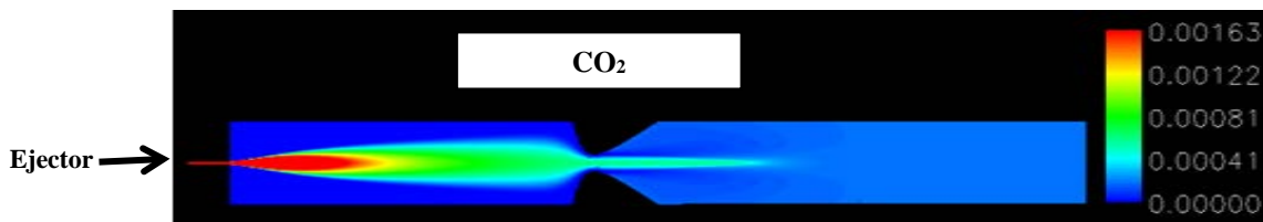
Figure 3. Axisymmetric radial CO 2 distribution as a function of axial distance in dilution chamber for a dilution ratio of 100:1
