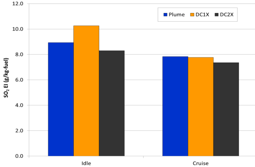
Figure 38. T63 Engine SO 2 emission indices for sulfur-doped JP-8 (JP-8S) fuel
