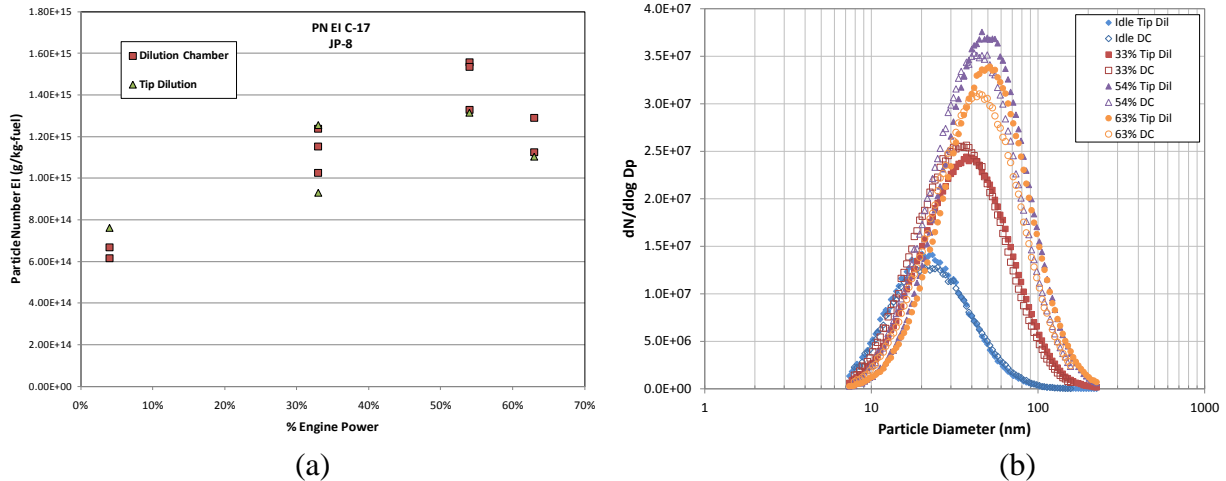
Figure 7. Average PM measurements in PW-F117 engine at several power settings for probe-tip and N 2 diluted dilution chamber: (a) Particle number EI, (b) Particle Size Distribution
