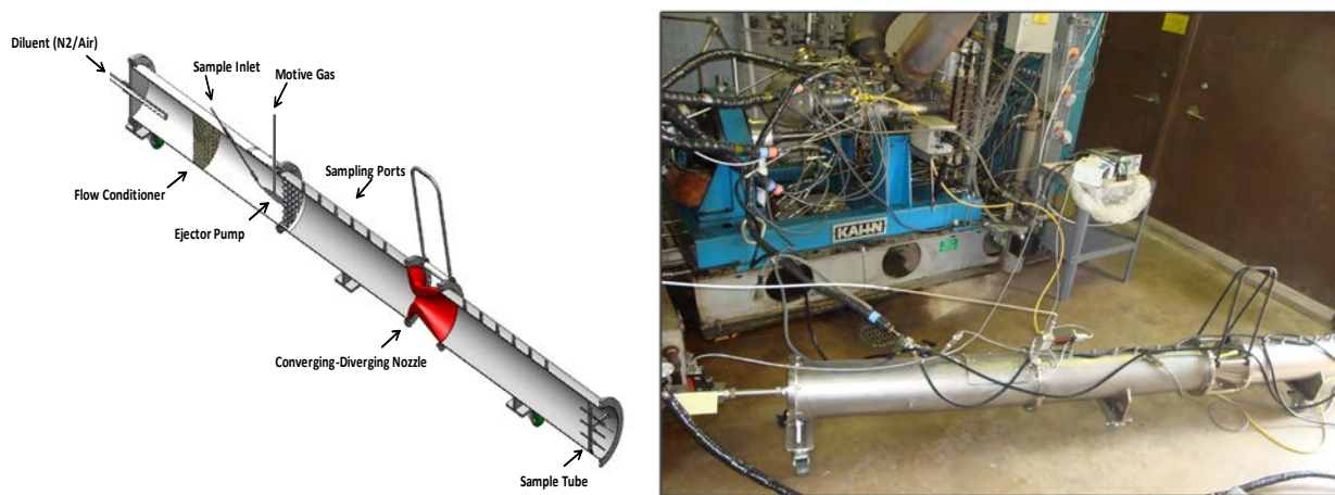
Figure 2. Schematic of dilution chamber (DC) and implementation of DC on T63 engine
