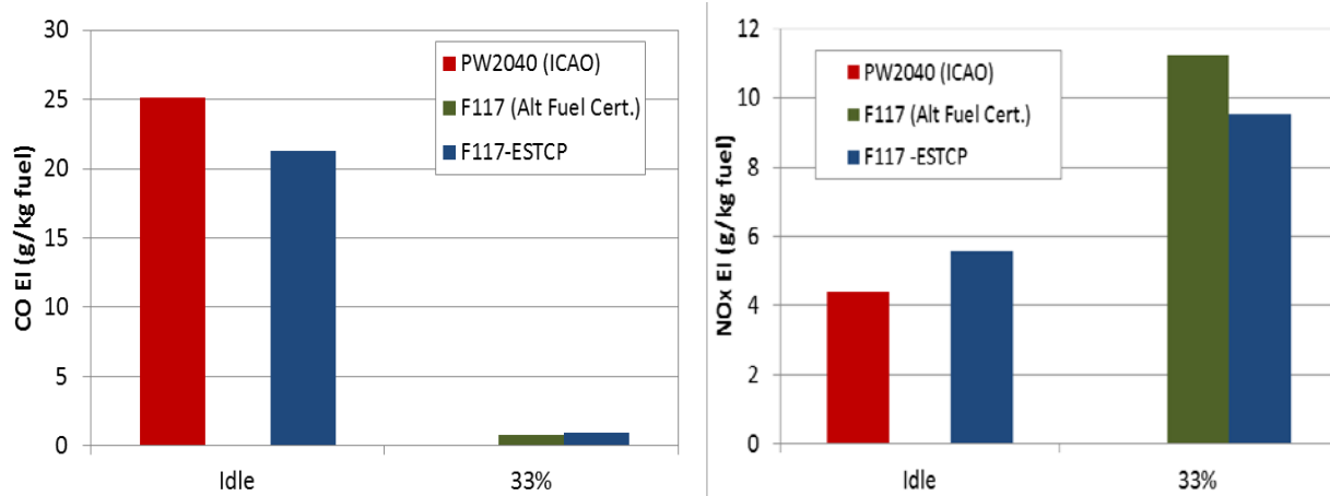
Figure 46. Comparison of CO and NO x emissions between PW-F17 engines and commercial variant engine (data from ICAO Databank) at idle and 33% max thrust
