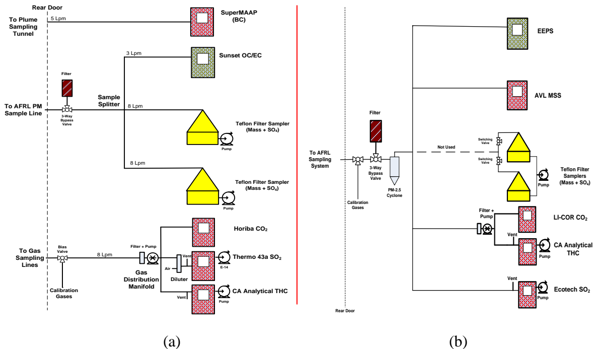
Figure 16. EPA instrumentation and equipment setup for demonstrations on (a) T63 and (b) C-17 engine
