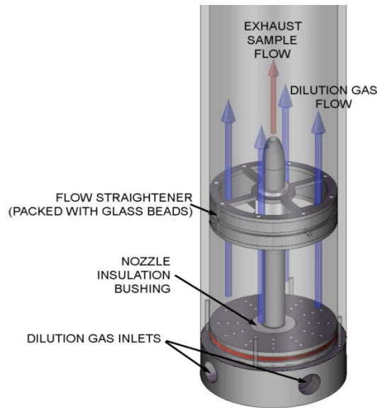
Figure 5. Schematic of the inlet region of the condensation dilution probe
