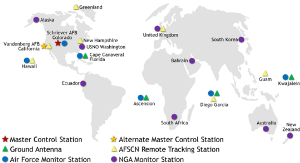
Figure 1. GPS Ground Control Segment 105
