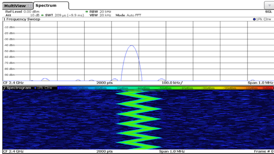
Figure 73. Instantaneous Transmitting Frequency of FMCW Signal in Frequency Domain at t = t_1
