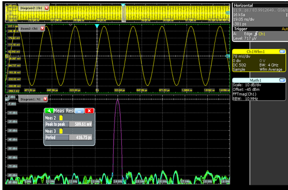
Figure 15. Screenshot of Measurement Results for RF Cable PE300-36 using R&S RTO2000 Digital Oscilloscope at 2.4 GHz with Input Power of 0 dBm
