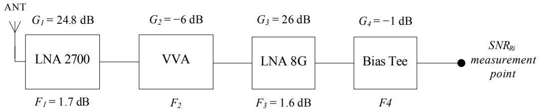
Figure 89. Cascade of LNAs and Bias Tee in Receiver
