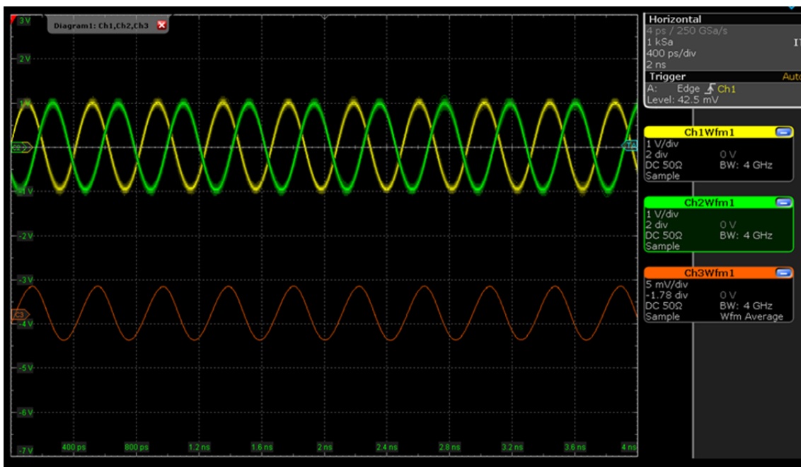
Figure 39. 90° Phase Shift between Reference and Measurement Channels with V_{bias} = 0.5 \text{ V}
