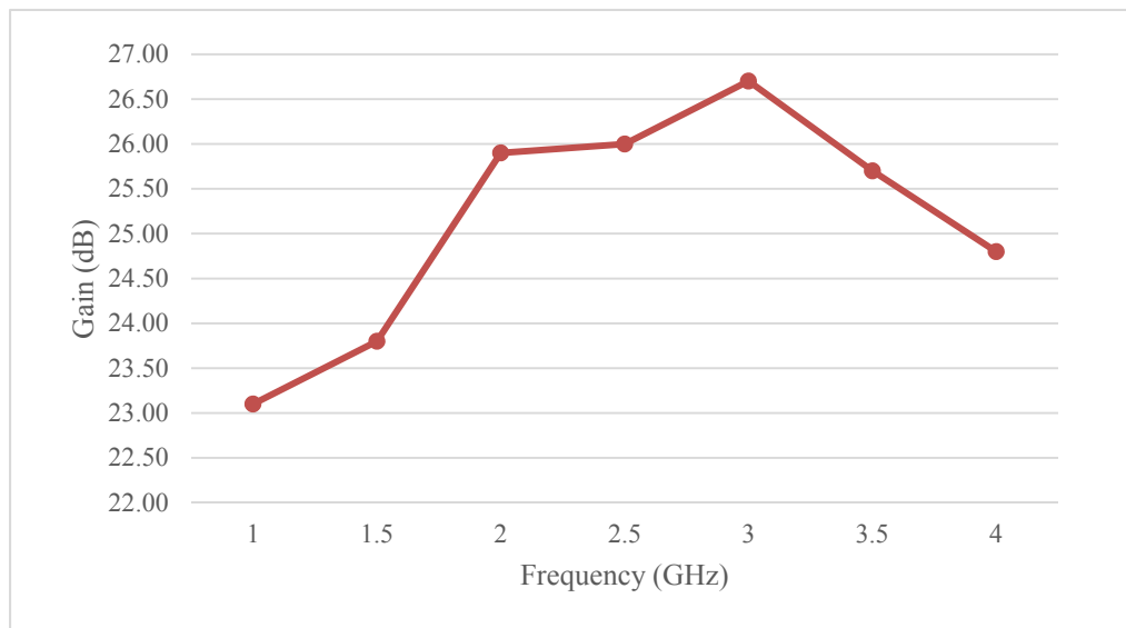
Figure 21. Gain versus Frequency for LNA 8G
