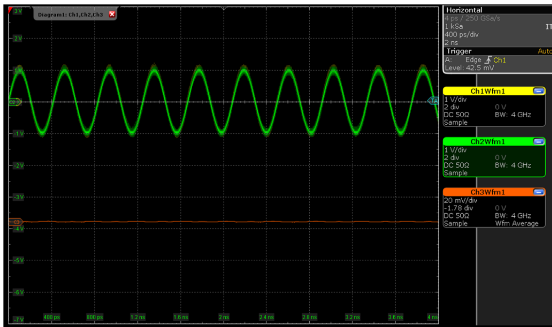
Figure 36. In-Phase Reference and Measurement Channel with V_{bias} = 0.0 V
