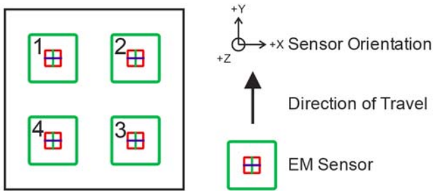
Figure 2-2: TEMTADS Coil Geometry
