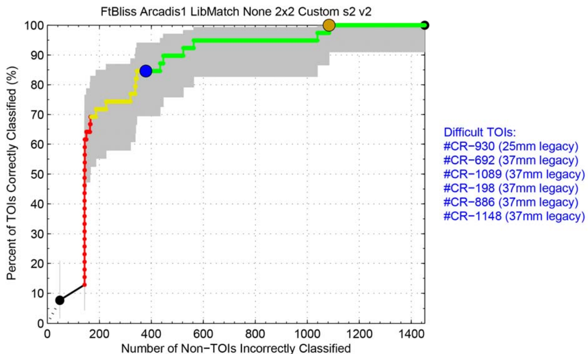
Figure 6-1: Analyst 1 ROC Curve
