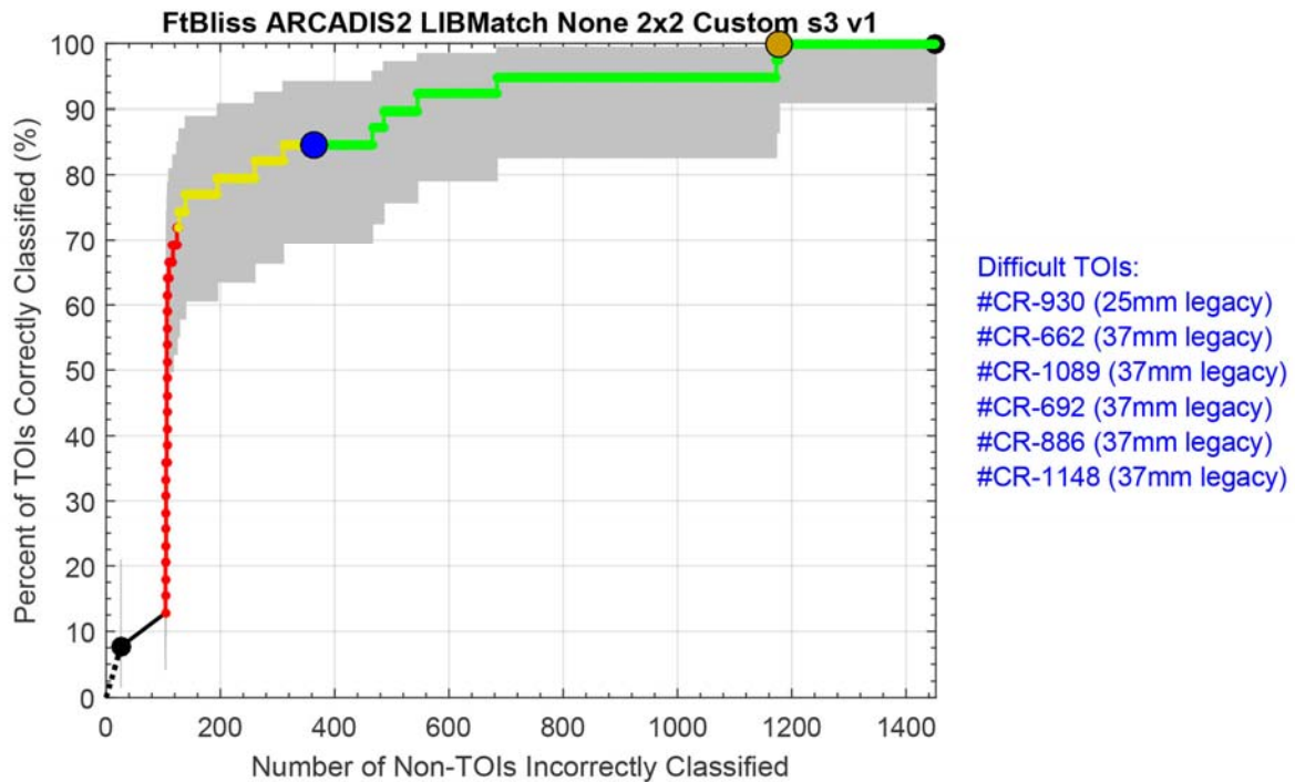
Figure 6-2: Analyst 2 ROC Curve
