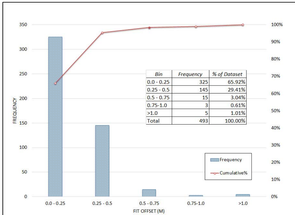
Figure 7-7: Analyst 2 Target Location Offset Distribution
