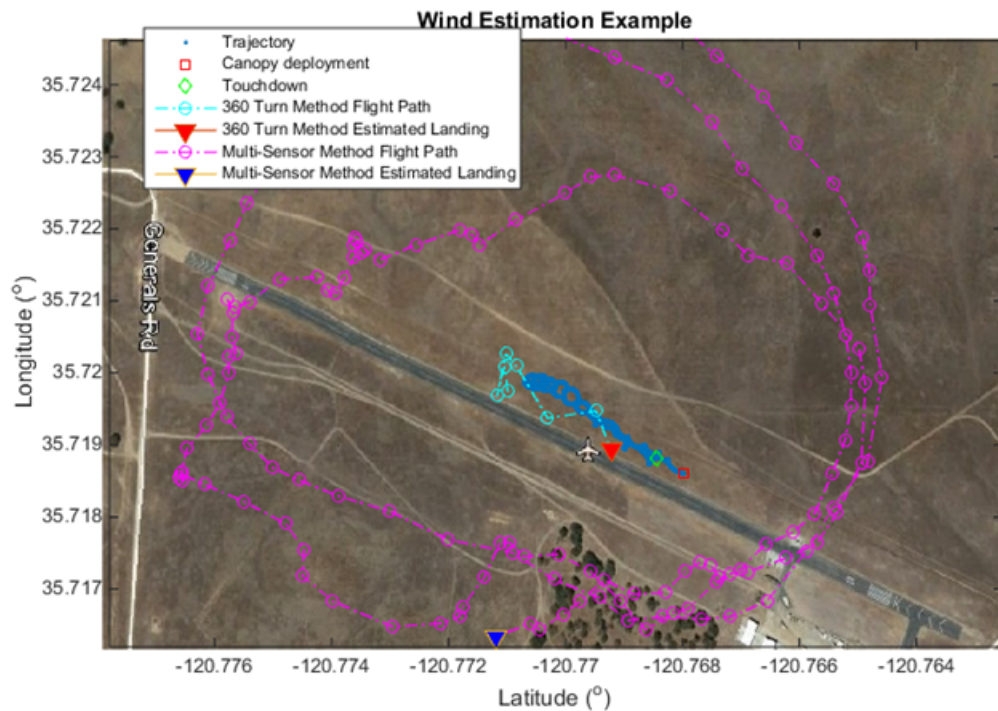
Figure 31. Zoomed-In Wind Estimation Example. Adapted from [18].
