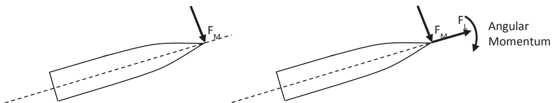
Figure 7. Direction of Overturning Moment and Lift Forces in a Spinning Projectile.
