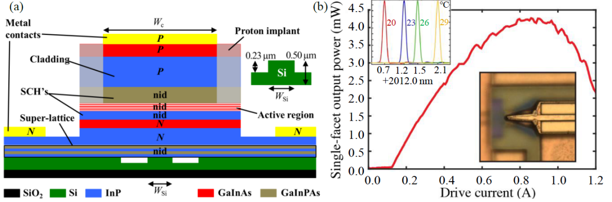
Figure 7. (a) Cross-section schematic of 2.0- \mu\text{m} laser or SOA on Si. (b) Output power characteristic with insets showing the laser spectra at different temperatures and a micrograph of the taper transition between the gain and passive regions.
