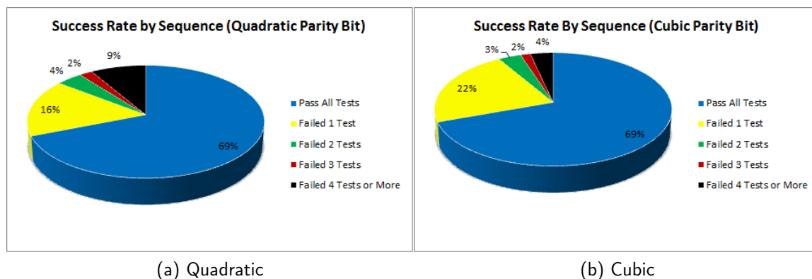
Figure 4.2: Quadratic versus Cubic Parity Sequence Results
