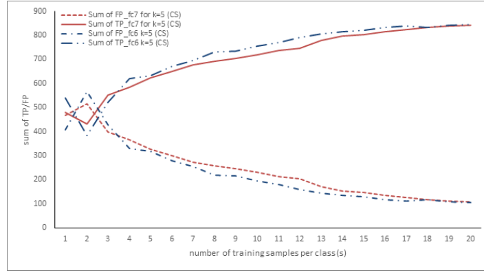
Figure B.9. Variation of TP and FP for Different Layers (CS, k=5 ).
