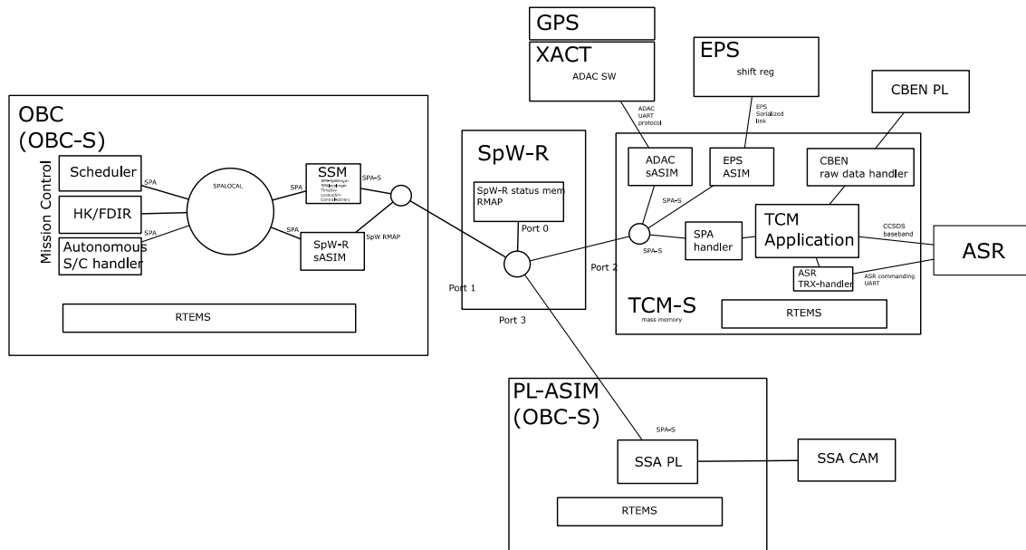
Figure 10. A broad view of the distributed software architecture throughout the SPARC-1 spacecraft.
