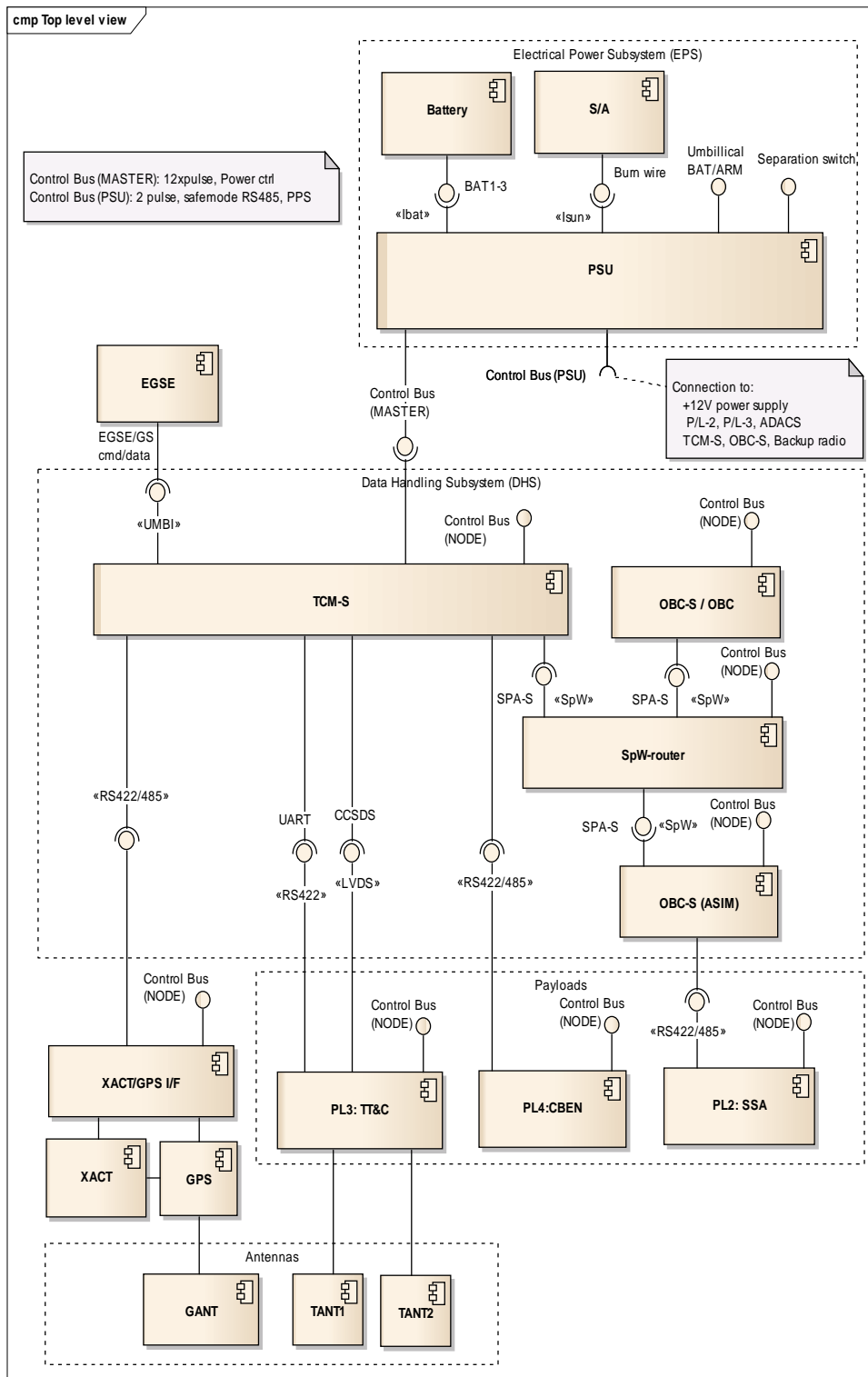
Figure 5. SPARC-1 top-level block diagram
