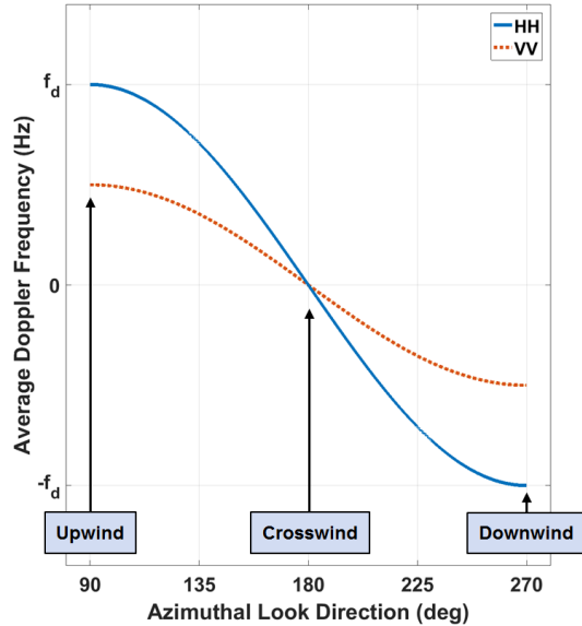
Fig. 2. The differential average Doppler across HH and VV co-polarizations is most pronounced when looking upwind and downwind. It goes to zero only when looking exactly crosswind.
