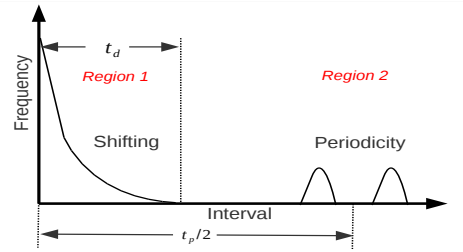
Fig. 3. Histogram of intervals between two consecutive flows with a specific feature quantized to the same discrete value.
