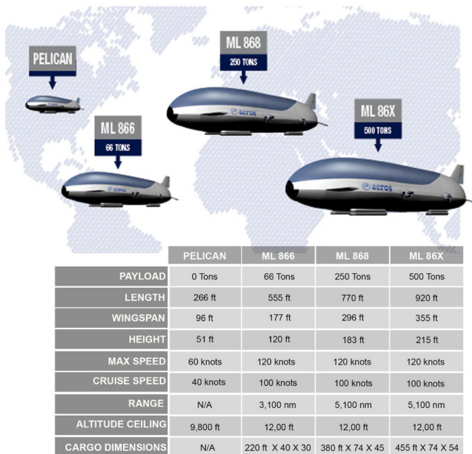
Figure 13 Technical characteristics on the existing and future Aeroscraft fleet of airships 25 [145]
