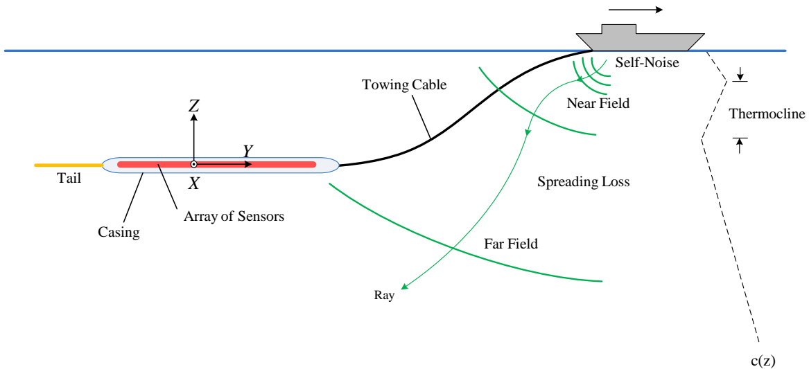
Figure 2 Towed sonar array (adapted from [4]).
