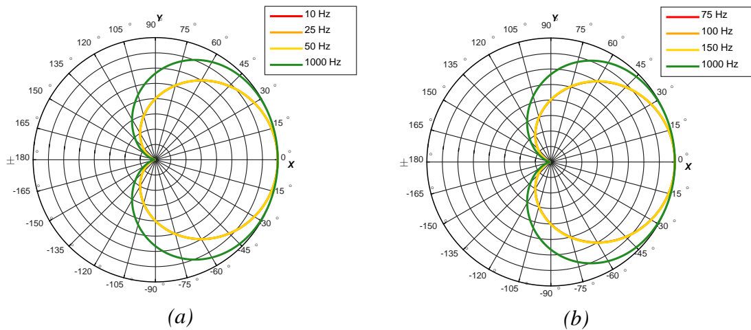
Figure 9 Equalized, horizontal FF beam patterns in the XY plane vs. bearing angle \psi and frequency.
