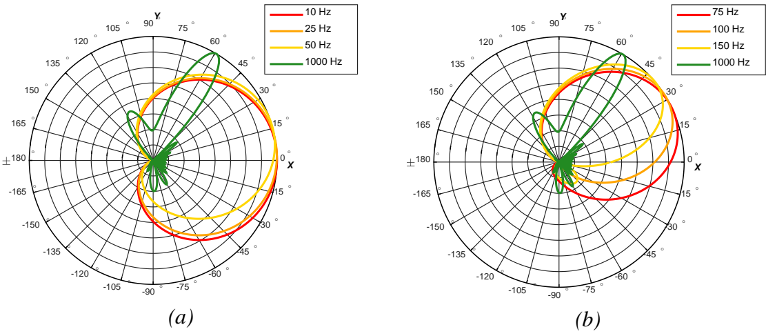
Figure 16 Equalized, horizontal FF beam patterns in the XY plane of a linear array of 11 triplets vs. frequency and bearing angle \psi , steered to 60°.
