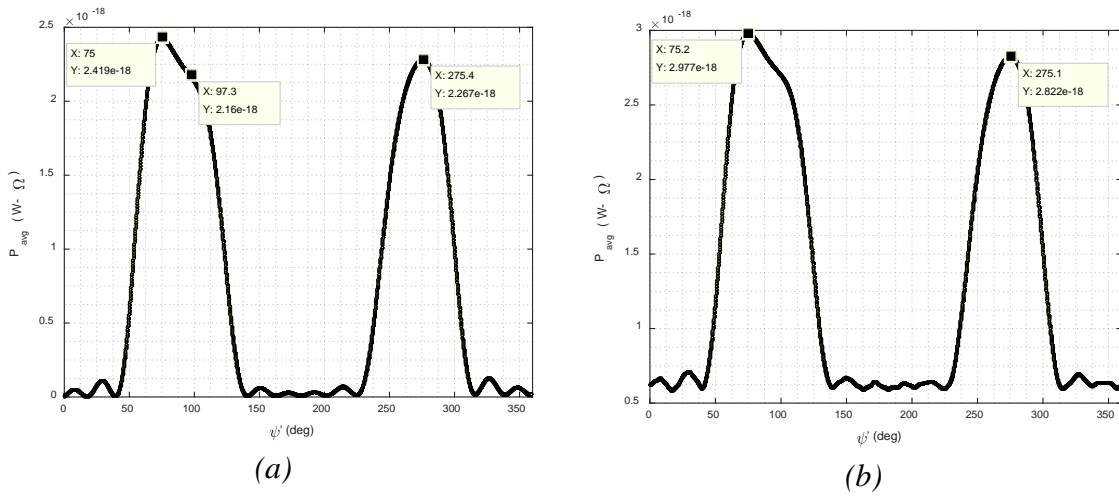
Figure 34 Time-average power (in W \cdot \Omega ) of r(t) vs. bearing angle \psi' for the target located at \psi_s = 75^\circ , with (a) no noise and (b) SNR = -3 dB.
