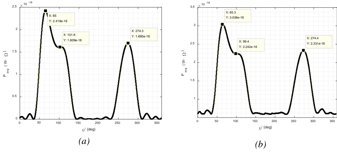
Figure 33 Time-average power (in W \cdot \Omega ) of r(t) vs. bearing angle \psi' for the target located at \psi_s = 65^\circ , with (a) no noise and (b) SNR = -3 dB.
