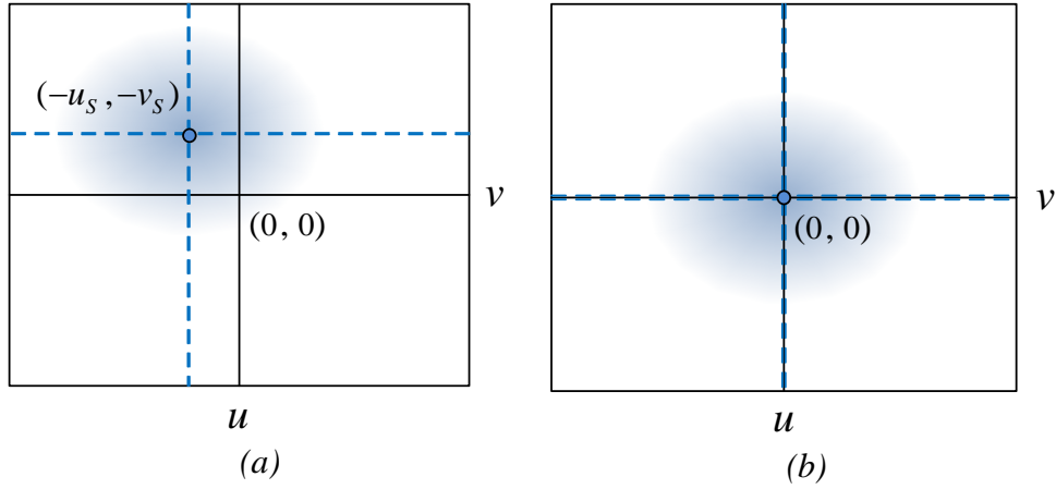
Figure 27 Normalized magnitude of \hat{R}(q, r, s) as a function of direction cosines u and v , (a) with no beam steering) and (b) using correct beam steering.
