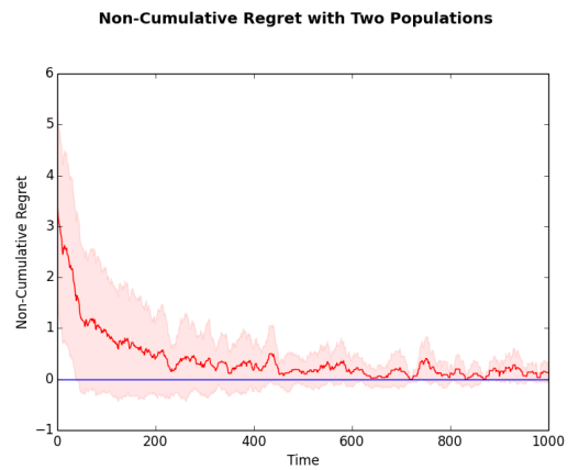
Figure 4.9: Non-cumulative Regret for Two (Mix) Populations
