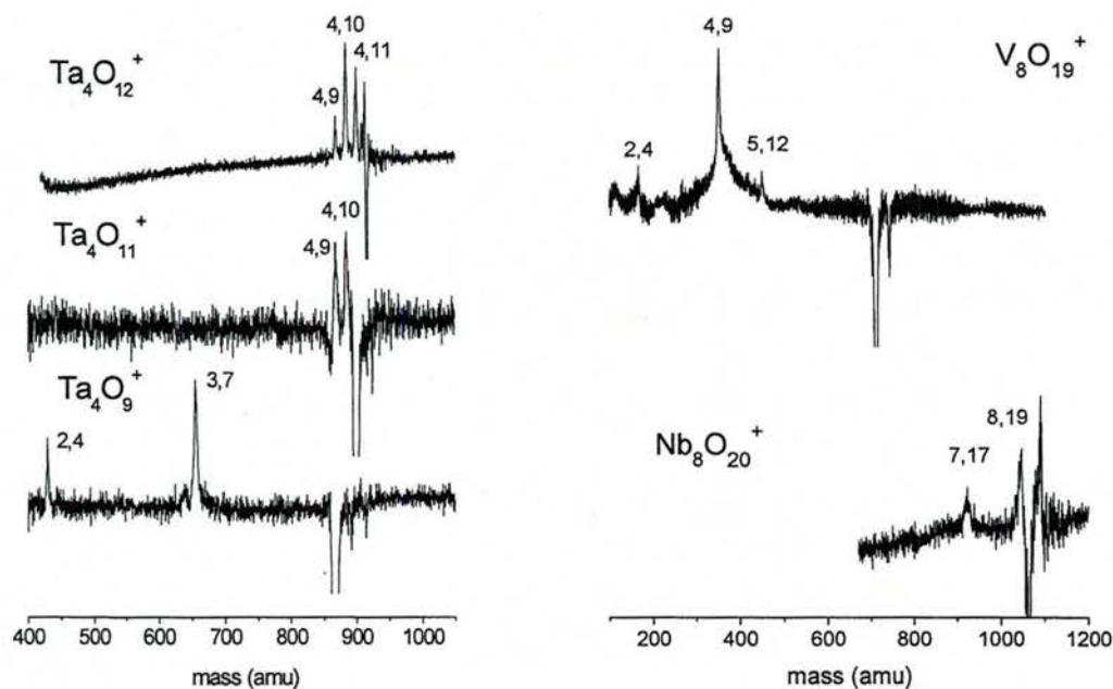
Figure 4. Photodissociation of Ta, V and Nb oxide clusters at 355 nm.
