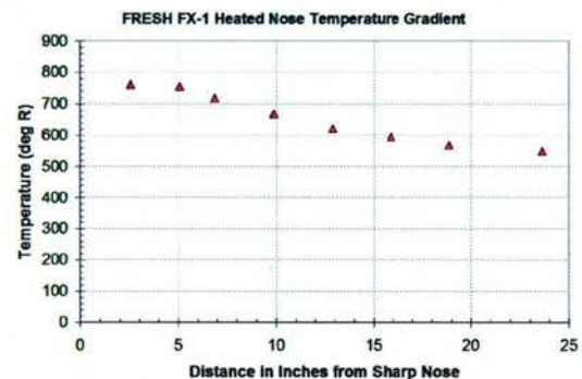
Figure 34. Pre-run Wall Temperature Gradient as Measured Thin-film Sensors
