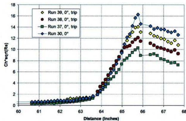
Figure 50. Tripped Mach 7.2 Forebody Flare Region Heat Flux Results for a Range of Reynolds Numbers
