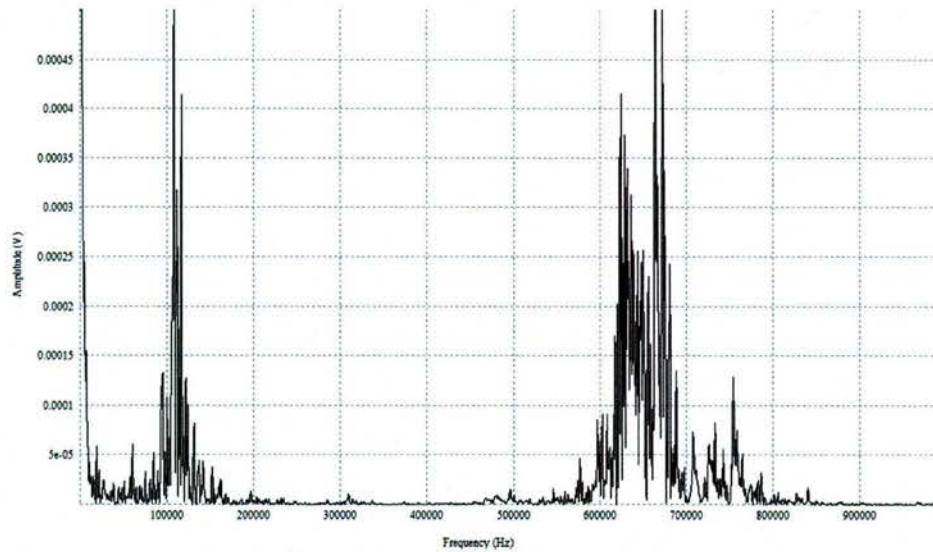
Figure 56. Frequencies Measured with Surface Time of Arrival Pressure Instrumentation at Flight Conditions
