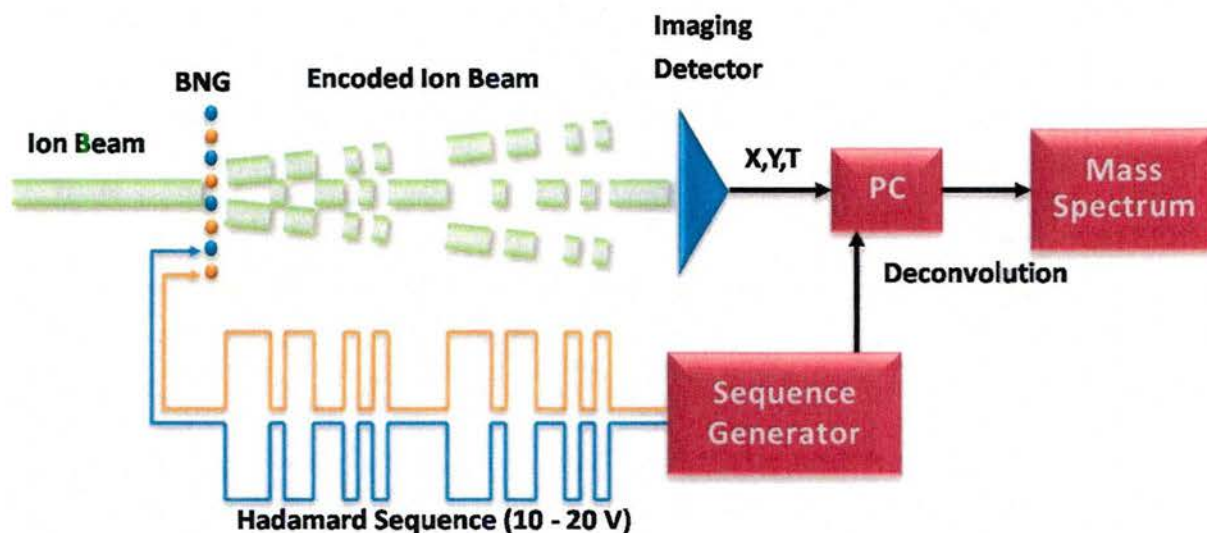
Figure 1: Schematic of the HT-TOFMS experiment.
