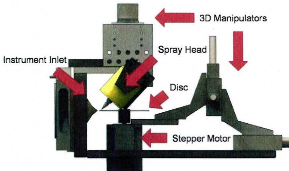
Figure 8: Disk platform for rapid DESI analysis.
