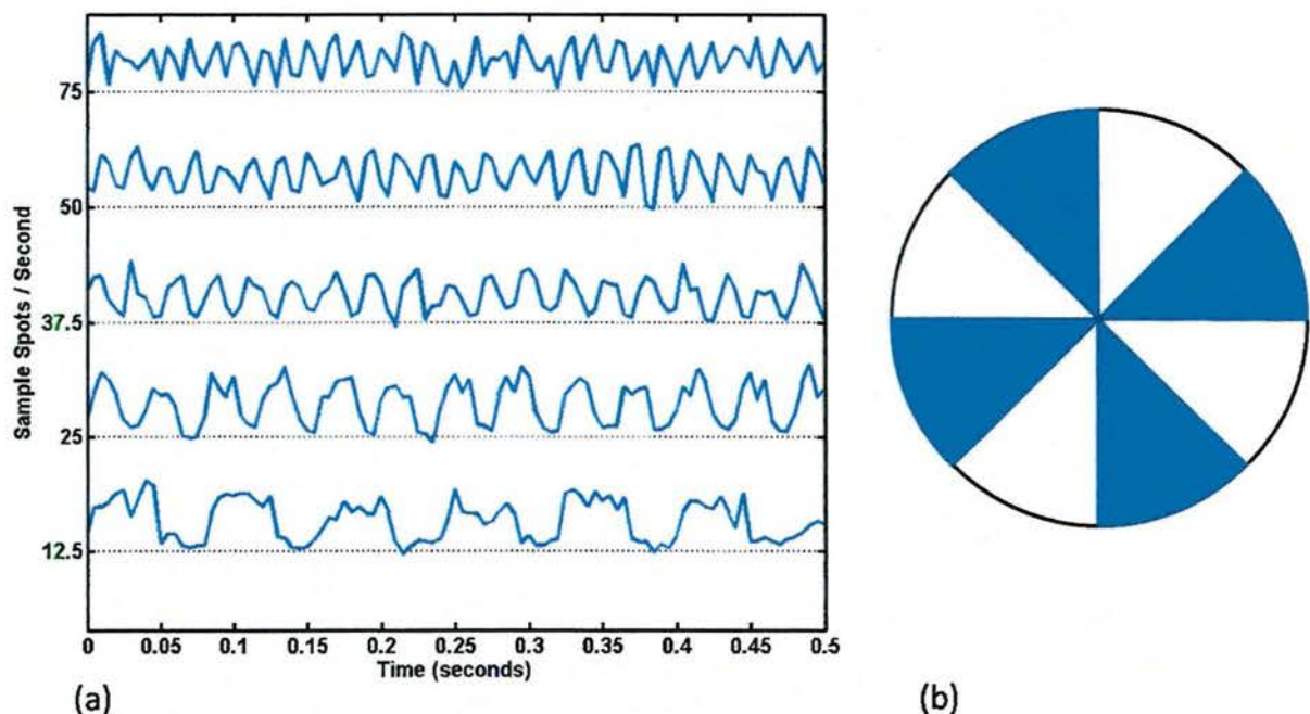
Figure 9: (a) Ion intensity of the basic blue 7 peak plotted vs time for various sampling rates and (b) cartoon of the analyzed disk surface with black sectors representing analyte-painted region.
