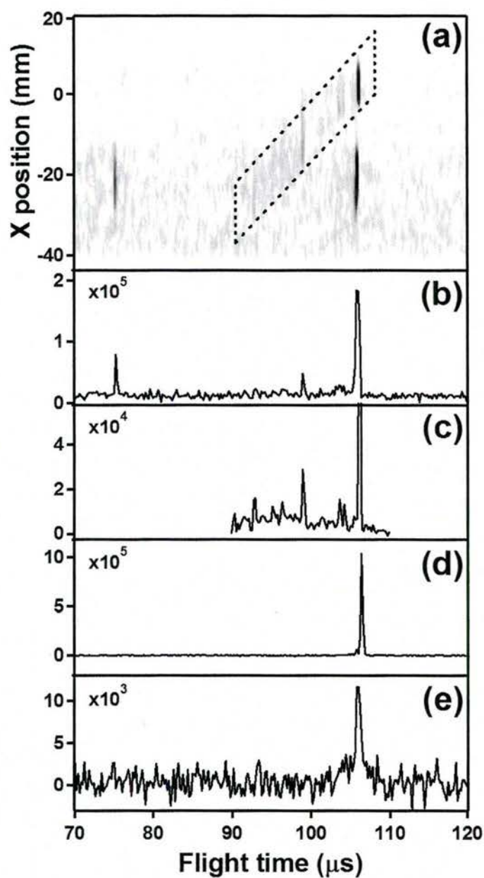
Figure 7: Mass spectra for data presented in Figure 6. (a) 2D plot of x position and flight time with the detector grid at 0 V in which the PSD fragment ions lie within the dotted box and (b–e) flight time spectra obtained (b) by summing over x positions, (c) by summing the dotted box region over x positions, (d) with detector grid at 1500 V, and (e) with detector grid at 2000 V.
