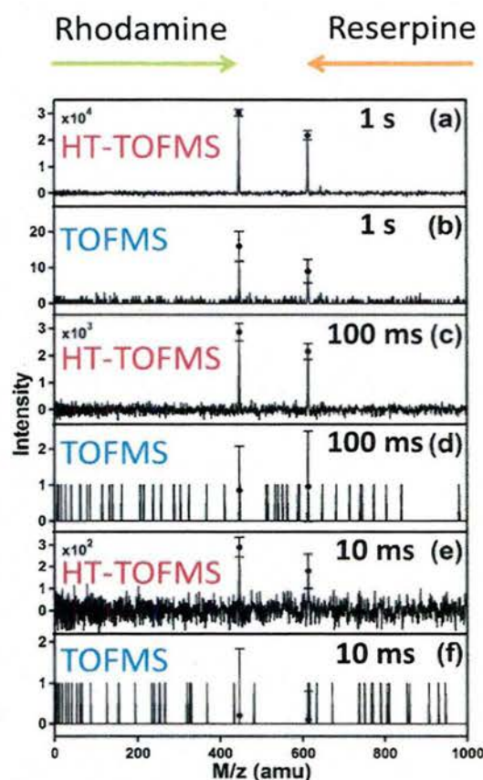
Figure 3: Peak height precision enhancement study of a mixture of rhodamine 6G (479 amu) and reserpine (609 amu) showing the spectral acquisition (a) of 1 s in Hadamard mode; (b) of 1 s in conventional mode; (c) of 100 ms in Hadamard mode; (d) of 100 ms in conventional mode; (e) of 10 ms in Hadamard mode; and (f) of 10 ms in conventional mode. The error bars are calculated from 16 experiments. Each plot is for one representative spectrum and dots represent the average peak heights.
