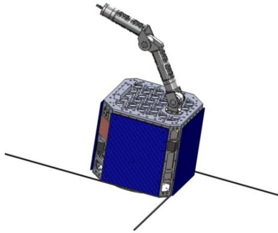
Figure 7. DYMAFLEX with Deployed Antennas. Source: [19].
