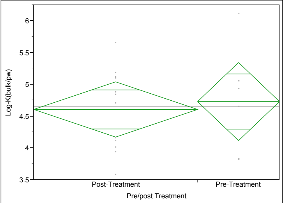
Oneway Analysis of Log-K(bulk/pw) By Pre/post Treatment
