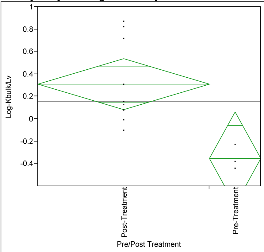
Oneway Analysis of Log- K_{bulk/Lv} By Pre/Post Treatment
