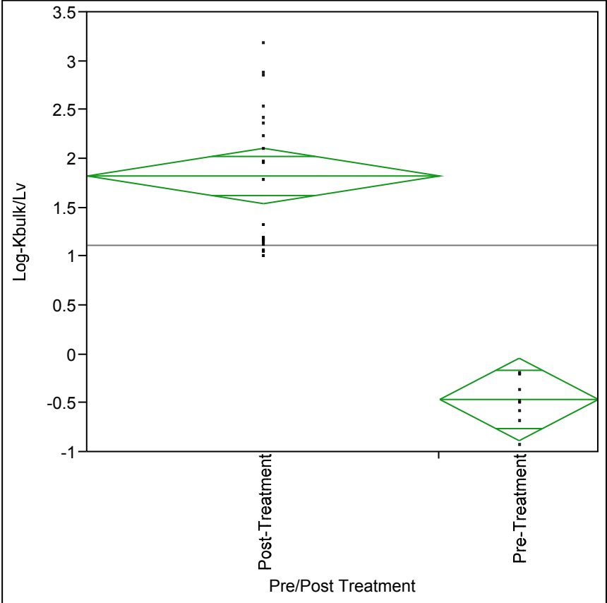
Oneway Analysis of Log- K_{bulk/Lv} By Pre/Post Treatment
