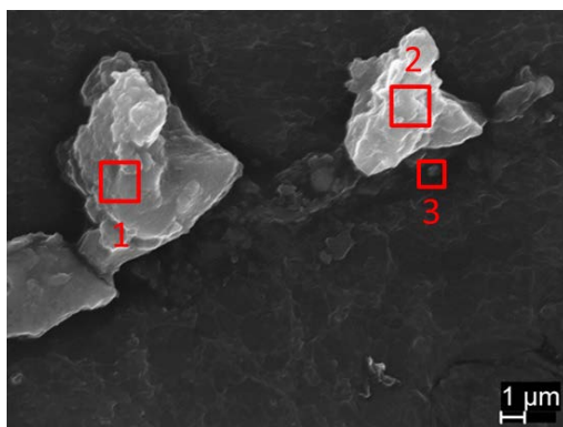
Figure 55. Secondary electron image of post-LDHP tektite particles analyzed showing significantly different chemical compositions. Red boxes indicate particles analyzed.
