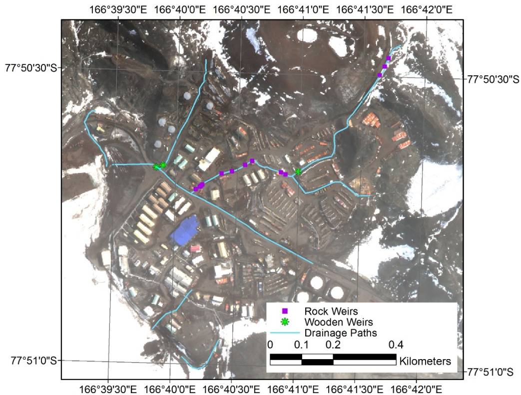
Figure 4. Actual locations where the wooden and the rock weirs were installed.
