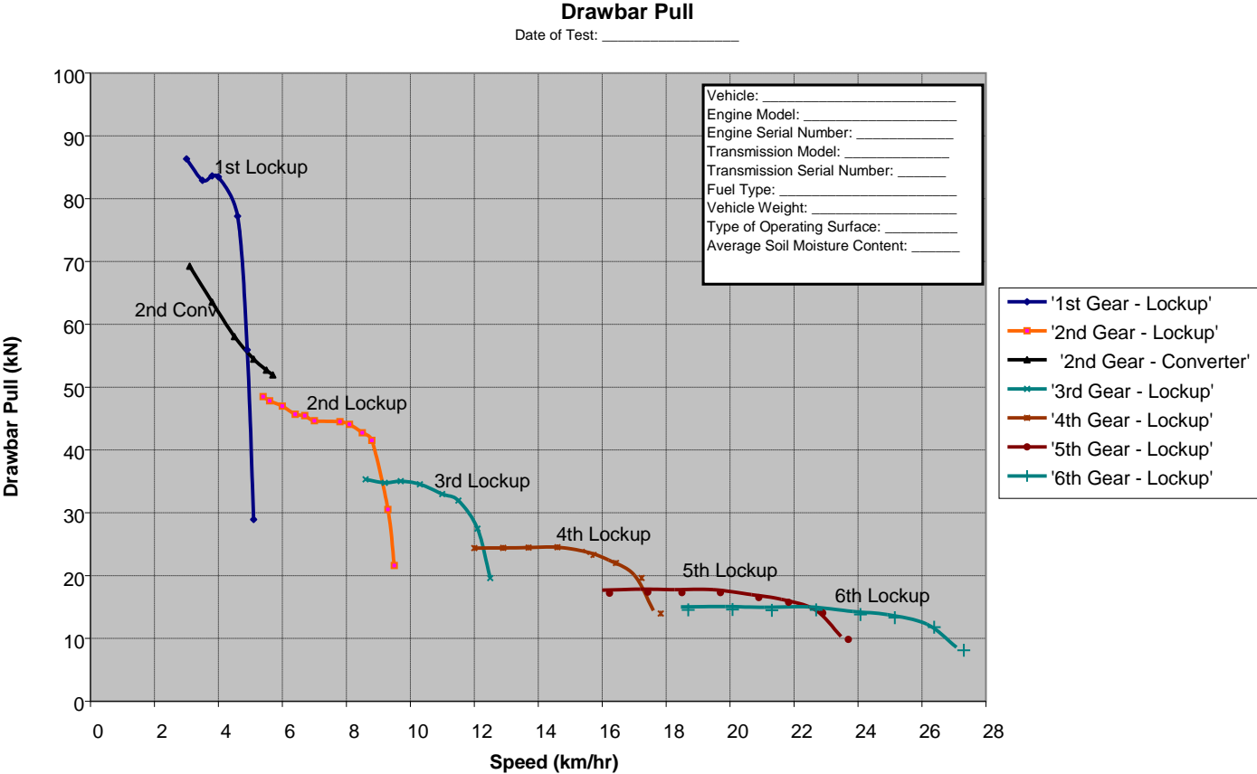
Figure 1. Drawbar pull characteristics.
