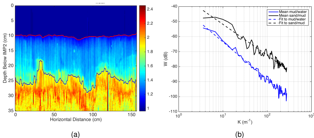
Figure 2: (a) Formation factor measured by the IMP2 conductivity probe in St. Andrew's Bay. The red and black lines indicate the mud/water interface and the sand/mud interface respectively. (b) The roughness power spectra corresponding to the surfaces indicated in (a).
