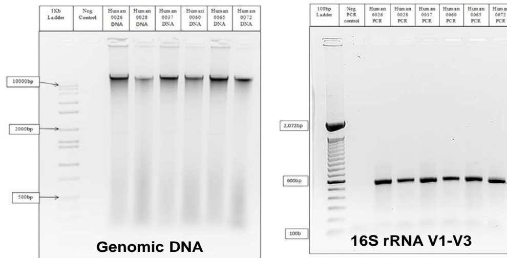
Figure 4. Gel electrophoresis of the genomic DNA and PCR amplification of bacteria from OpenBiome human donors
