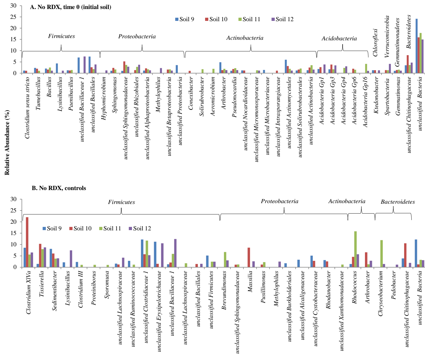
Figure 3.3. A comparison of the relative abundance (%) of the most common phylotypes (>1% , at the lowest classification level) in all four soils in the no RDX samples, including the initial soils (No RDX, time 0) (A) and the microcosms without RDX (No RDX controls) (B).
