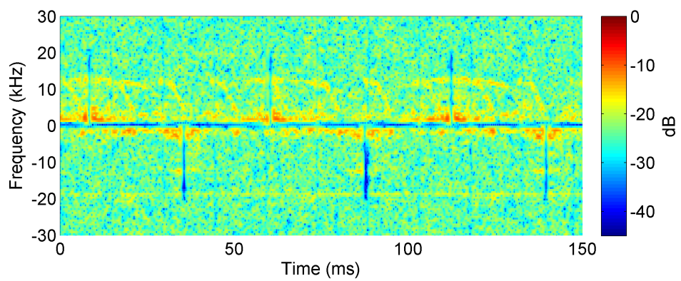
Figure 27: Stage 3 processing – for the tail rotor blades – on Squirrel helicopter data, at X-band, 180° aspect.
