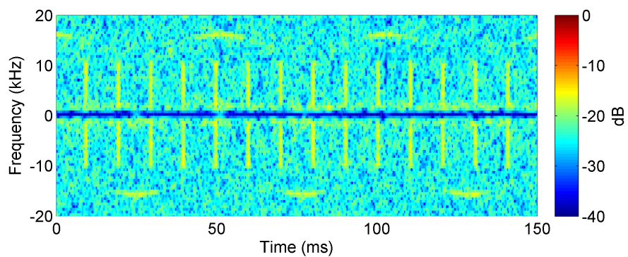
Figure 9: Simulated results in Stage 2 of the algorithm, for main rotor processing.
