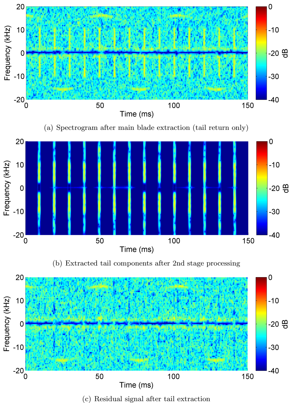
Figure 11: Simulated results in Stage 3 of the algorithm, for tail rotor processing.
