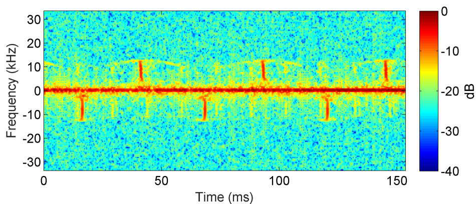
(b) Original data with additive clutter at SCR_{total} = 10 dB
