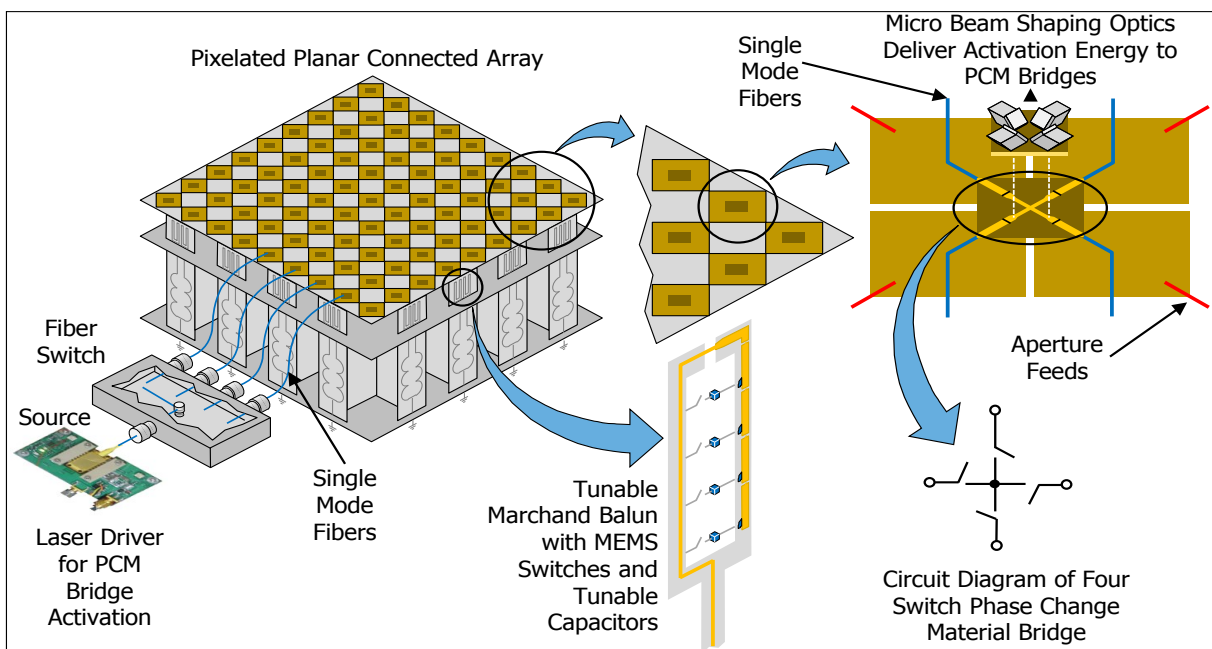
Figure 1. Block diagram of integrated optically-controlled pixelated connected array
