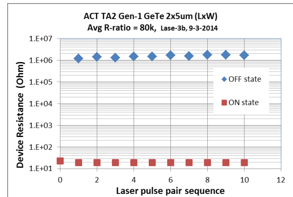
Figure 8. Repeatabile Toggle Between ON and OFF
