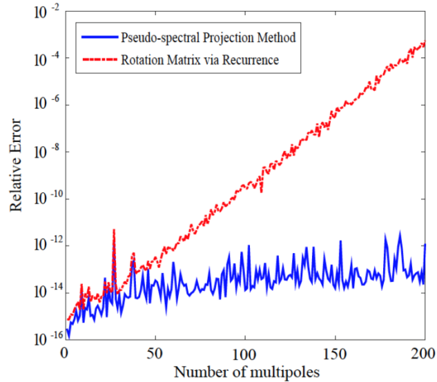
Figure 5. Relative error analysis of the coordinate rotation and pseudospectral projection rotation.
