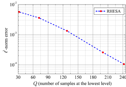
Figure 9. Accuracy test for far scattered fields of a dielectric sphere illuminated by a plane wave.
