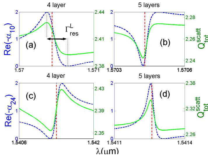
Fig. 7. Scattering resonances of the TE_{10} and TE_{24} modes (with N_{\text{clad}} = 4 and 5). The dashed lines represent the resonant scattering coefficient -\text{Re}(\alpha_i) (whose values are shown on the left y-axis), and the solid lines represent the total scattering efficiency Q_{\text{tot}}^{\text{scatt}} (whose values are shown on the right y-axis). The dashed vertical lines give the position of modal wavelength.
