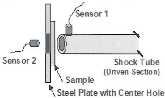
Figure 1: Experimental test setup showing the relative locations of the 79 mm diameter shock tube, sample and pressure sensors.
