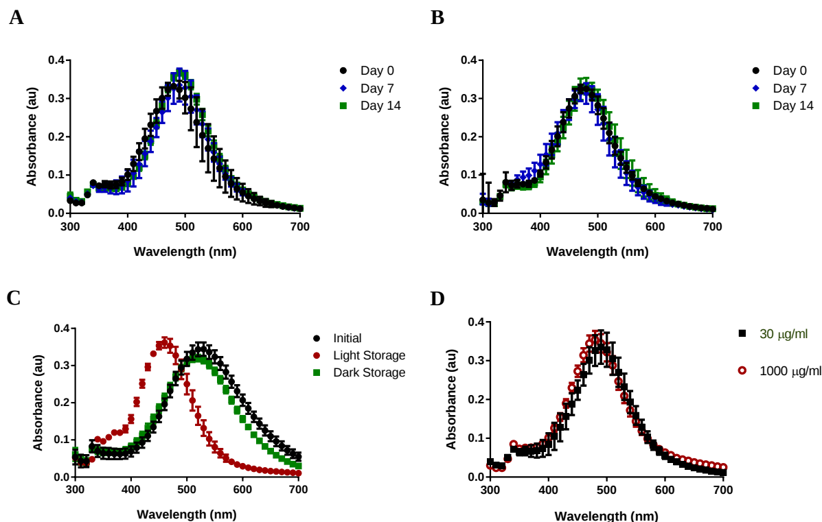
Figure 5: Silver nanoparticles stored in water for 14 days. A) Silver nanoparticle UV/vis spectra remained at 480 \pm 10 nm during storage at 4°C. B) Silver nanoparticle UV/vis spectra remained at 480 \pm 10 nm during storage at room temperature protected from light. C) This batch of AgNPs had an initial UV/vis spectra centered at 540 nm, which underwent a small shift to 520 nm when stored at room temperature protected from light but underwent a larger shift to 460 nm when stored at room temperature exposed to ambient light. D) Silver nanoparticle UV/vis spectra were equivalent for AgNPs stored at 4°C at concentrations of 30 µg/ml and 1000 µg/ml. All samples were analyzed at a concentration of 30 µg/ml.
