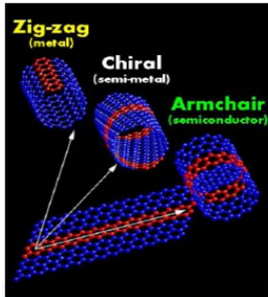
Figure 3: Three Forms of Carbon Nanotubes Based on Chirality 21
