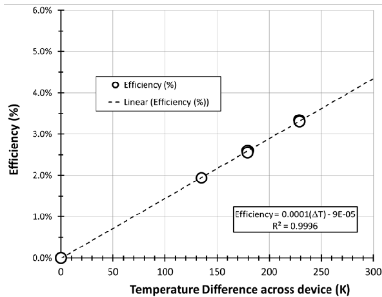
Fig. 3 Slope efficiency to determine ZT_{\text{max}} . T_{\text{cold}} = 343 \text{ K} and T_{\text{hot}} \text{ limit} = 873 \text{ K}
