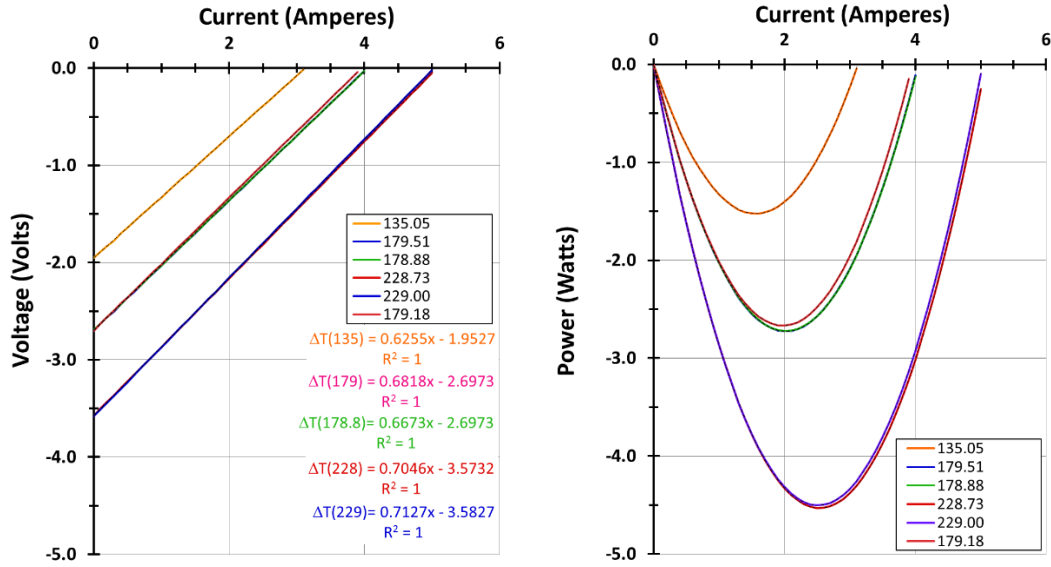
Fig. 2 Current-voltage load lines (left) and current-power curves (right) obtained with T_{\text{cold}} = 70 \text{ }^{\circ}\text{C} . The highest T_{\text{hot}} = 300 \text{ }^{\circ}\text{C} for which \Delta T = 229 \text{ }^{\circ}\text{C} .
