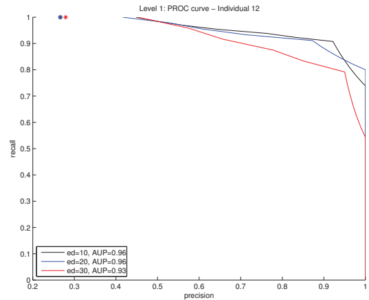
Fig. 3: PROC curve.
